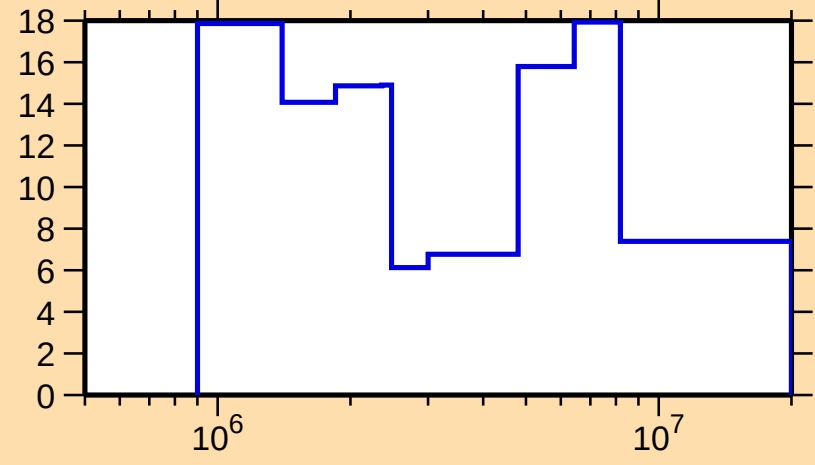
\Delta\sigma/\sigma vs. E for ^{261}\text{Lw}(n,\text{el.})
