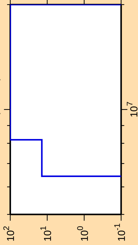
\Delta\sigma/\sigma vs. E for ^{261}\text{Lw}(n,2n\alpha)
