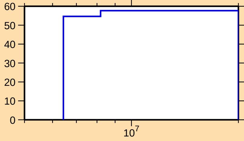
\Delta\sigma/\sigma vs. E for ^{261}\text{Lw}(n,\text{inel.})
