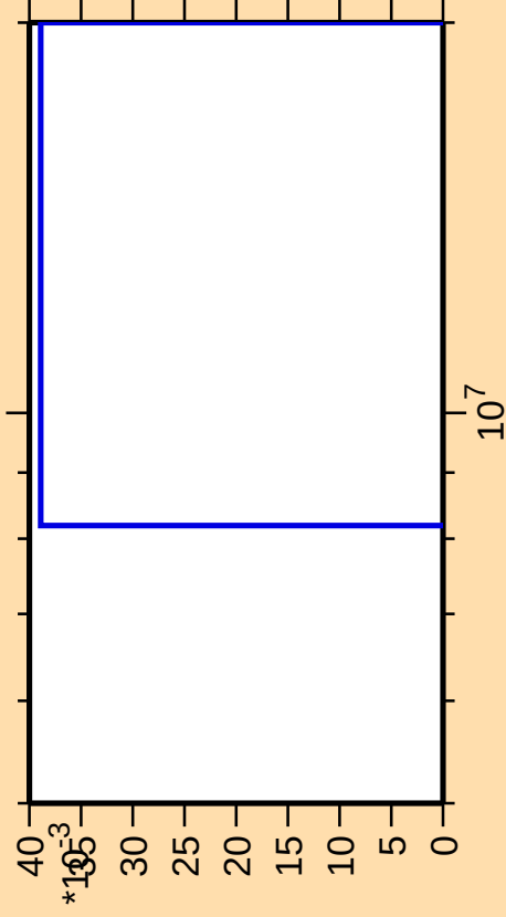
\Delta\sigma/\sigma vs. E for ^{261}\text{Lw(mt 42)}
