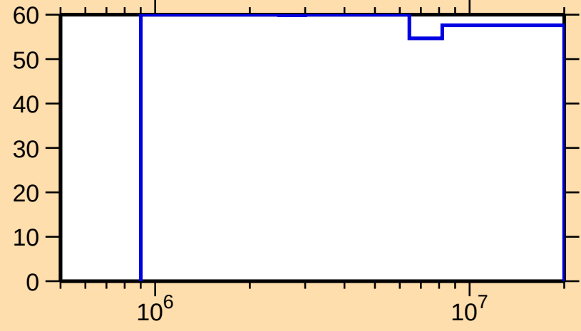
\Delta\sigma/\sigma vs. E for ^{261}\text{Lw}(n,n\text{cont.})
