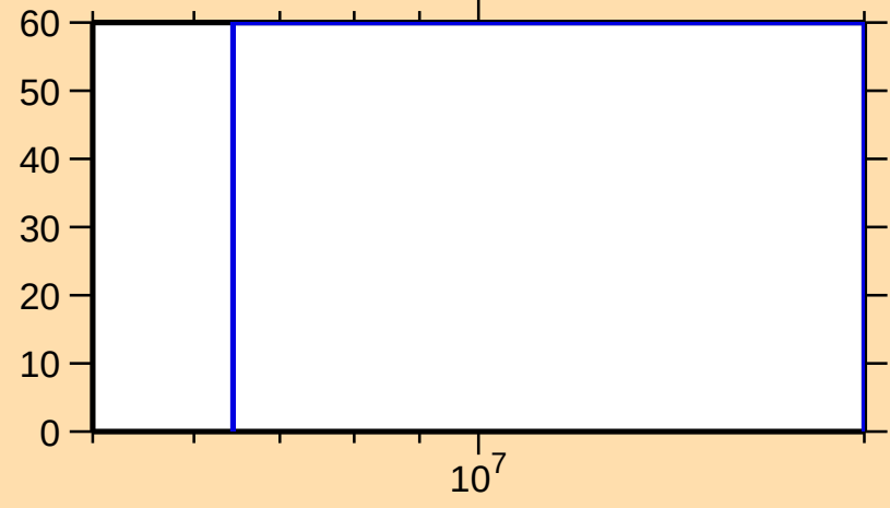
\Delta\sigma/\sigma vs. E for ^{261}\text{Lw}(n,2n)
