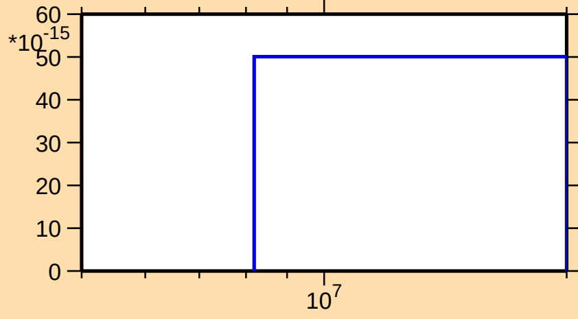
\sigma vs. E for ^{261}\text{Lw(mt 11)}
