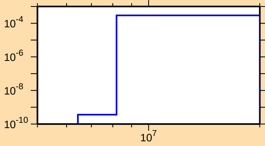
\sigma vs. E for ^{261}\text{Lw}(n,d)
