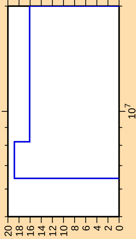
\Delta\sigma/\sigma vs. E for ^{261}\text{Lw}(n,f)
