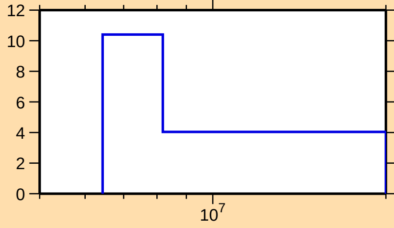
\Delta\sigma/\sigma vs. E for ^{261}\text{Lw}(n,\text{tot.})
