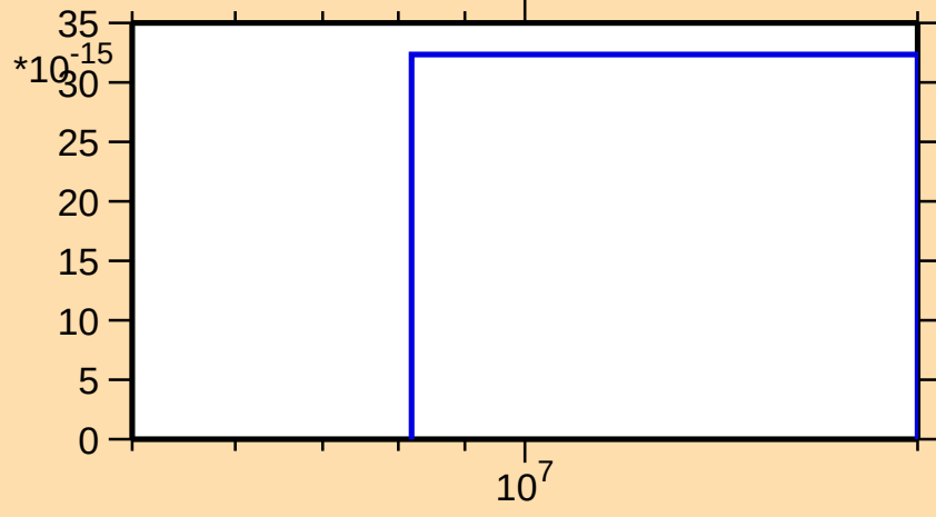
\sigma vs. E for ^{261}\text{Lw(mt 45)}
