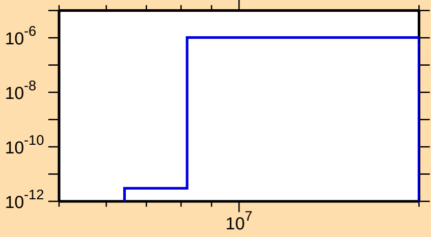
\sigma vs. E for ^{261}\text{Lw}(n,2n\alpha)
