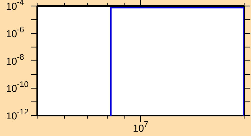
\sigma vs. E for ^{261}\text{Lw}(n,t)
