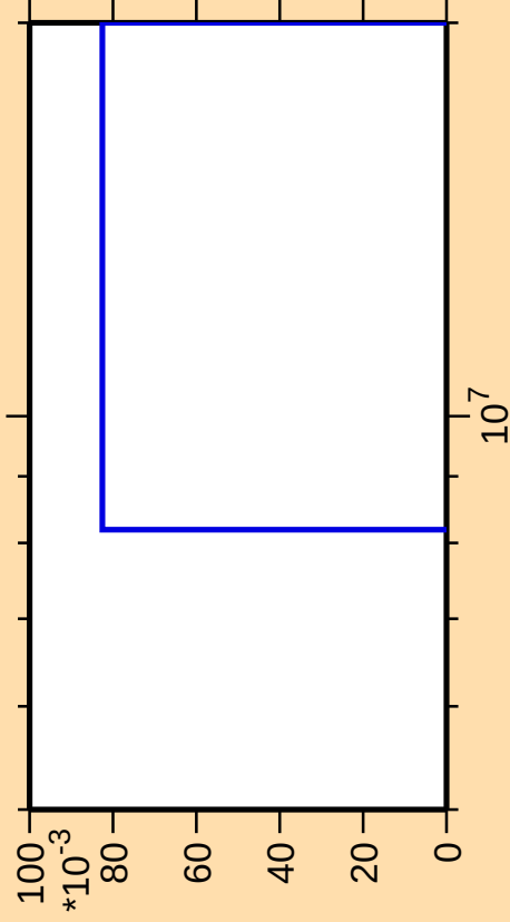
\Delta\sigma/\sigma vs. E for ^{261}\text{Lw(mt 11)}
