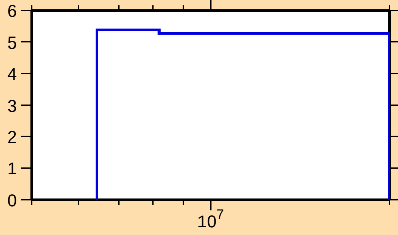
\Delta\sigma/\sigma vs. E for ^{261}\text{Lw}(n,\text{nonel.})
