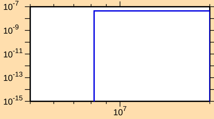
\sigma vs. E for ^{261}\text{Lw}(n,nd)
