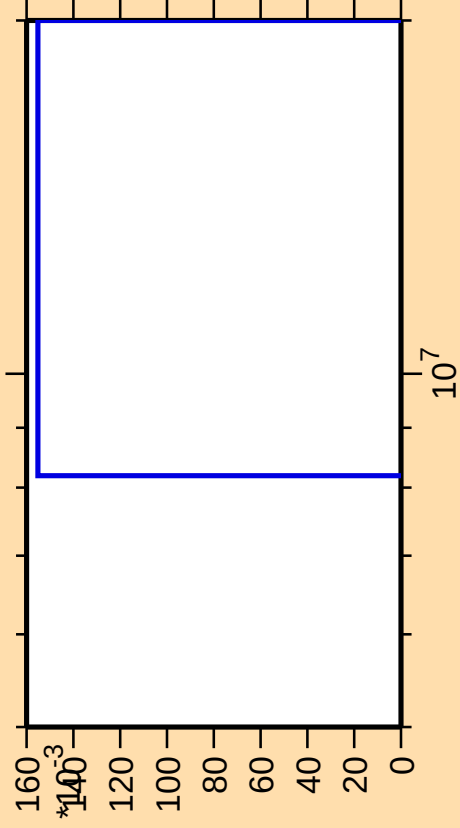
\Delta\sigma/\sigma vs. E for ^{261}\text{Lw(mt 45)}
