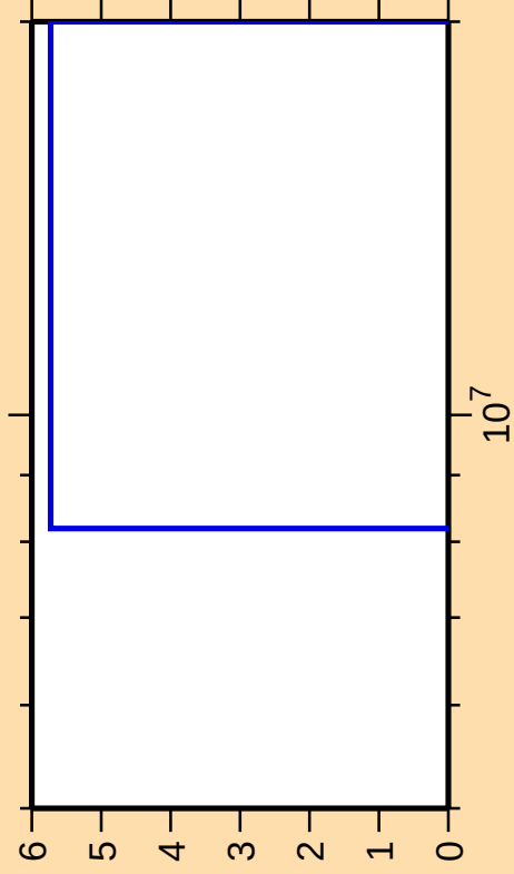
\Delta\sigma/\sigma vs. E for ^{261}\text{Lw}(n,p\alpha)
