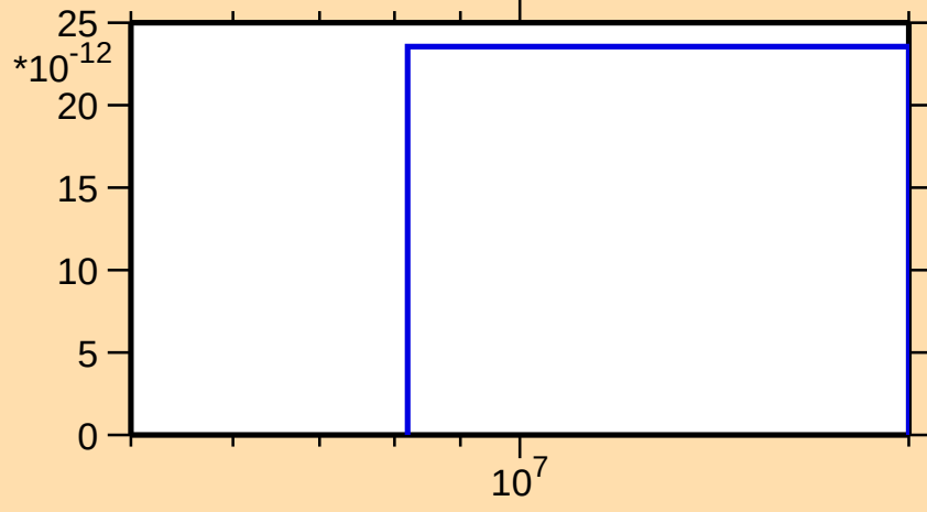
\sigma vs. E for ^{261}\text{Lw}(n,\text{He3})
