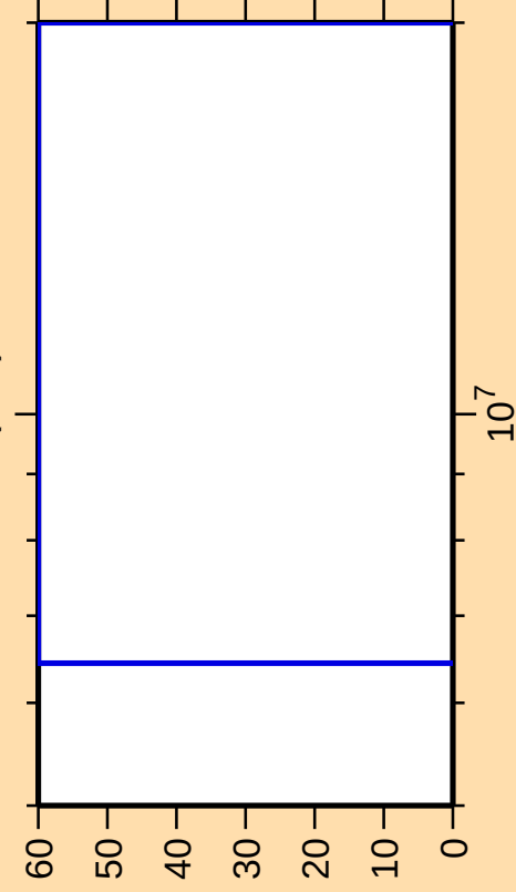
\Delta\sigma/\sigma vs. E for ^{261}\text{Lw}(n,d)
