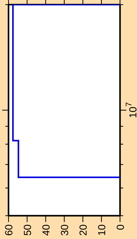
\Delta\sigma/\sigma vs. E for ^{261}\text{Lw}(n,n\text{cont.})
