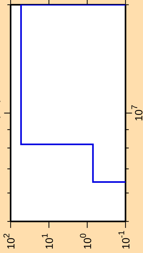
\Delta\sigma/\sigma vs. E for ^{261}\text{Lw}(n,t)
