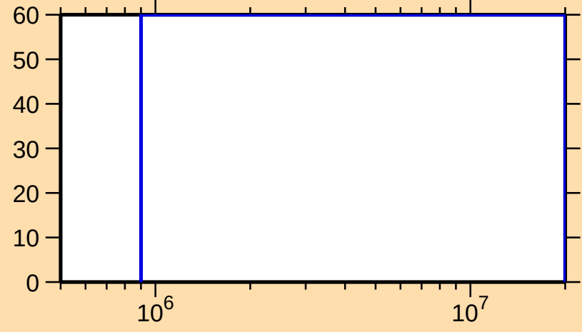
\Delta\sigma/\sigma vs. E for ^{261}\text{Lw}(n,n_1)
