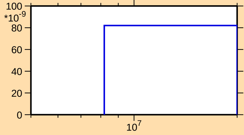
\sigma vs. E for ^{261}\text{Lw}(n,3n\alpha)
