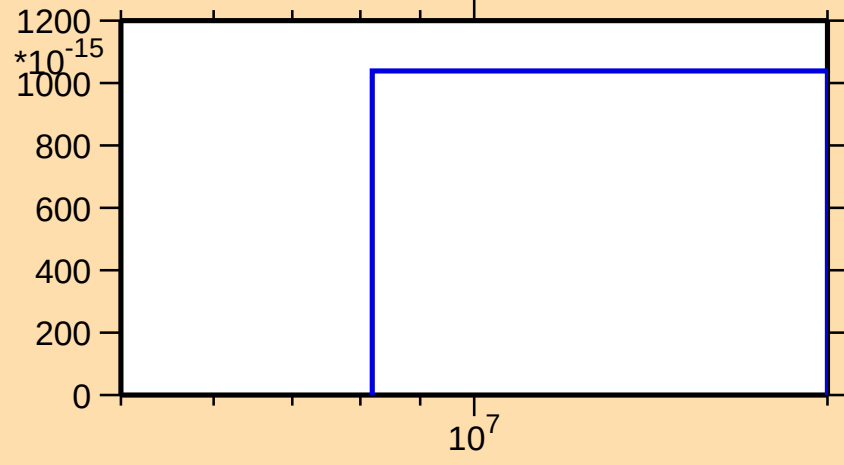
\sigma vs. E for ^{261}\text{Lw}(n,p\alpha)
