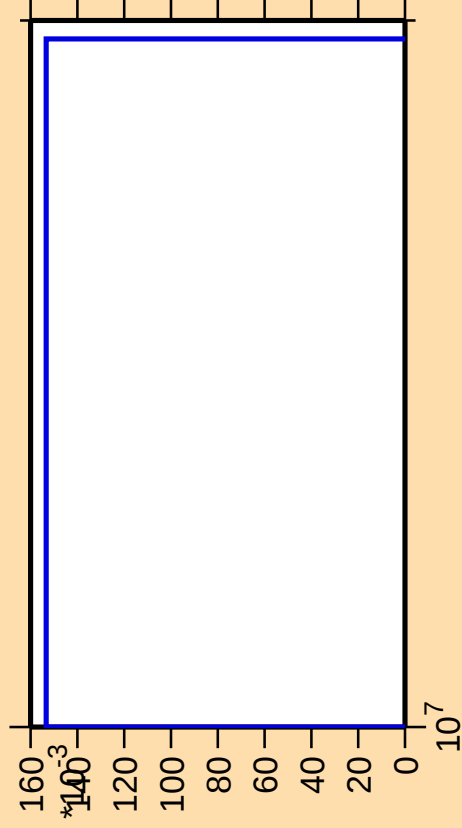
\Delta\sigma/\sigma vs. E for ^{262}\text{Lw(mt 11)}
