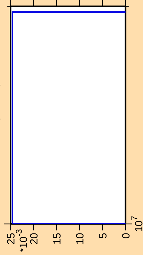
\Delta\sigma/\sigma vs. E for ^{262}\text{Lw}(\text{mt } 42)
