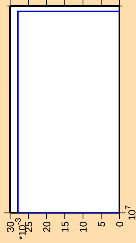
\Delta\sigma/\sigma vs. E for ^{262}\text{Lw}(\text{mt } 34)
