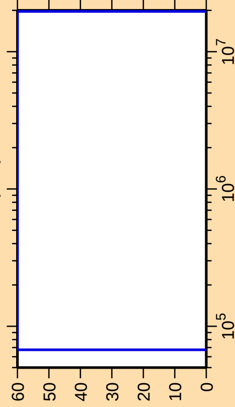
\Delta\sigma/\sigma vs. E for ^{262}\text{Lw}(n,\alpha)
