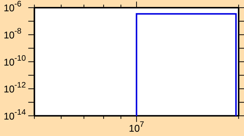
\sigma vs. E for ^{262}\text{Lw}(n,nd)
