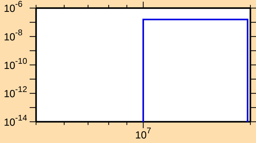
\sigma vs. E for ^{262}\text{Lw}(n,nt)
