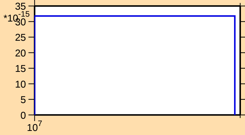
\sigma vs. E for ^{262}\text{Lw(mt 11)}
