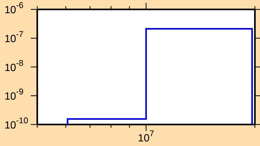
\sigma vs. E for ^{262}\text{Lw}(n,2n\alpha)
