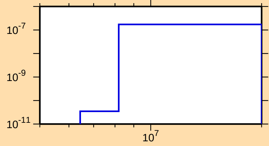
\sigma vs. E for ^{262}\text{Lw}(n,2n\alpha)
