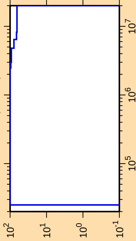
\Delta\sigma/\sigma vs. E for ^{262}\text{Lw}(n,\text{inel.})
