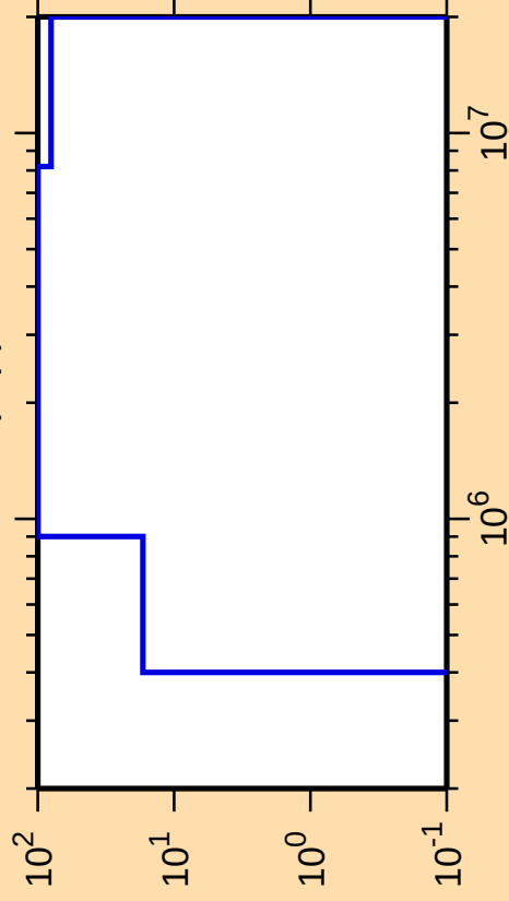
\Delta\sigma/\sigma vs. E for ^{262}\text{Lw}(n,p)
