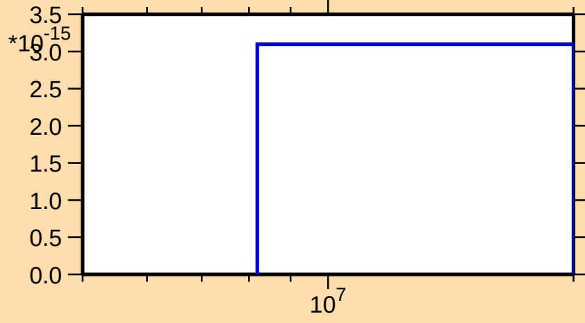
\sigma vs. E for ^{262}\text{Lw}(\text{mt } 34)
