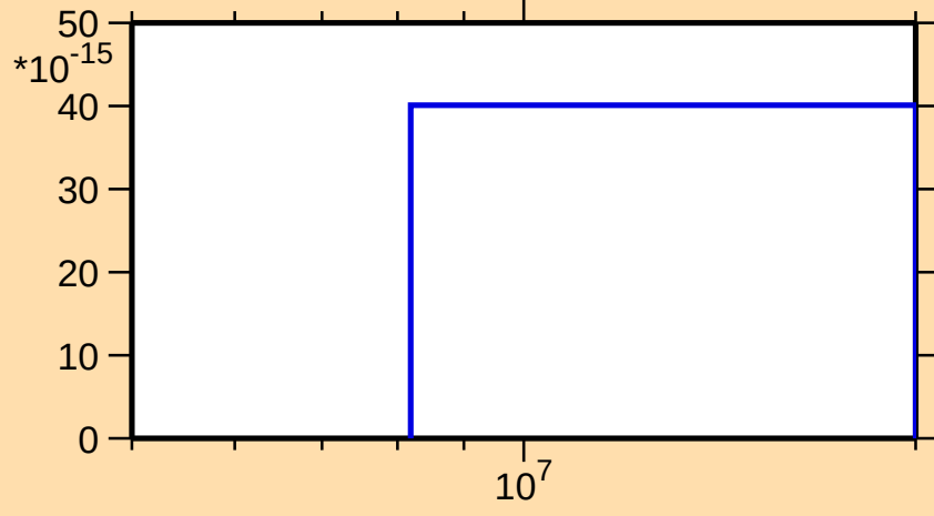
\sigma vs. E for ^{262}\text{Lw}(\text{mt 11})
