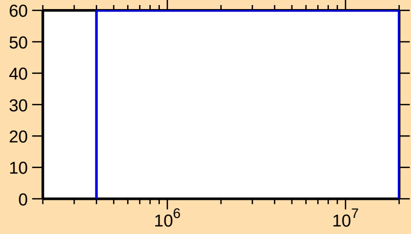
\Delta\sigma/\sigma vs. E for ^{262}\text{Lw}(n,n\text{cont.})
