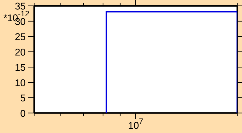
\sigma vs. E for ^{262}\text{Lw}(n,\text{He3})
