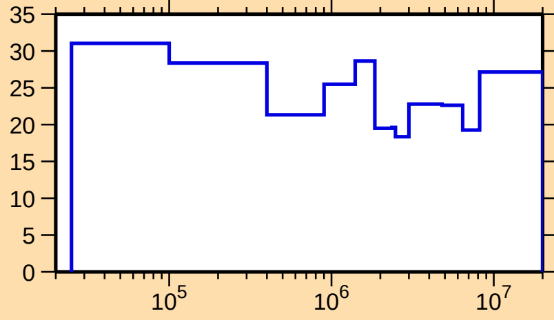
\Delta\sigma/\sigma vs. E for ^{262}\text{Lw}(n,\text{el.})
