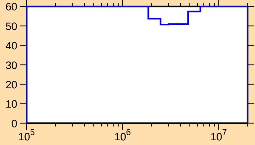
\Delta\sigma/\sigma vs. E for ^{262}\text{Lw}(n,n_1)
