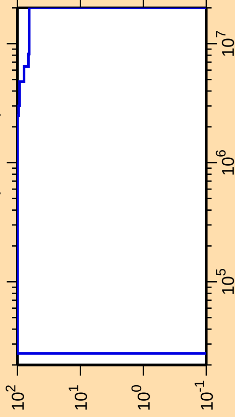
\Delta\sigma/\sigma vs. E for ^{262}\text{Lw}(n,\text{ncont.})
