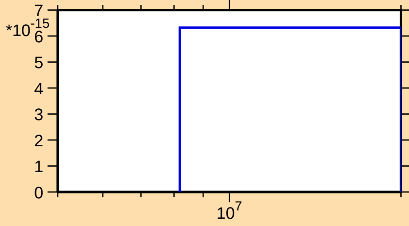
\sigma vs. E for ^{262}\text{Lw(mt 42)}
