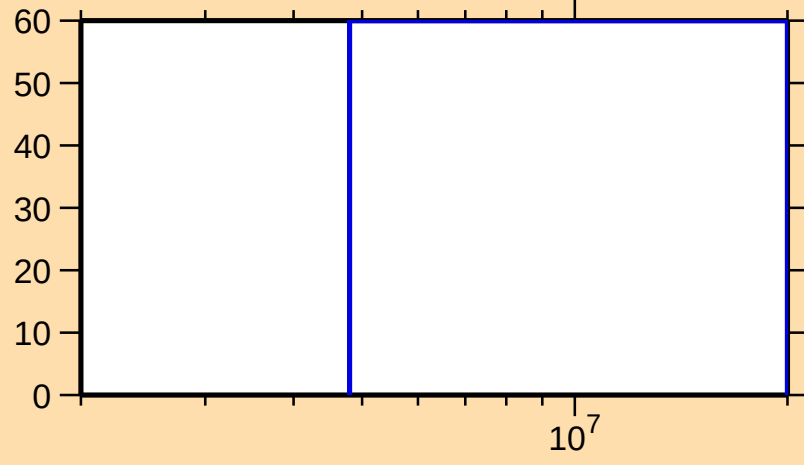
\Delta\sigma/\sigma vs. E for ^{262}\text{Lw}(n,2n)
