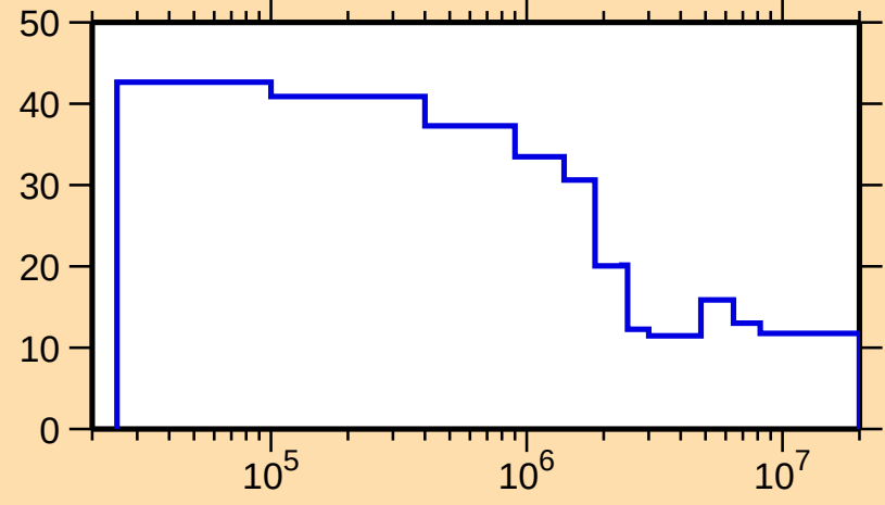
\Delta\sigma/\sigma vs. E for ^{262}\text{Lw}(n,n\text{onel.})
