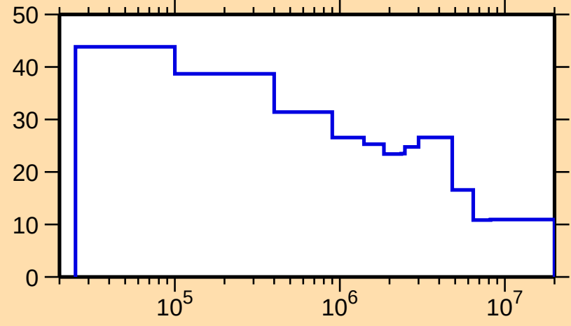
\Delta\sigma/\sigma vs. E for ^{262}\text{Lw}(n,f)
