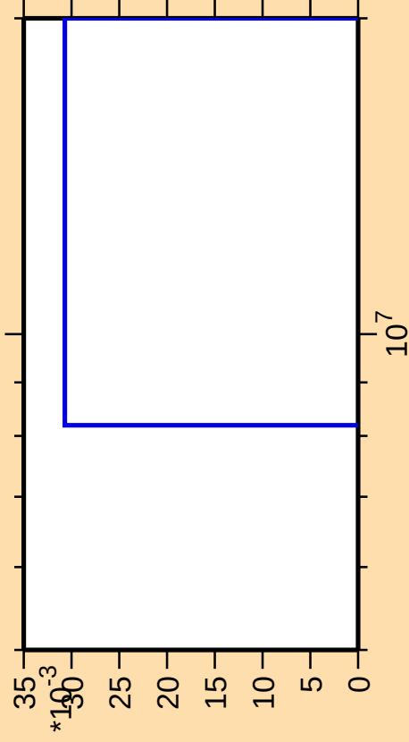
\Delta\sigma/\sigma vs. E for ^{262}\text{Lw(mt 42)}
