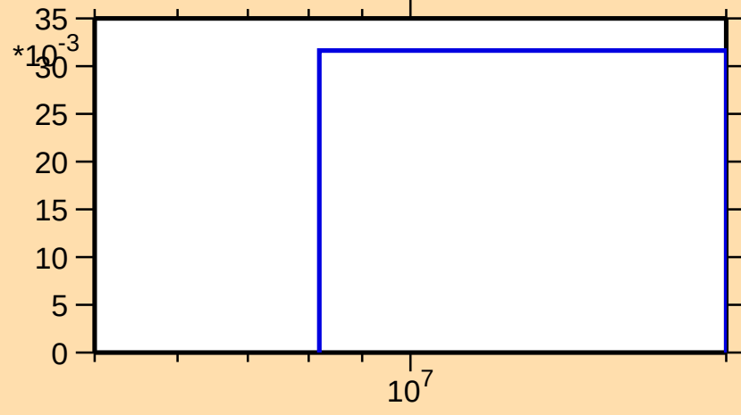
\sigma vs. E for ^{262}\text{Lw}(n,3n)
