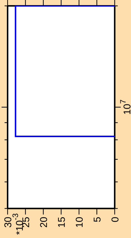
\Delta\sigma/\sigma vs. E for ^{262}\text{Lw}(\text{mt } 34)
