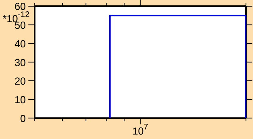
\sigma vs. E for ^{262}\text{Lw}(n,3n\alpha)
