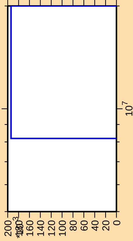
\Delta\sigma/\sigma vs. E for ^{262}\text{Lw}(\text{mt 11})
