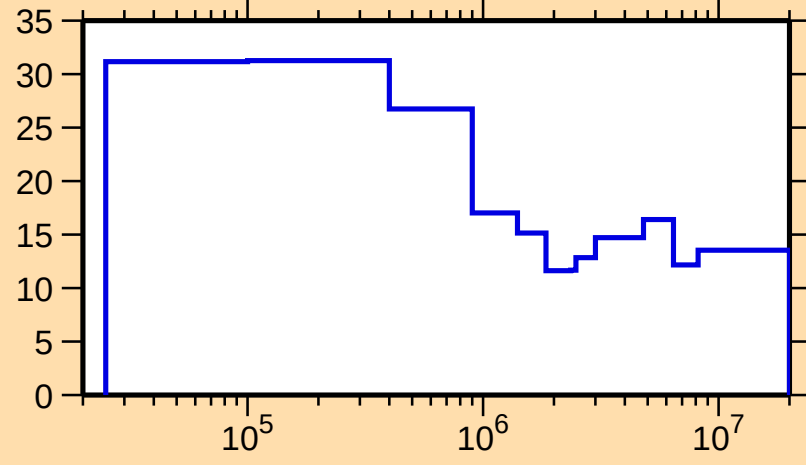
\Delta\sigma/\sigma vs. E for ^{262}\text{Lw}(n,\text{tot.})
