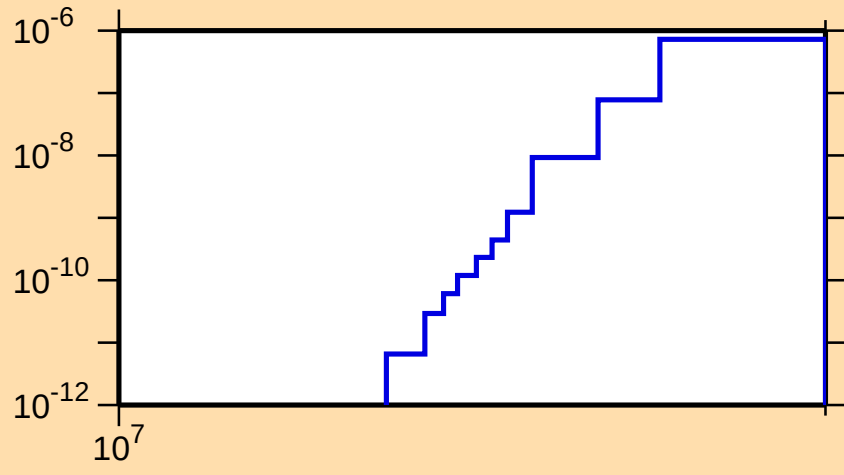
\sigma vs. E for ^{265}\text{Lw}(n,nt)
