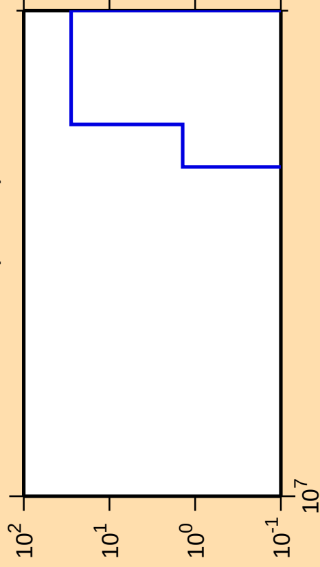
\Delta\sigma/\sigma vs. E for ^{265}\text{Lw}(n,\text{He3})
