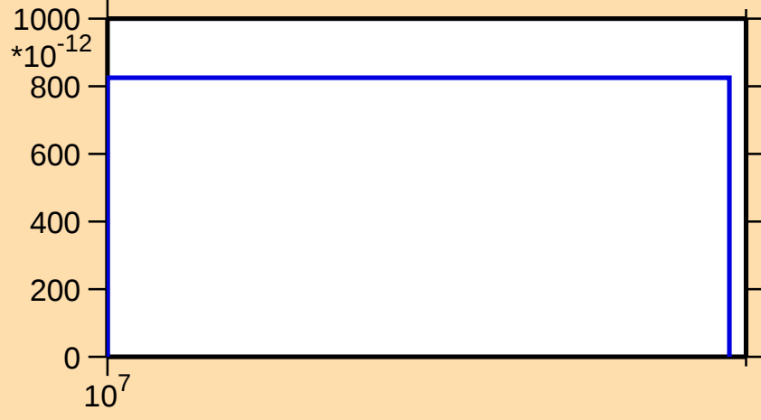
\sigma vs. E for ^{265}\text{Lw}(n,nd)
