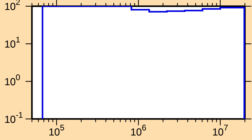
\Delta\sigma/\sigma vs. E for ^{265}\text{Lw}(n,\text{inel.})
