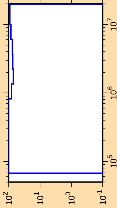
\Delta\sigma/\sigma vs. E for ^{265}\text{Lw}(n,\text{inel.})
