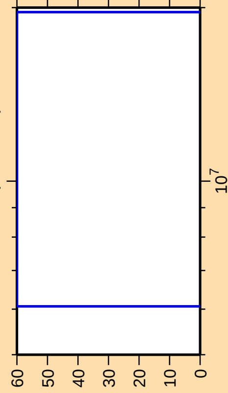
\Delta\sigma/\sigma vs. E for ^{265}\text{Lw}(n,n\text{cont.})
