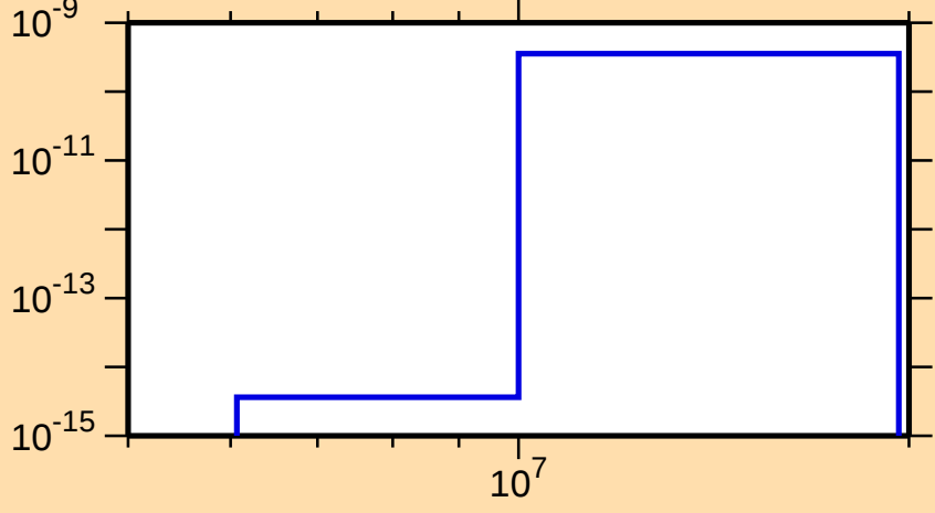
\sigma vs. E for ^{265}\text{Lw}(n,2n\alpha)
