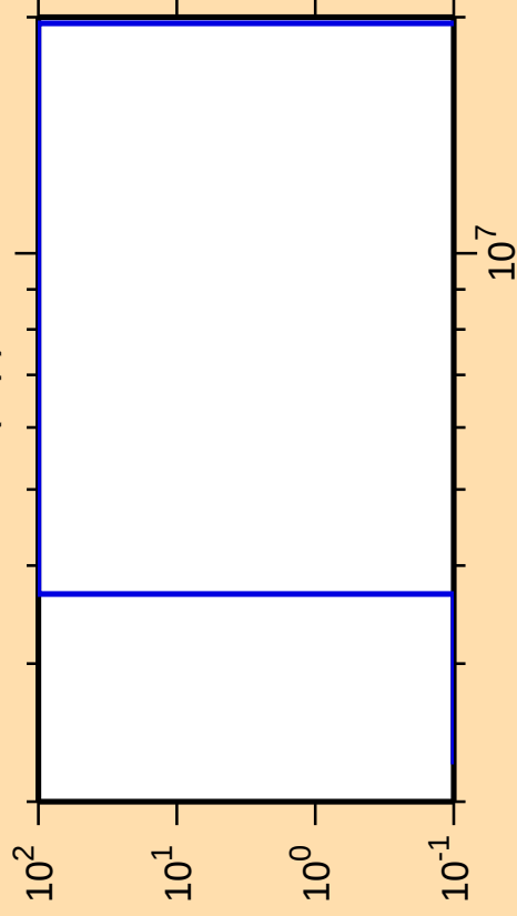
\Delta\sigma/\sigma vs. E for ^{265}\text{Lw}(n,p)
