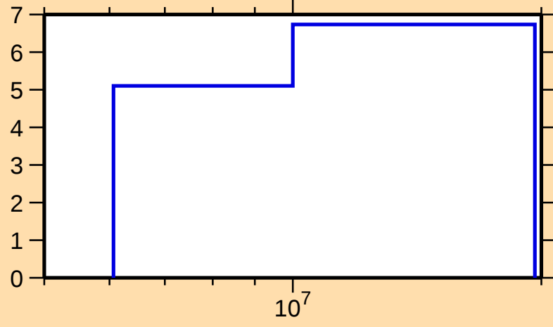
\Delta\sigma/\sigma vs. E for ^{265}\text{Lw}(n,\text{nonel.})
