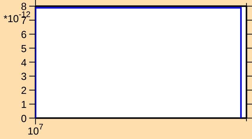
\sigma vs. E for ^{265}\text{Lw}(n,2np)
