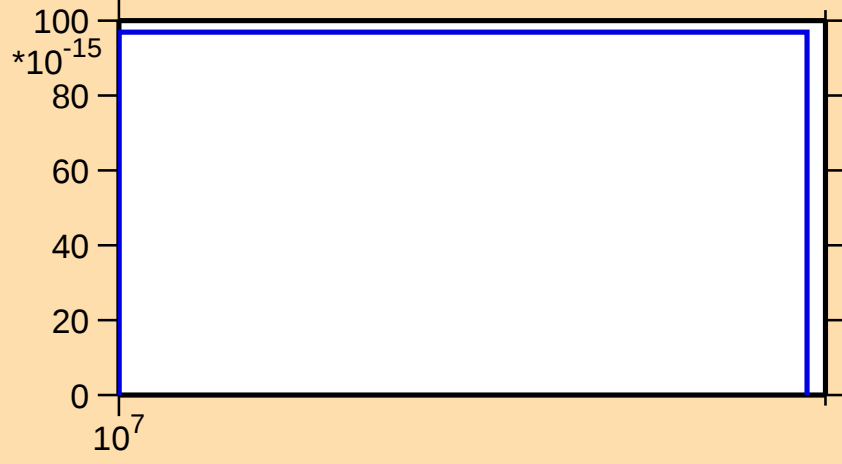
\sigma vs. E for ^{265}\text{Lw}(n,\text{He3})
