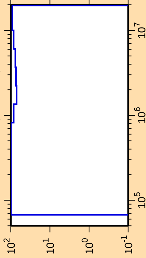
\Delta\sigma/\sigma vs. E for ^{265}\text{Lw}(n,\text{ncont.})
