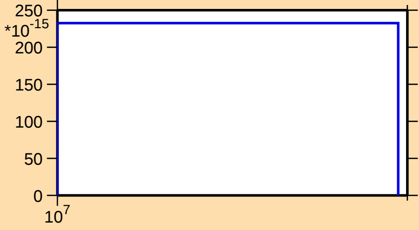
\sigma vs. E for ^{265}\text{Lw}(n,3n\alpha)
