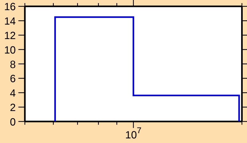
\Delta\sigma/\sigma vs. E for ^{265}\text{Lw}(n,\text{el.})
