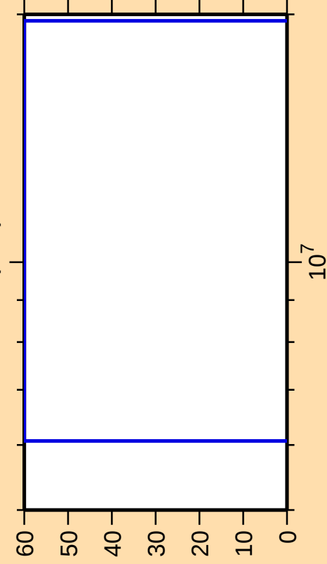
\Delta\sigma/\sigma vs. E for ^{265}\text{Lw}(n,\alpha)
