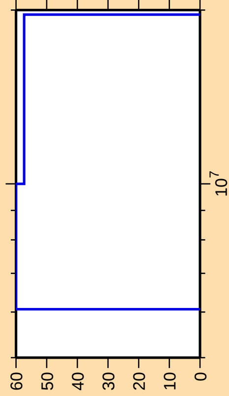
\Delta\sigma/\sigma vs. E for ^{265}\text{Lw}(n,2n)
