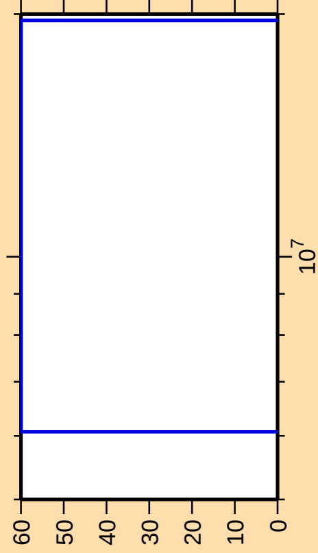
\Delta\sigma/\sigma vs. E for ^{265}\text{Lw}(n,\gamma)
