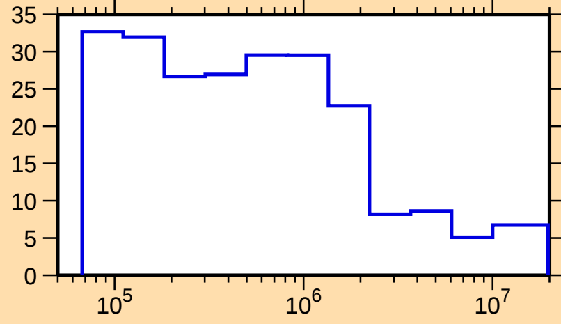
\Delta\sigma/\sigma vs. E for ^{265}\text{Lw}(n,\text{nonel.})
