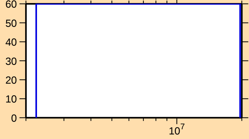
\Delta\sigma/\sigma vs. E for ^{265}\text{Lw}(n,n\text{cont.})
