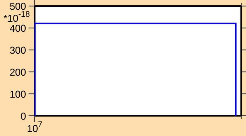
\sigma vs. E for ^{265}\text{Lw(mt 11)}
