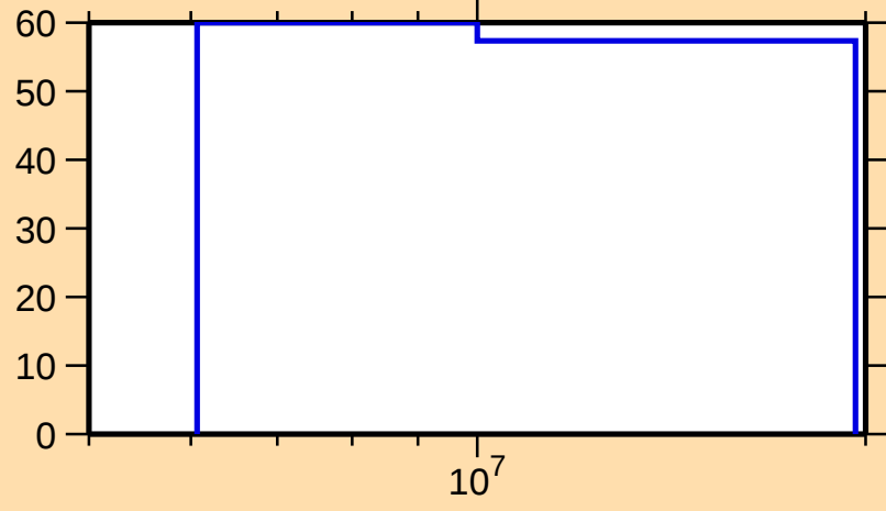
\Delta\sigma/\sigma vs. E for ^{265}\text{Lw}(n,2n)
