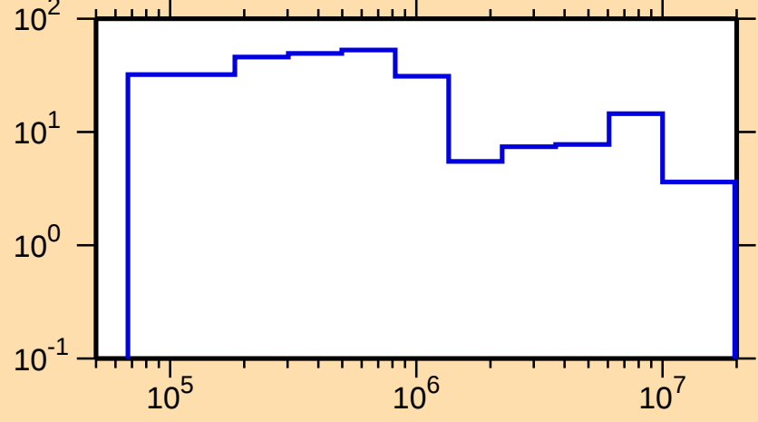
\Delta\sigma/\sigma vs. E for ^{265}\text{Lw}(n,\text{el.})
