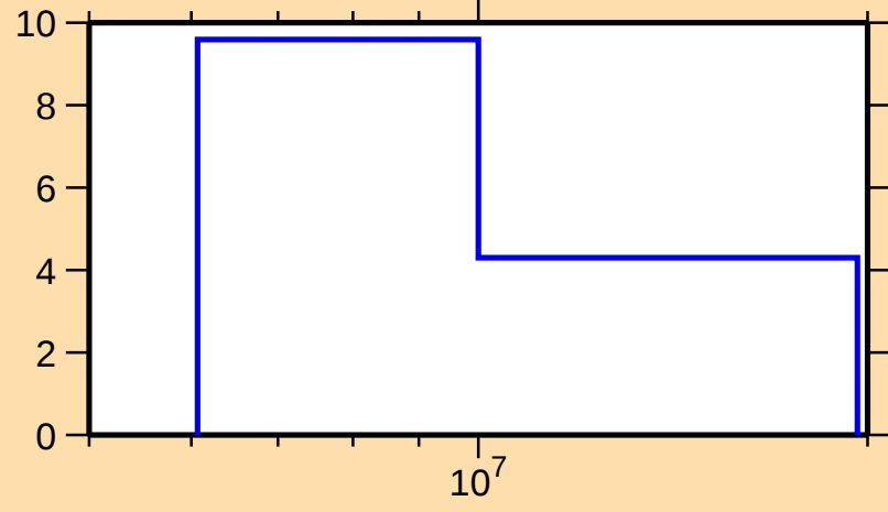
\Delta\sigma/\sigma vs. E for ^{265}\text{Lw}(n,\text{tot.})
