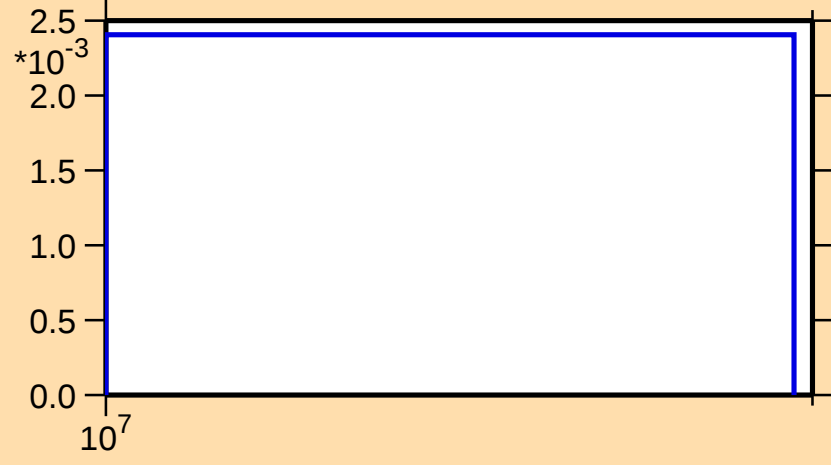
\sigma vs. E for ^{265}\text{Lw}(n,3n)
