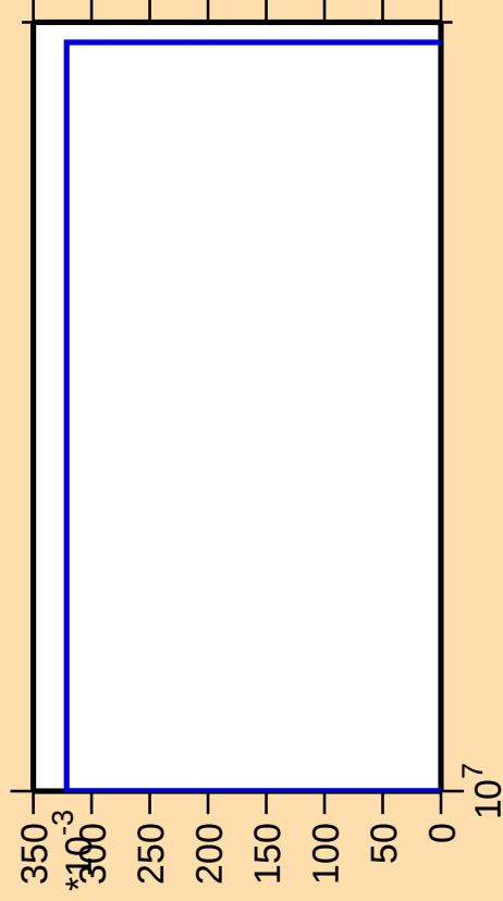
\Delta\sigma/\sigma vs. E for ^{265}\text{Lw}(n,\text{He3})
