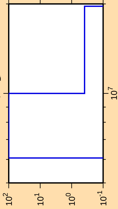
\Delta\sigma/\sigma vs. E for ^{265}\text{Lw}(n,n_1)
