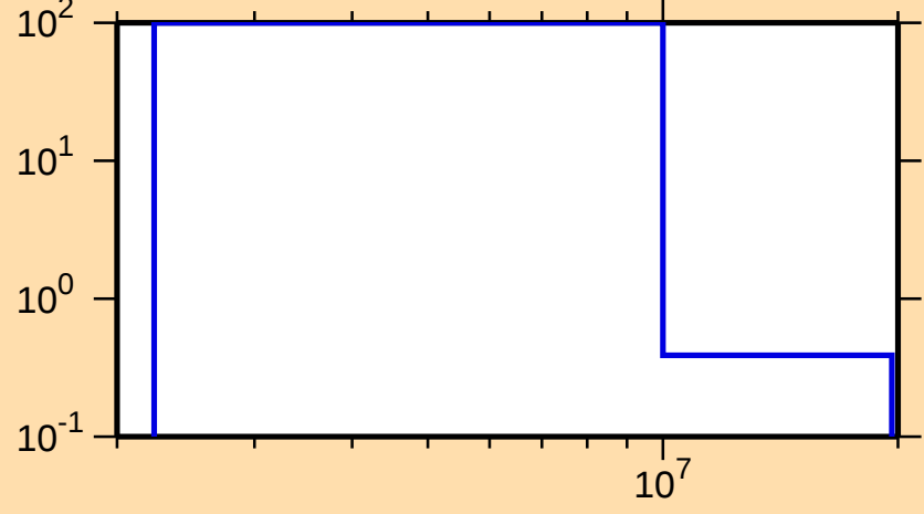
\Delta\sigma/\sigma vs. E for ^{265}\text{Lw}(n,n_1)
