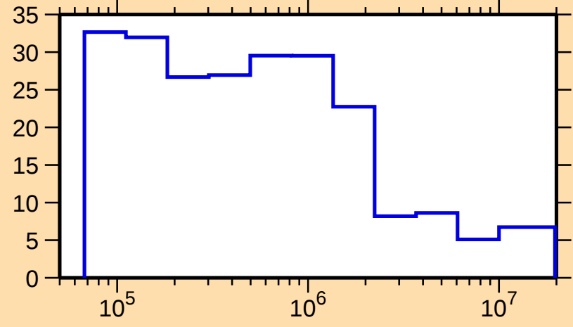
\Delta\sigma/\sigma vs. E for ^{265}\text{Lw}(n,n\text{oncl.})
