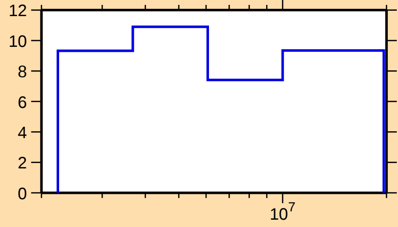
\Delta\sigma/\sigma vs. E for ^{265}\text{Lw}(n,f)
