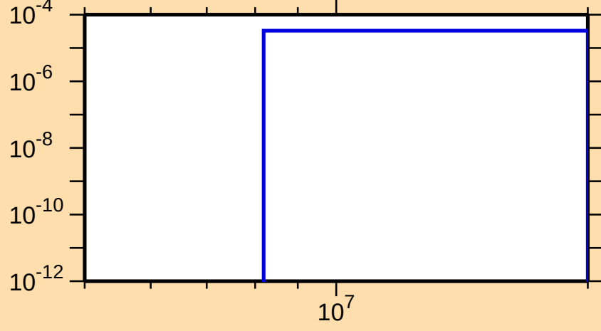
\sigma vs. E for ^{265}\text{Lw}(n,t)
