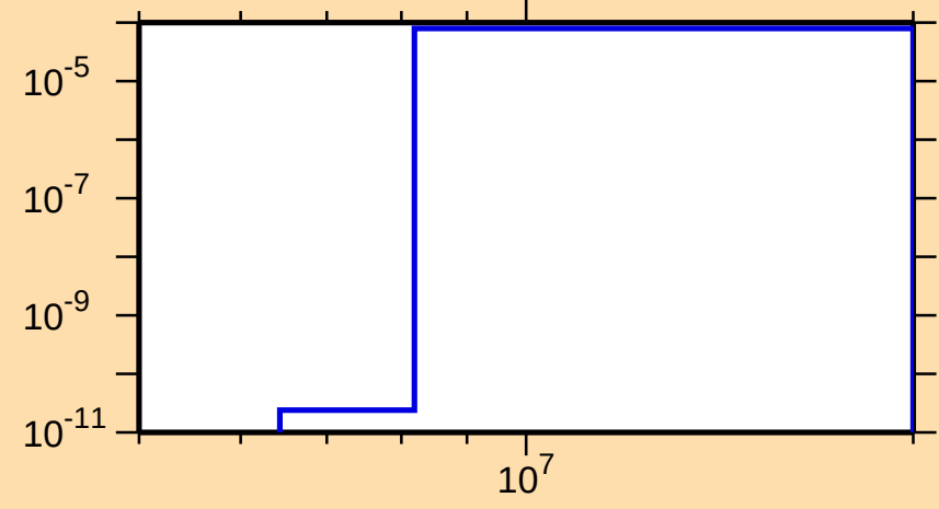
\sigma vs. E for ^{265}\text{Lw}(n,d)
