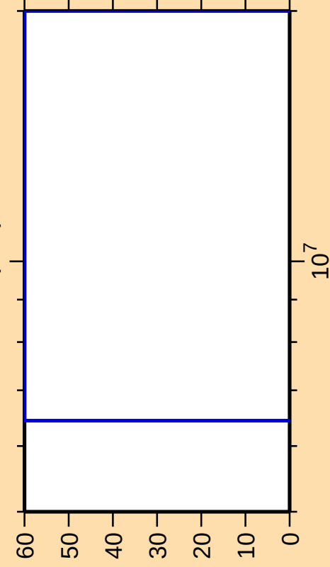
\Delta\sigma/\sigma vs. E for ^{265}\text{Lw}(n,d)
