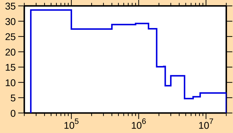
\Delta\sigma/\sigma vs. E for ^{265}\text{Lw}(n,n\text{onel.})
