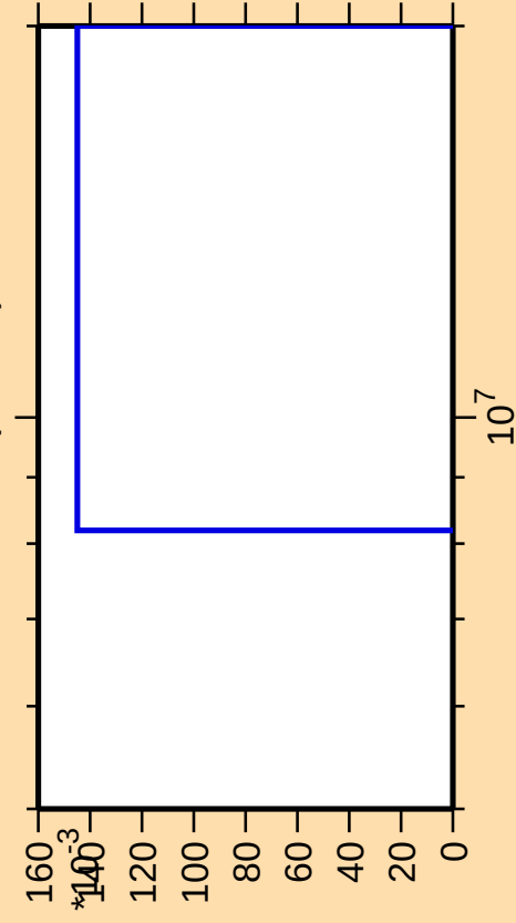
\Delta\sigma/\sigma vs. E for ^{265}\text{Lw}(n,3n\alpha)
