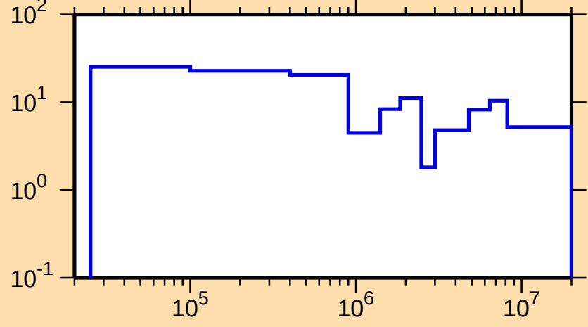
\Delta\sigma/\sigma vs. E for ^{265}\text{Lw}(n,\text{tot.})
