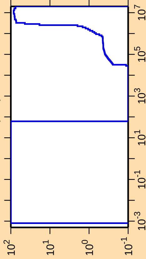
\Delta\sigma/\sigma vs. E for ^{266}\text{Lw}(n,\alpha)
