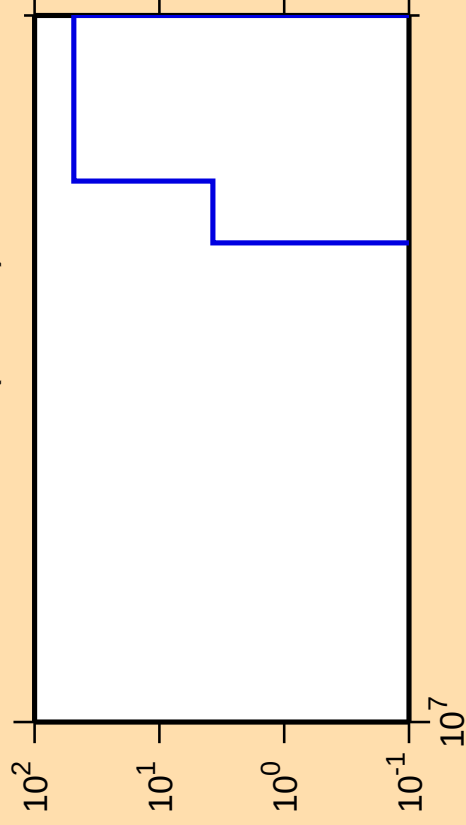
\Delta\sigma/\sigma vs. E for ^{266}\text{Lw}(n,\text{He3})
