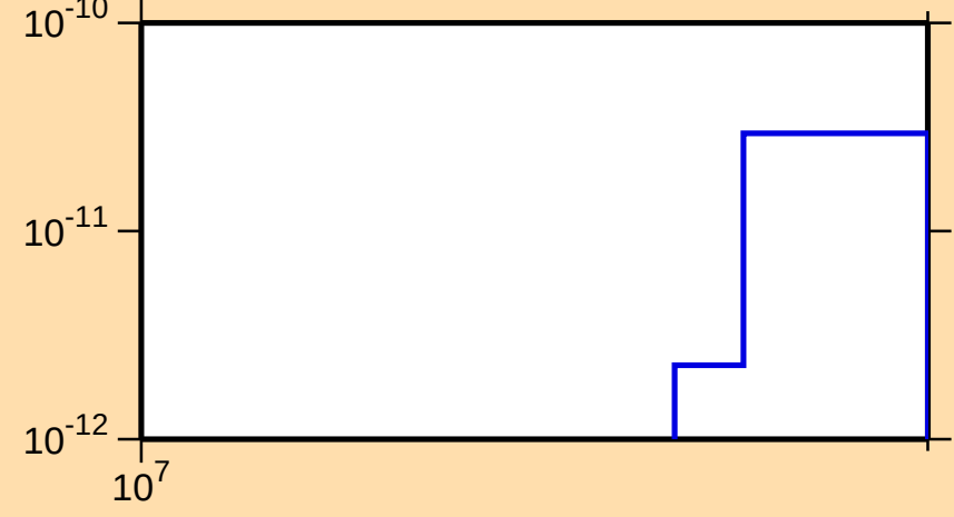
\sigma vs. E for ^{266}\text{Lw}(n,\text{He3})
