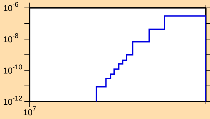
\sigma vs. E for ^{266}\text{Lw}(n,nd)
