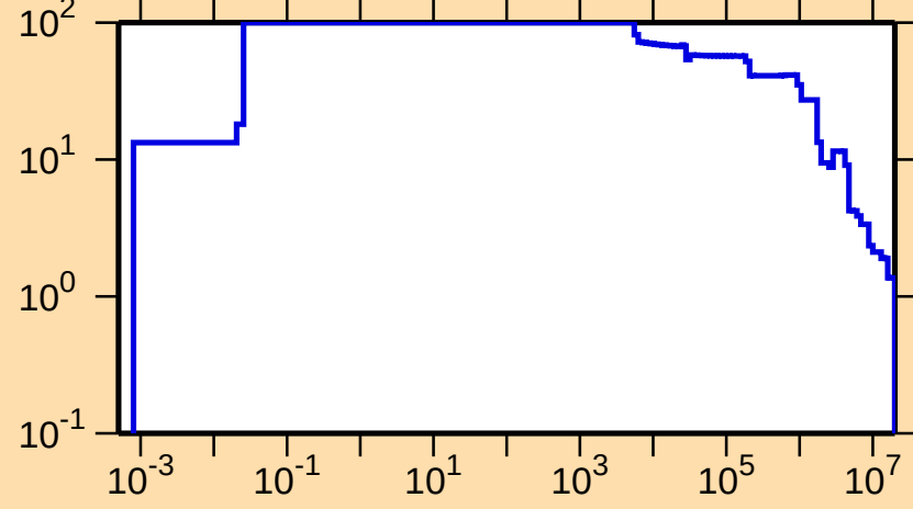
\Delta\sigma/\sigma vs. E for ^{266}\text{Lw}(n,\text{nonel.})
