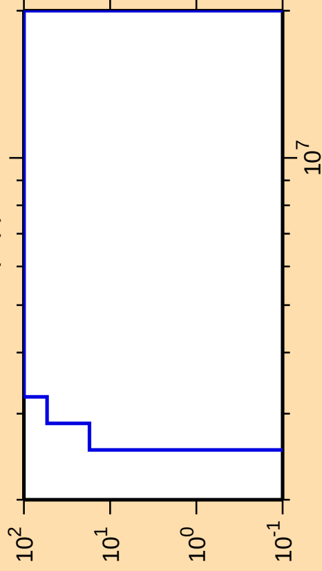
\Delta\sigma/\sigma vs. E for ^{266}\text{Lw}(n,p)
