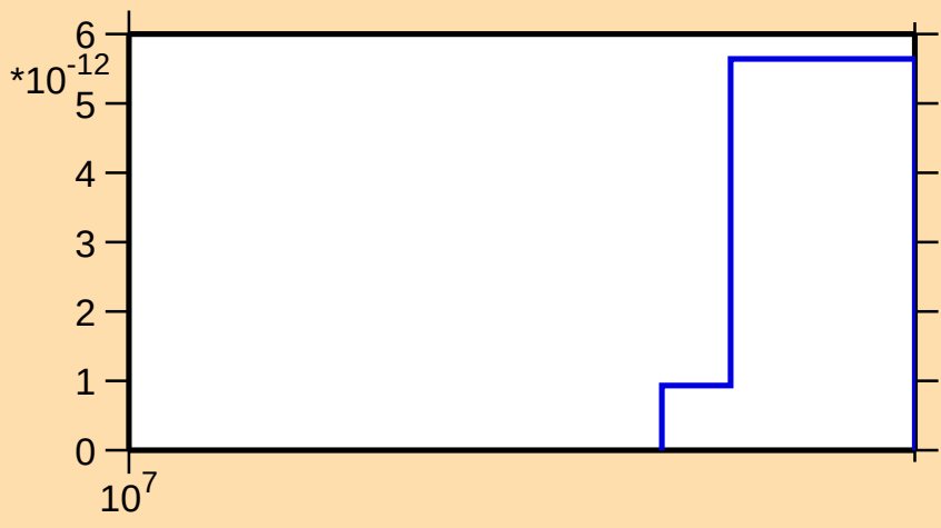
\sigma vs. E for ^{266}\text{Lw}(n,3n\alpha)
