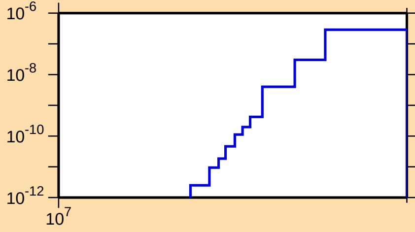
\sigma vs. E for ^{266}\text{Lw}(n,nt)
