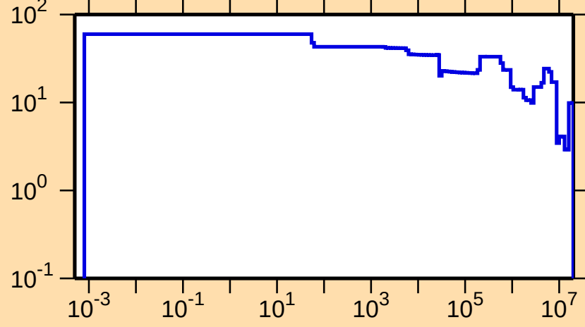
\Delta\sigma/\sigma vs. E for ^{266}\text{Lw}(n,\text{el.})
