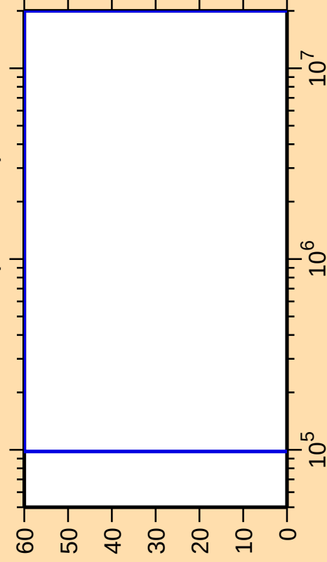
\Delta\sigma/\sigma vs. E for ^{266}\text{Lw}(n,n\text{cont.})
