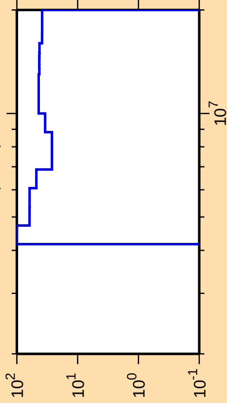
\Delta\sigma/\sigma vs. E for ^{266}\text{Lw}(n,2n)
