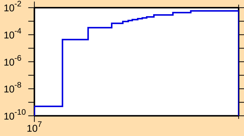
\sigma vs. E for ^{266}\text{Lw}(n,3n)
