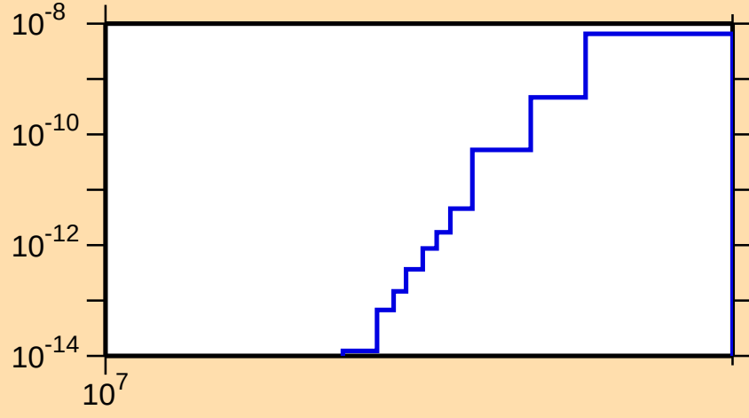
\sigma vs. E for ^{266}\text{Lw}(n,2np)
