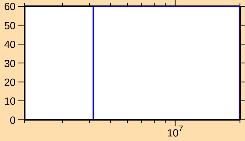
\Delta\sigma/\sigma vs. E for ^{266}\text{Lw}(n,\text{inel.})
