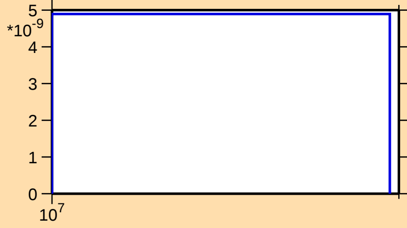
\sigma vs. E for ^{266}\text{Lw}(n,nt)
