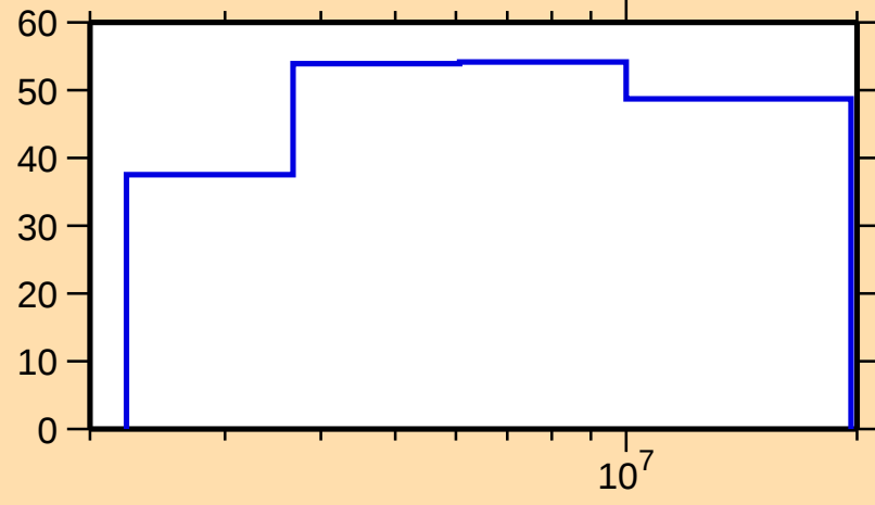
\Delta\sigma/\sigma vs. E for ^{266}\text{Lw}(n,n_1)
