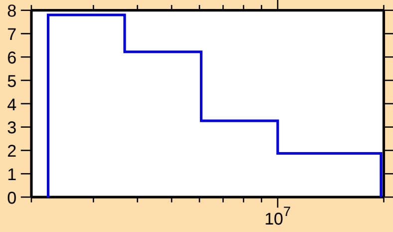
\Delta\sigma/\sigma vs. E for ^{266}\text{Lw}(n,f)
