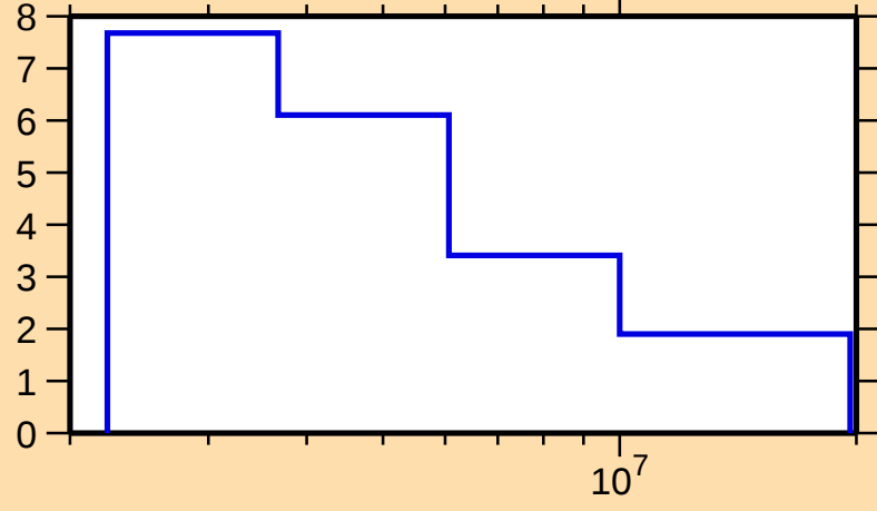
\Delta\sigma/\sigma vs. E for ^{266}\text{Lw}(n,\text{nonel.})
