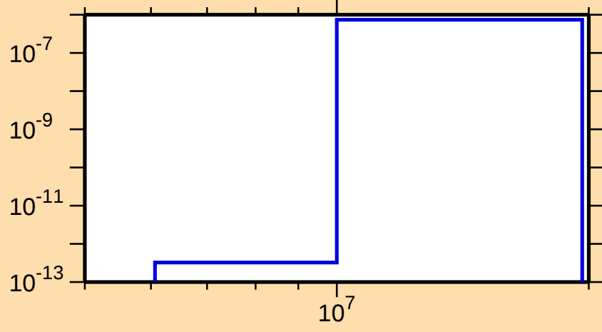
\sigma vs. E for ^{266}\text{Lw}(n,np)
