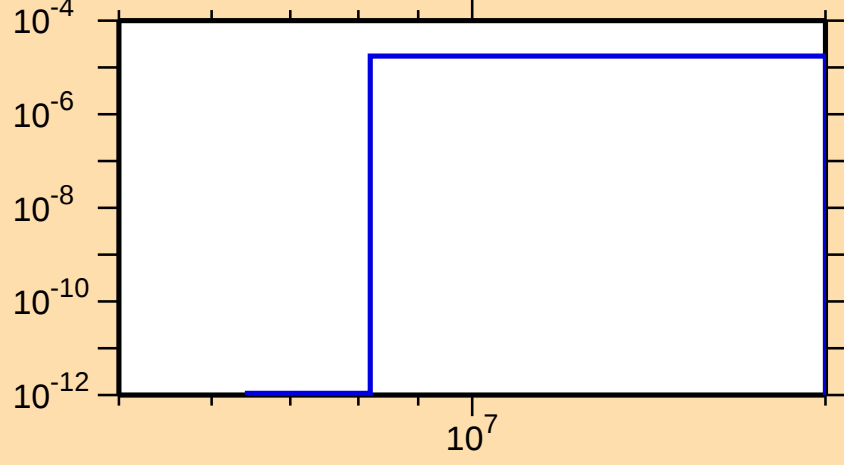
\sigma vs. E for ^{266}\text{Lw}(n,d)
