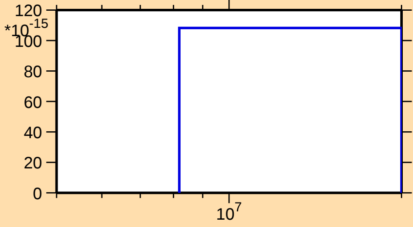
\sigma vs. E for ^{266}\text{Lw}(n,3n\alpha)
