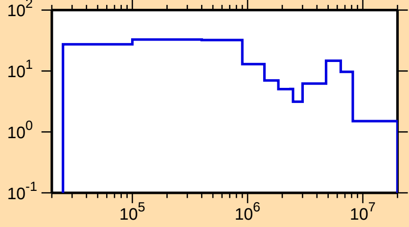
\Delta\sigma/\sigma vs. E for ^{266}\text{Lw}(n,\text{tot.})
