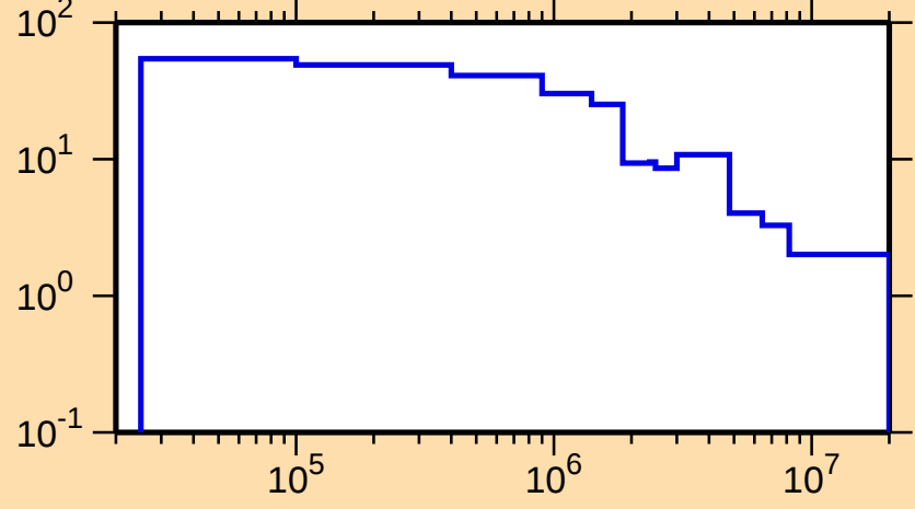
\Delta\sigma/\sigma vs. E for ^{266}\text{Lw}(n,f)
