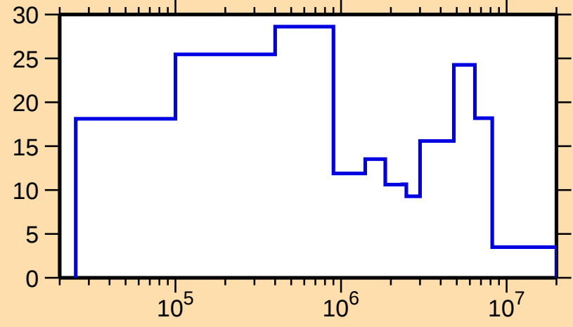
\Delta\sigma/\sigma vs. E for ^{266}\text{Lw}(n,\text{el.})
