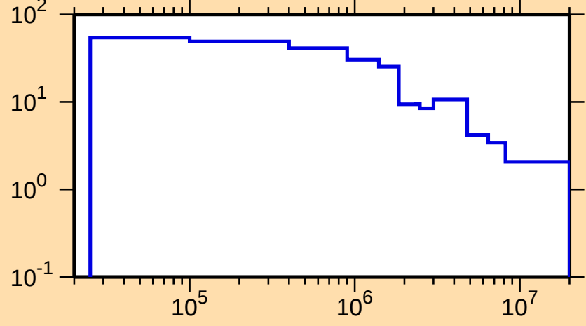
\Delta\sigma/\sigma vs. E for ^{266}\text{Lw}(n,n\text{onel.})
