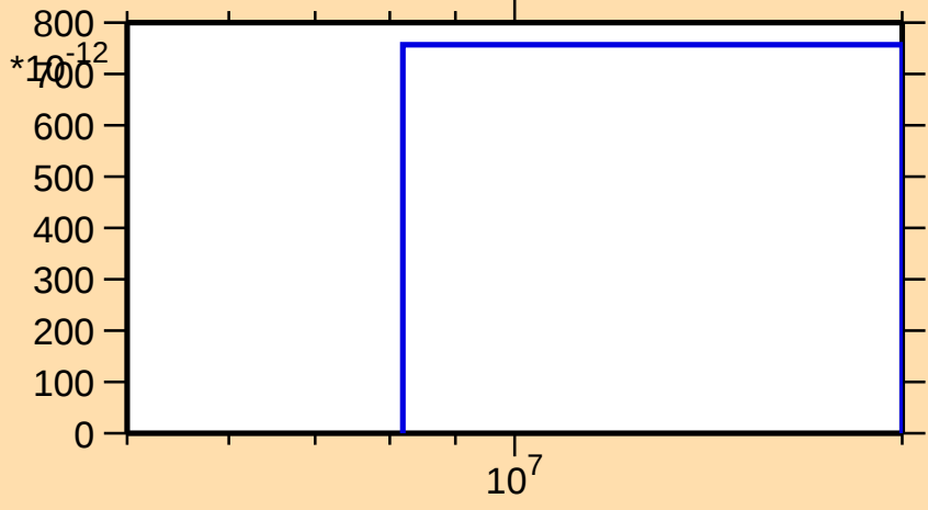
\sigma vs. E for ^{266}\text{Lw}(n,2n\alpha)
