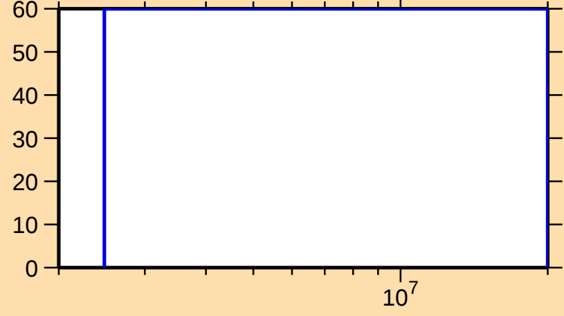
\Delta\sigma/\sigma vs. E for ^{266}\text{Lw}(n,n\text{cont.})
