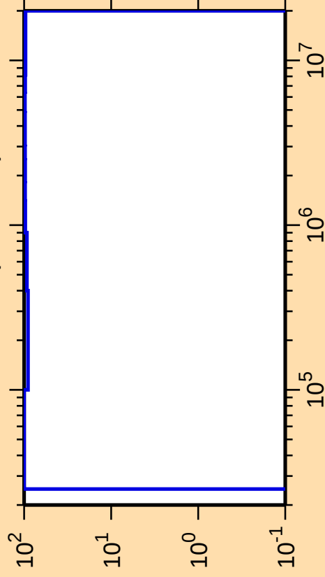
\Delta\sigma/\sigma vs. E for ^{266}\text{Lw}(n,\text{ncont.})
