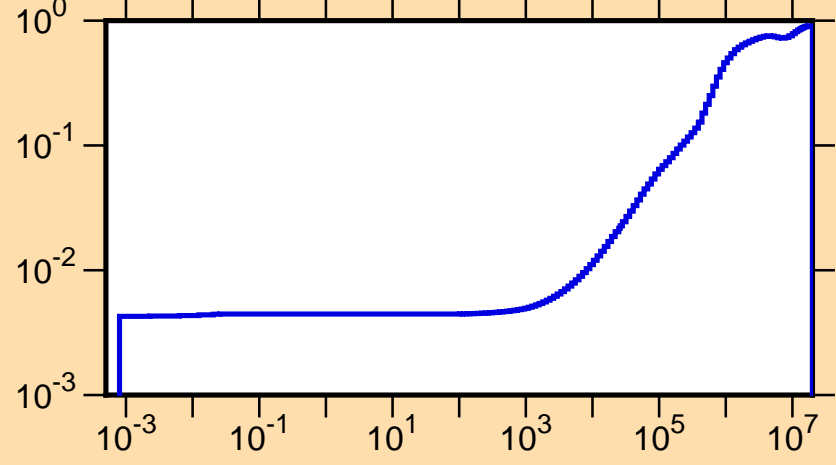
\mu vs. E for ^{158}\text{Lu}(\text{mt251})
