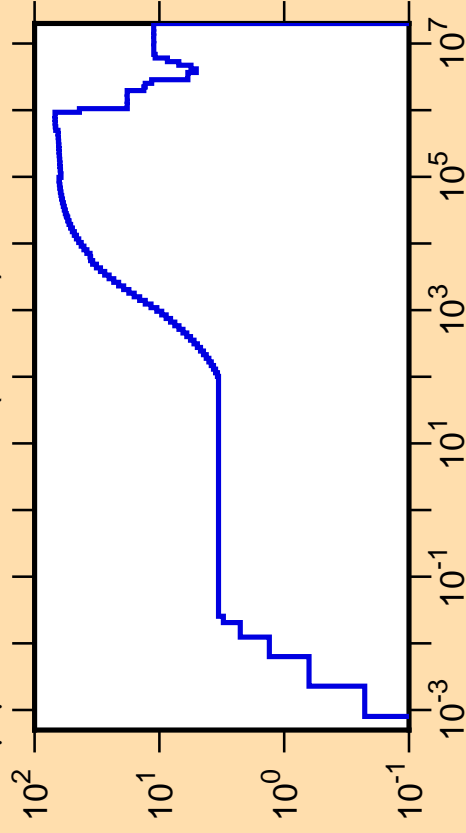
\Delta\mu/\mu vs. E for ^{158}\text{Lu}(\text{mt251})
