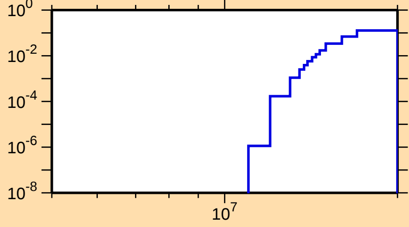
\sigma vs. E for ^{158}\text{Lu}(n,2np)
