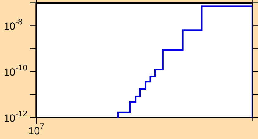
\sigma vs. E for ^{158}\text{Lu}(\text{mt } 34)
