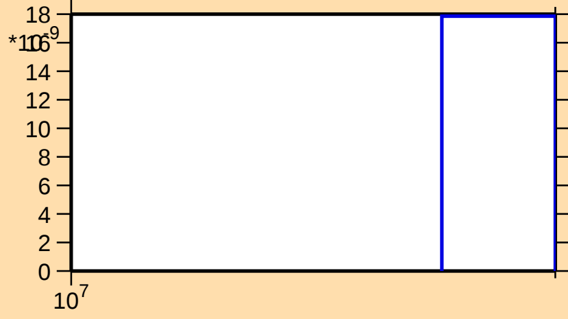
\sigma vs. E for ^{158}\text{Lu}(n,3n)
