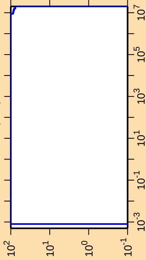
\Delta\sigma/\sigma vs. E for ^{158}\text{Lu}(n,\alpha)
