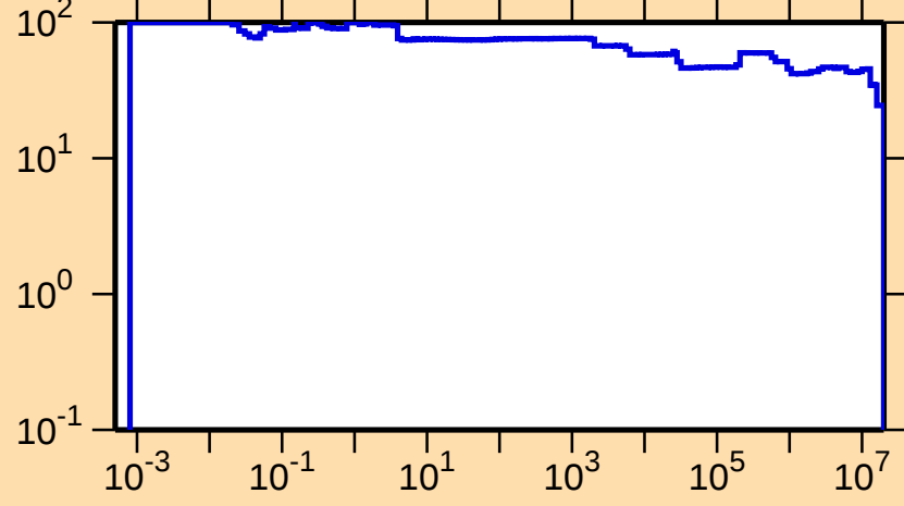
\Delta\sigma/\sigma vs. E for ^{158}\text{Lu}(n,p)
