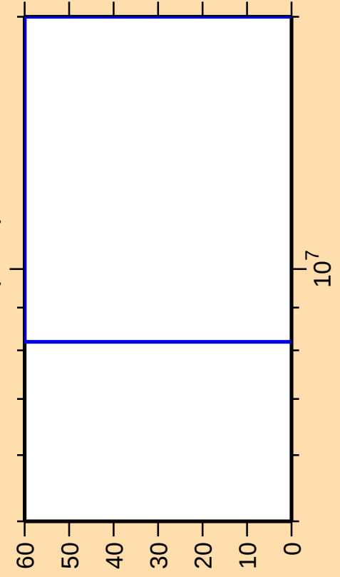
\Delta\sigma/\sigma vs. E for ^{158}\text{Lu}(n,3n)
