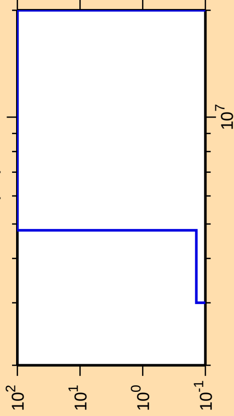
\Delta\sigma/\sigma vs. E for ^{158}\text{Lu}(n,t)
