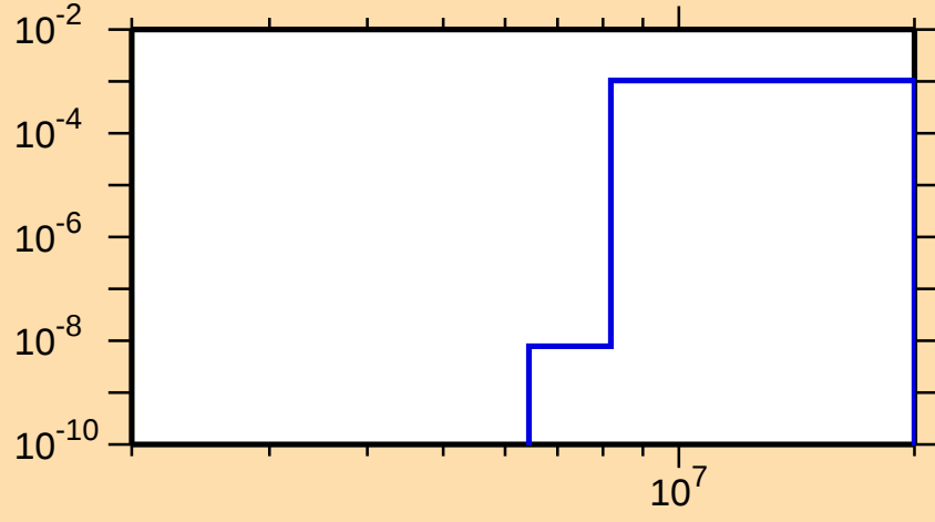
\sigma vs. E for ^{158}\text{Lu}(n,t)
