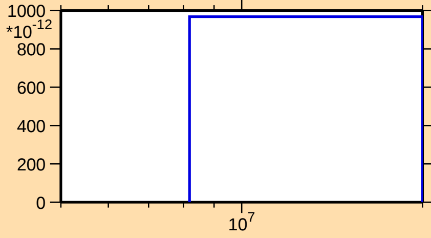
\sigma vs. E for ^{158}\text{Lu}(\text{mt } 34)
