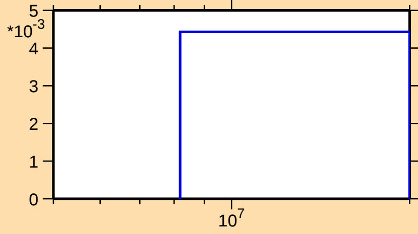
\sigma vs. E for ^{158}\text{Lu}(n,2n\alpha)
