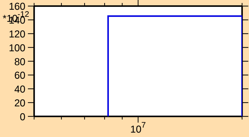
\sigma vs. E for ^{158}\text{Lu}(n,3n)
