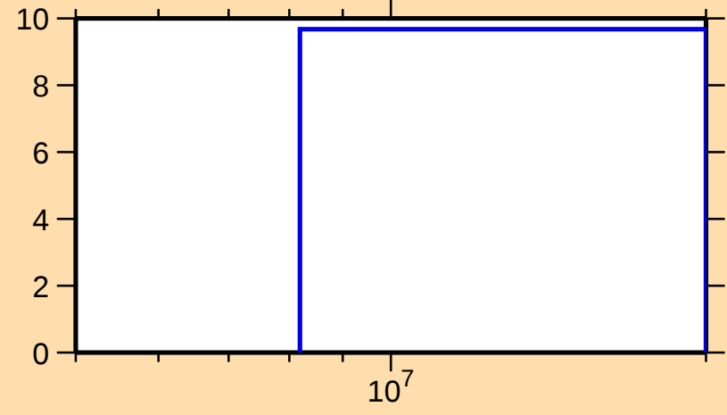
\Delta\sigma/\sigma vs. E for ^{158}\text{Lu}(n,\text{el.})
