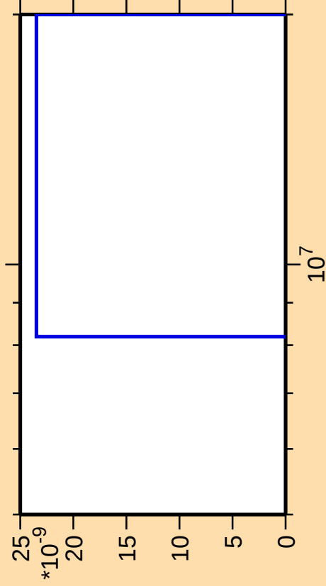
\Delta\sigma/\sigma vs. E for ^{158}\text{Lu}(\text{mt 11})
