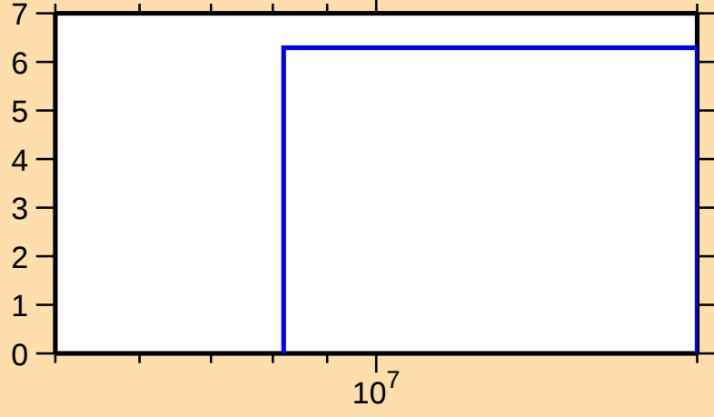
\Delta\sigma/\sigma vs. E for ^{158}\text{Lu}(n,\text{tot.})
