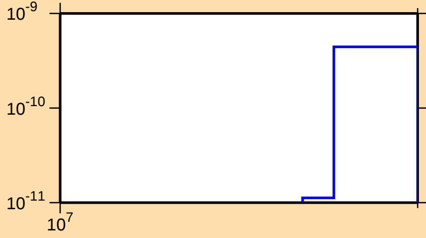
\sigma vs. E for ^{159}\text{Lu}(\text{mt 34})
