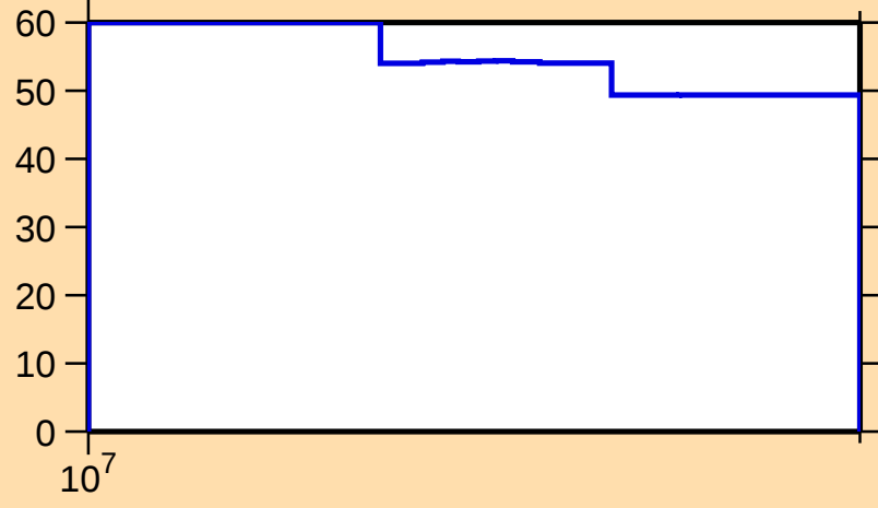
\Delta\sigma/\sigma vs. E for ^{159}\text{Lu}(n,\text{inel.})
