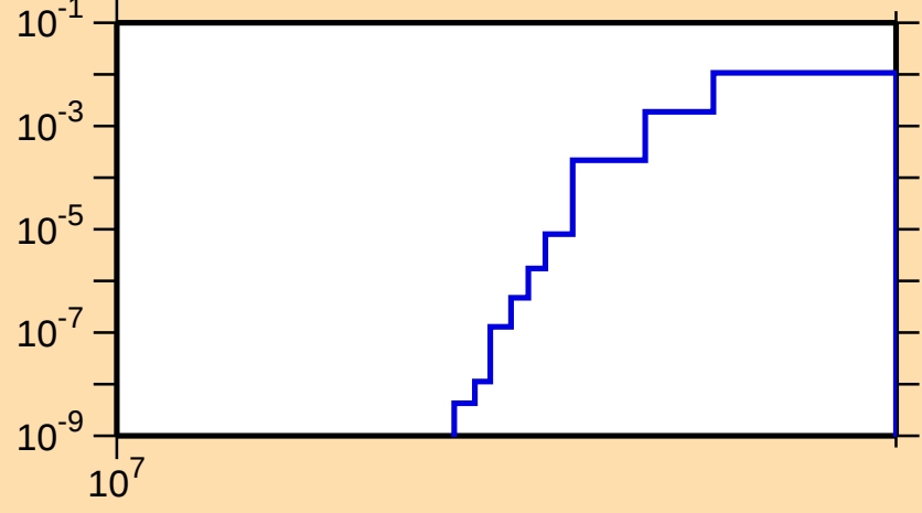
\sigma vs. E for ^{159}\text{Lu}(n,2np)
