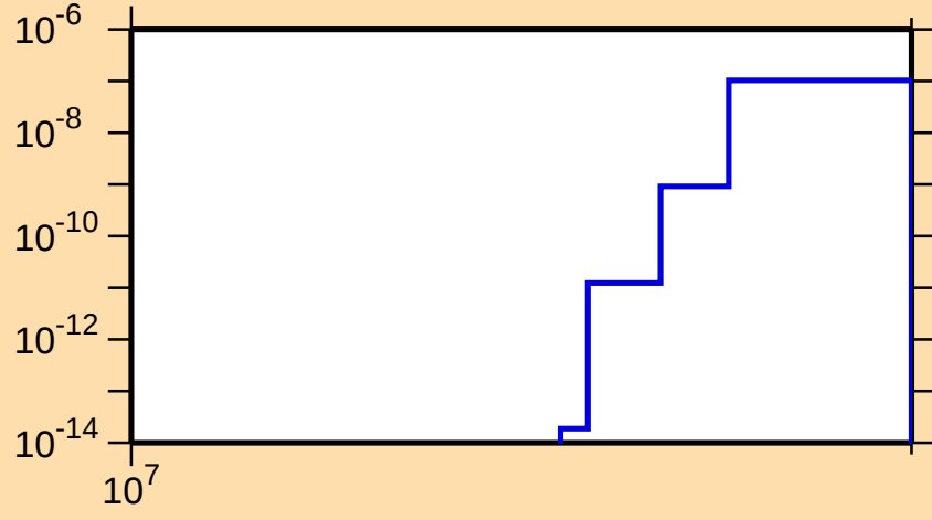
\sigma vs. E for ^{159}\text{Lu}(n,\text{nt})
