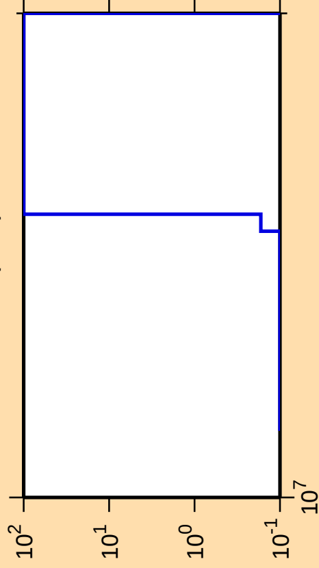
\Delta\sigma/\sigma vs. E for ^{159}\text{Lu}(n,\text{nt})
