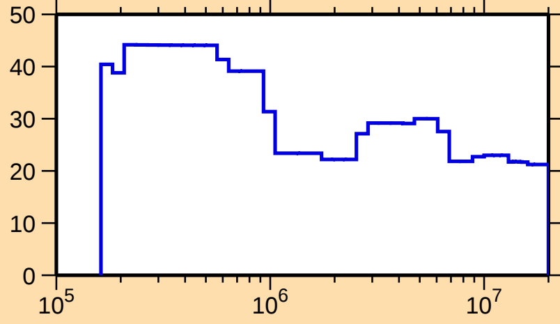
\Delta\sigma/\sigma vs. E for ^{159}\text{Lu}(n,n\text{onel.})
