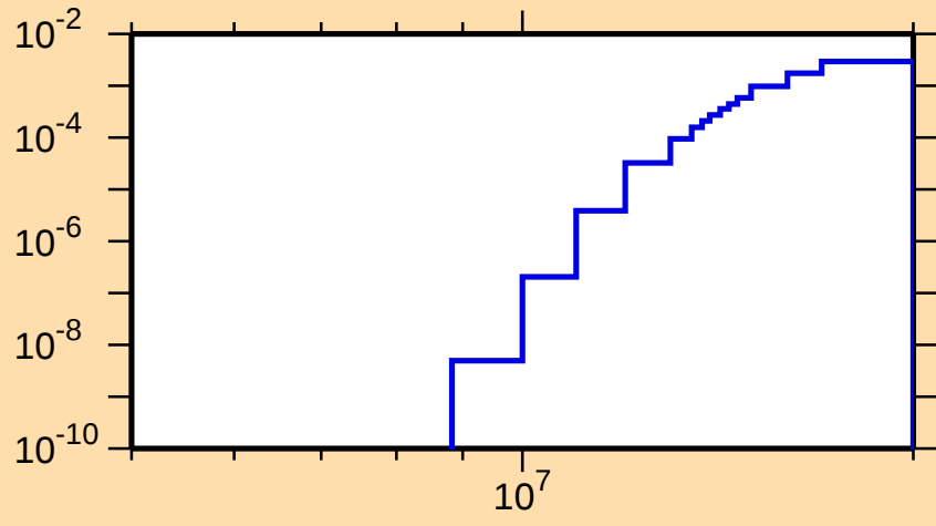
\sigma vs. E for ^{159}\text{Lu}(n,t)
