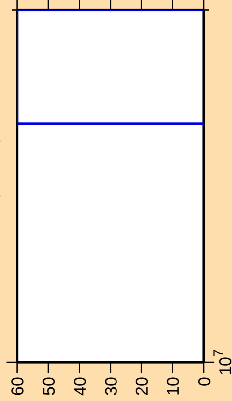
\Delta\sigma/\sigma vs. E for ^{159}\text{Lu}(\text{mt 34})
