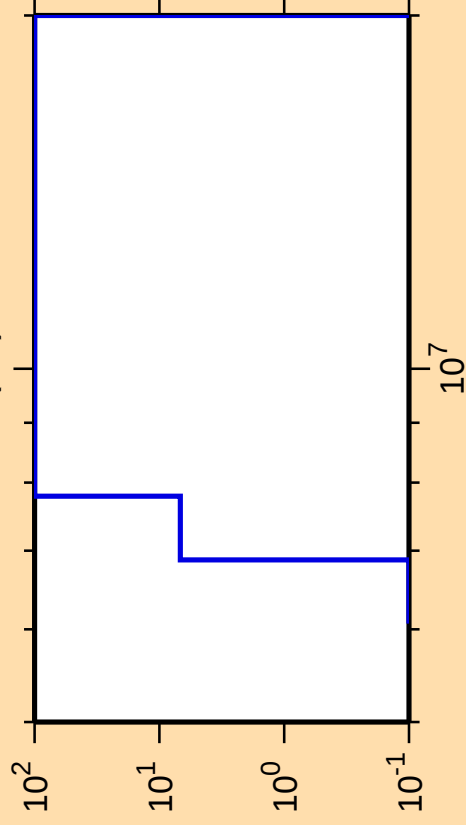
\Delta\sigma/\sigma vs. E for ^{159}\text{Lu}(n,t)
