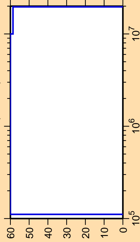
\Delta\sigma/\sigma vs. E for ^{159}\text{Lu}(n,\text{inel.})
