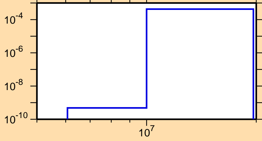
\sigma vs. E for ^{159}\text{Lu}(n,t)
