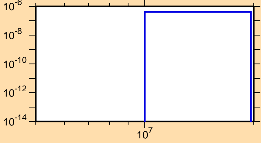
\sigma vs. E for ^{159}\text{Lu}(n,pd)
