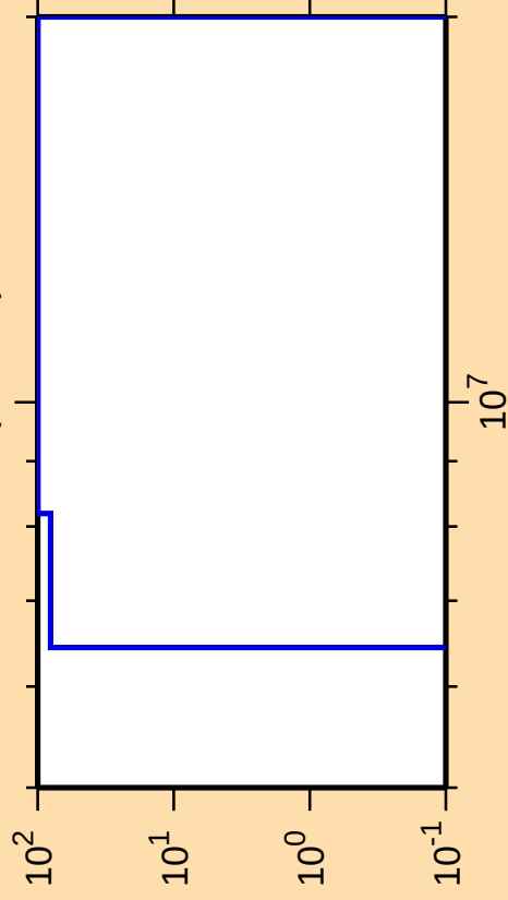
\Delta\sigma/\sigma vs. E for ^{159}\text{Lu}(n,\text{He}3)
