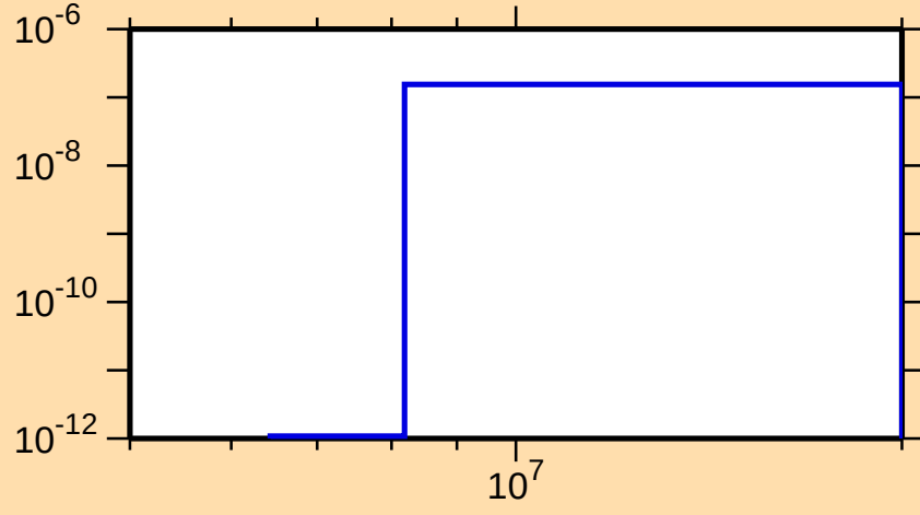
\sigma vs. E for ^{159}\text{Lu}(\text{mt117})
