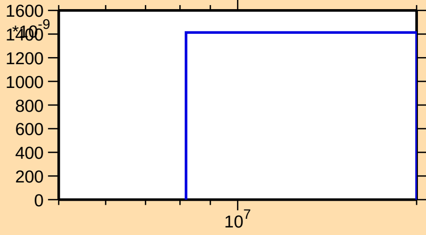
\sigma vs. E for ^{159}\text{Lu}(n,2n\alpha)
