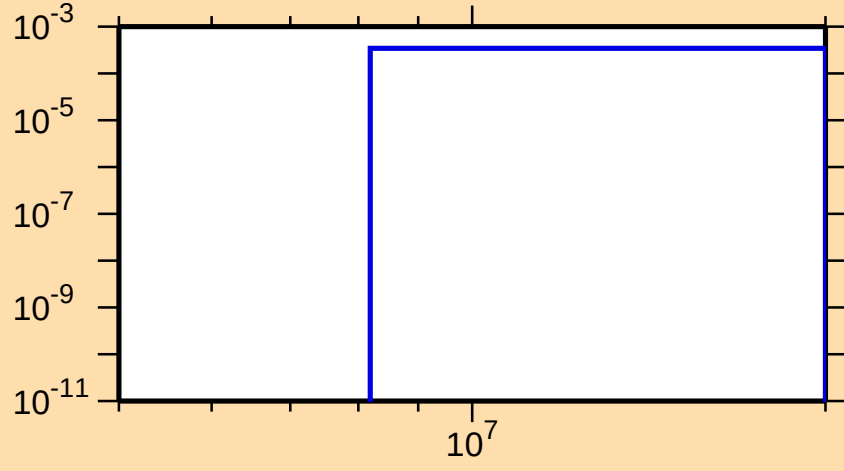
\sigma vs. E for ^{159}\text{Lu}(n,t)
