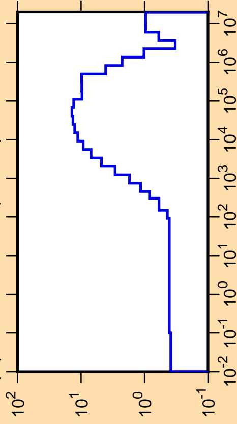
\Delta\mu/\mu vs. E for ^{175}\text{Lu}(\text{mt251})
