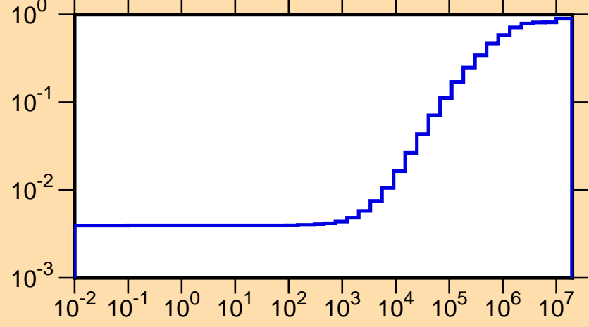
\mu vs. E for ^{175}\text{Lu}(\text{mt251})
