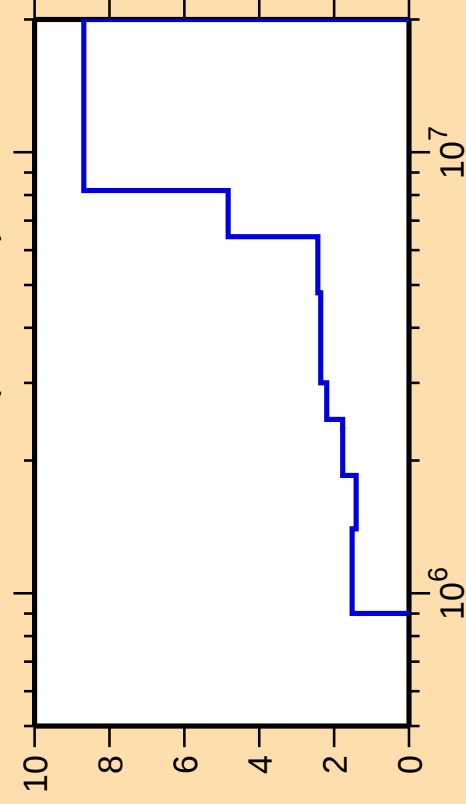
\Delta\sigma/\sigma vs. E for ^{175}\text{Lu}(n,\text{ncont.})
