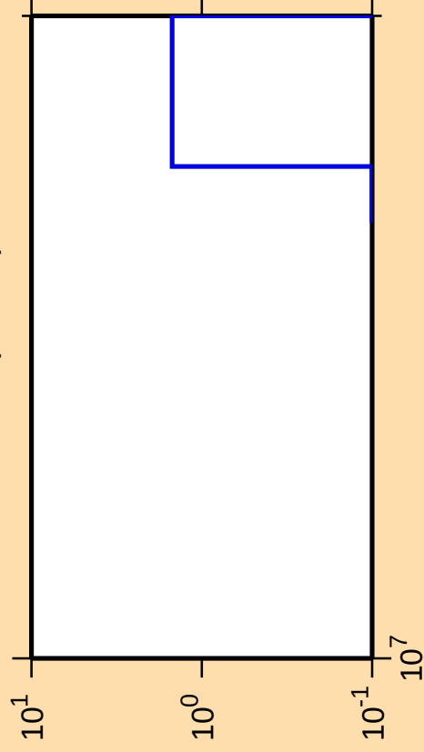
\Delta\sigma/\sigma vs. E for ^{183}\text{Lu}(n,3n\alpha)
