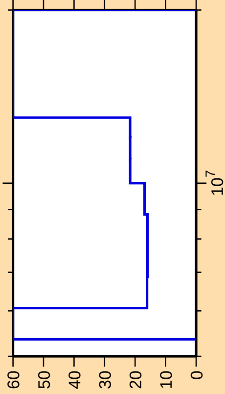
\Delta\sigma/\sigma vs. E for ^{183}\text{Lu}(n,2n)
