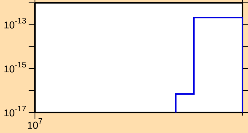
\sigma vs. E for ^{183}\text{Lu}(n,3n\alpha)
