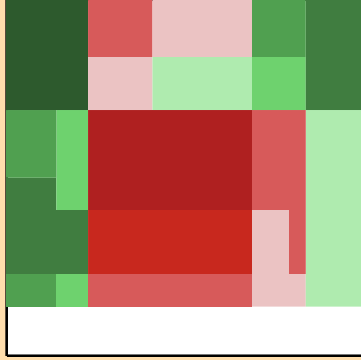
\Delta\sigma/\sigma vs. E for ^{183}\text{Lu}(n,\text{tot.})
