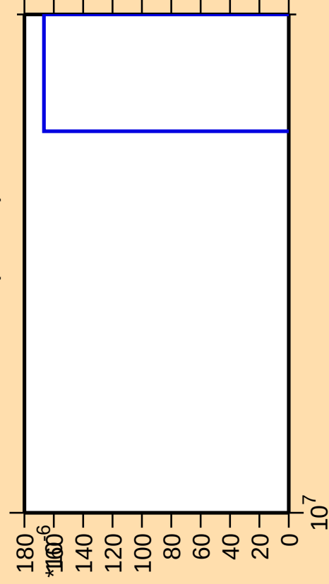
\Delta\sigma/\sigma vs. E for ^{183}\text{Lu} (mt 42)
