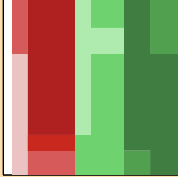
\Delta\sigma/\sigma vs. E for ^{183}\text{Lu}(n,2n)
