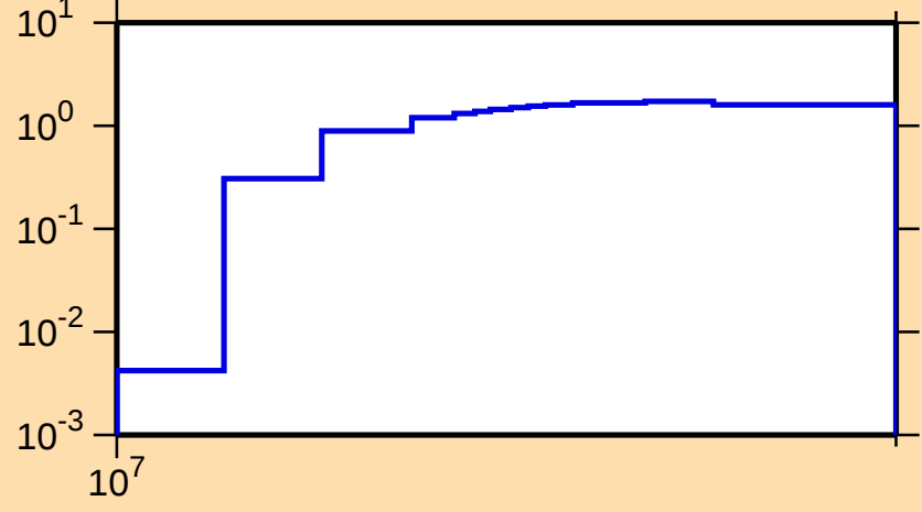
\sigma vs. E for ^{184}\text{Lu}(n,3n)
