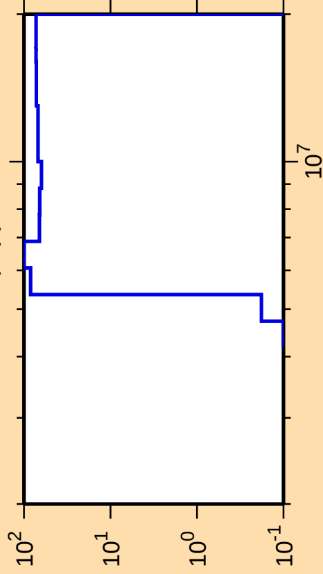
\Delta\sigma/\sigma vs. E for ^{184}\text{Lu}(n,p)
