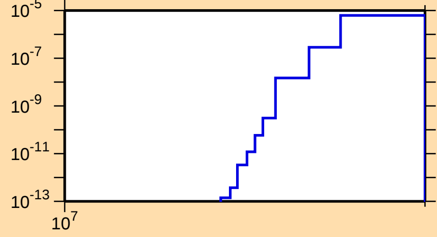
\sigma vs. E for ^{184}\text{Lu}(n,\text{nd})
