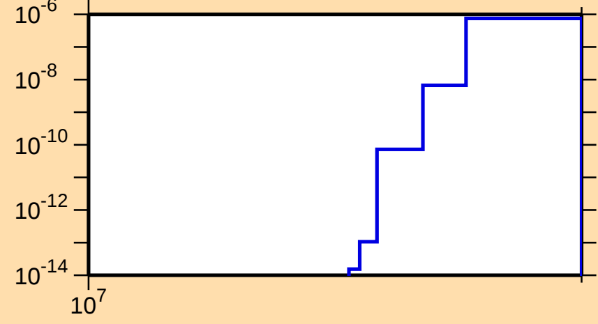
\sigma vs. E for ^{184}\text{Lu}(n,2np)
