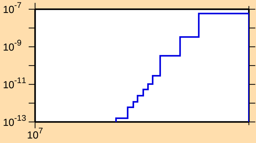
\sigma vs. E for ^{184}\text{Lu}(n,2n\alpha)
