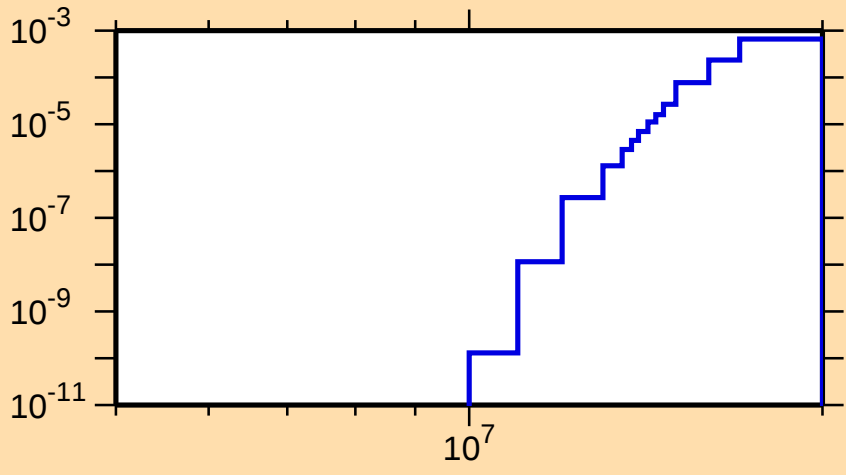
\sigma vs. E for ^{184}\text{Lu}(n,d)
