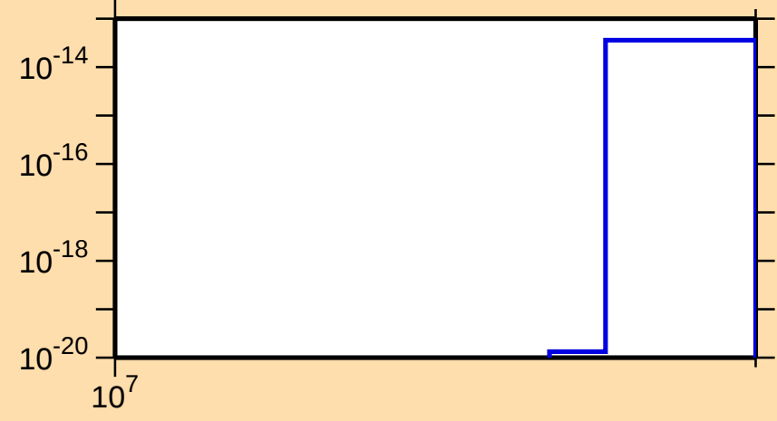
\sigma vs. E for ^{184}\text{Lu}(\text{mt 11})
