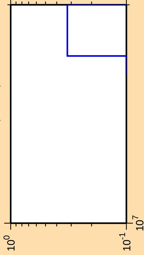
\Delta\sigma/\sigma vs. E for ^{184}\text{Lu}(\text{mt 11})
