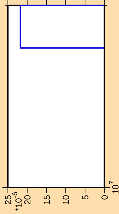
\Delta\sigma/\sigma vs. E for ^{184}\text{Lu}(\text{mt } 42)
