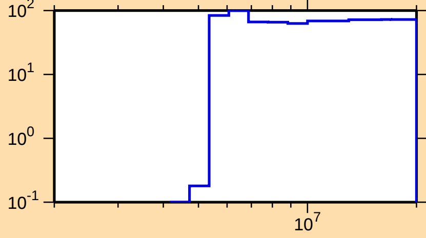
\Delta\sigma/\sigma vs. E for ^{184}\text{Lu}(n,p)
