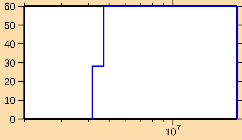
\Delta\sigma/\sigma vs. E for ^{184}\text{Lu}(n,n\text{cont.})
