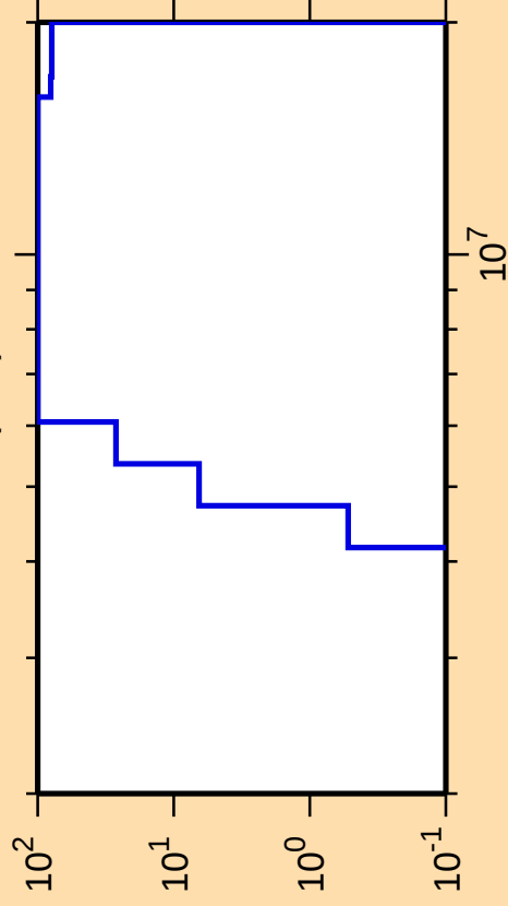
\Delta\sigma/\sigma vs. E for ^{184}\text{Lu}(n,\alpha)
