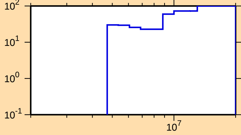
\Delta\sigma/\sigma vs. E for ^{184}\text{Lu}(n,2n)
