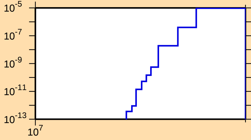
\sigma vs. E for ^{184}\text{Lu}(n,nt)
