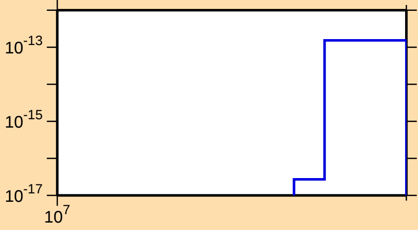
\sigma vs. E for ^{184}\text{Lu}(n,3n\alpha)
