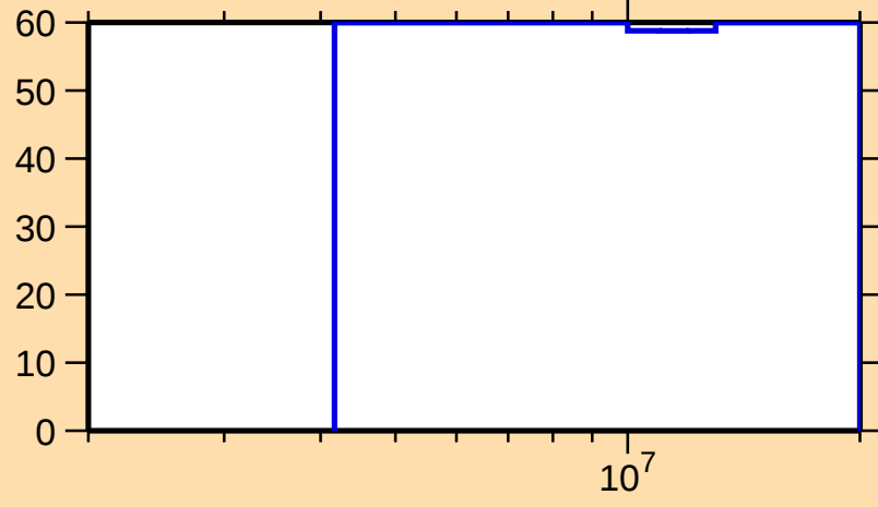
\Delta\sigma/\sigma vs. E for ^{184}\text{Lu}(n,\gamma)
