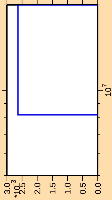
\Delta\sigma/\sigma vs. E for ^{184}\text{Lu}(\text{mt 11})
