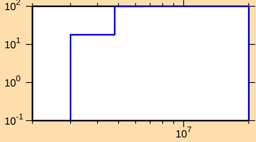
\Delta\sigma/\sigma vs. E for ^{184}\text{Lu}(n,n\text{cont.})
