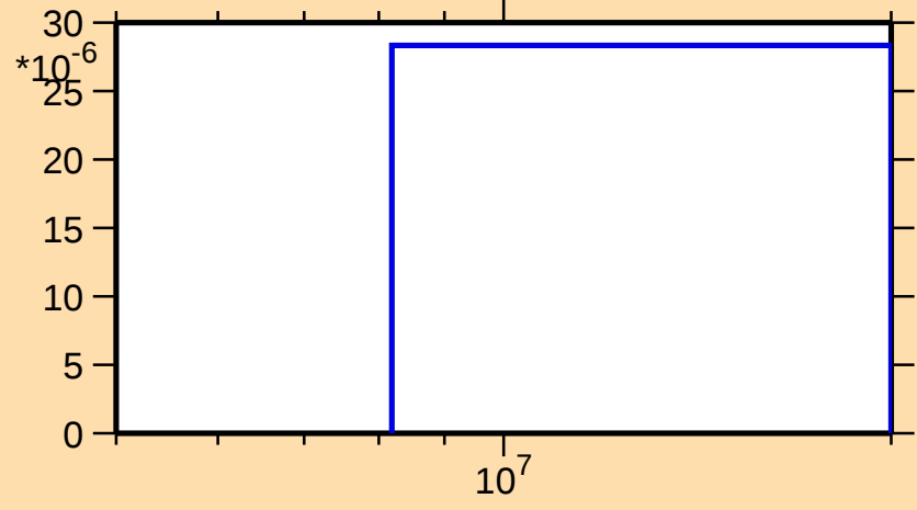
\sigma vs. E for ^{184}\text{Lu}(n,d)
