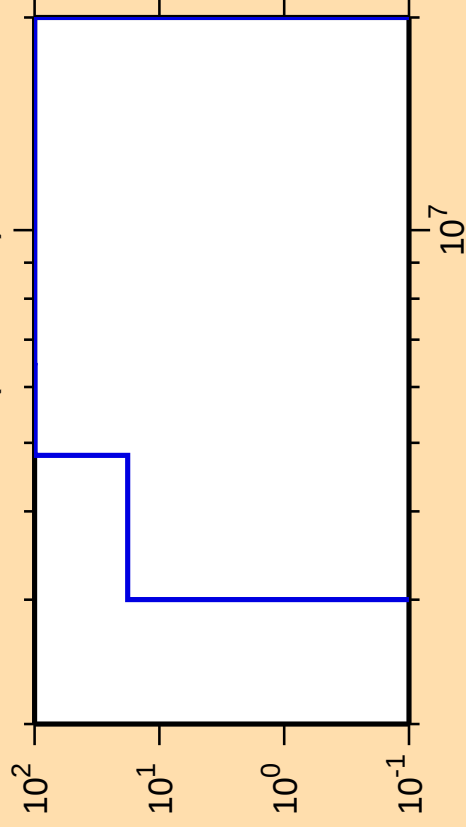
\Delta\sigma/\sigma vs. E for ^{184}\text{Lu}(n,n\text{cont.})
