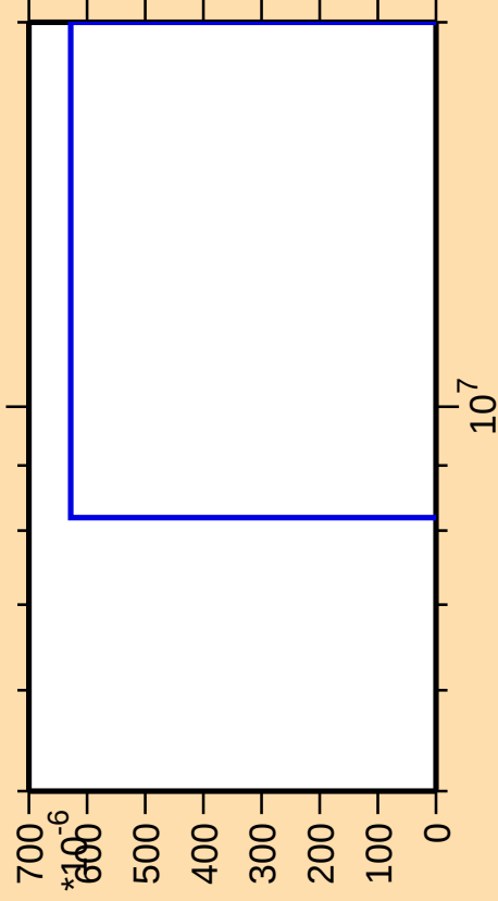
\Delta\sigma/\sigma vs. E for ^{184}\text{Lu}(n,3n\alpha)
