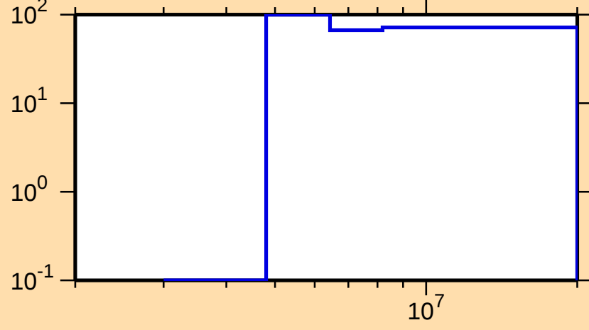
\Delta\sigma/\sigma vs. E for ^{184}\text{Lu}(n,p)
