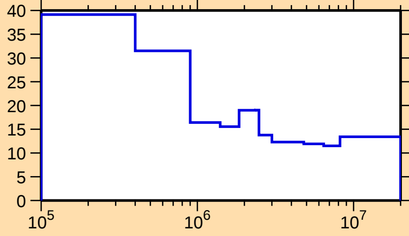
\Delta\sigma/\sigma vs. E for ^{184}\text{Lu}(n,n\text{onel.})
