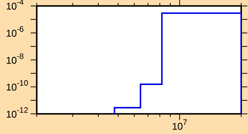
\sigma vs. E for ^{184}\text{Lu}(n,\alpha)
