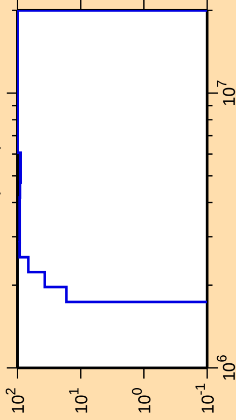
\Delta\sigma/\sigma vs. E for ^{254}\text{Md}(n,n\alpha)
