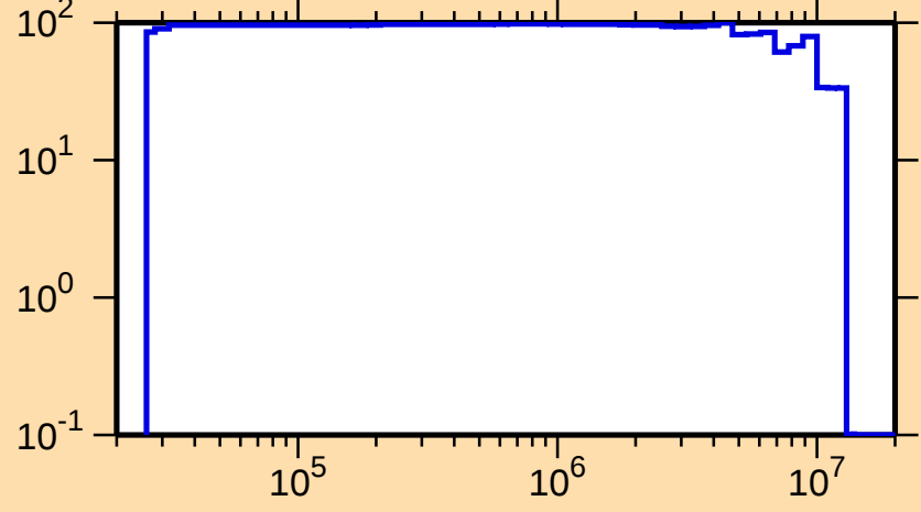
\Delta\sigma/\sigma vs. E for ^{254}\text{Md}(n,n_1)
