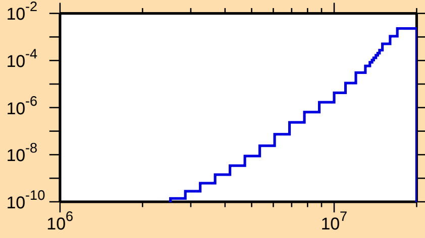
\sigma vs. E for ^{254}\text{Md}(n,n\alpha)
