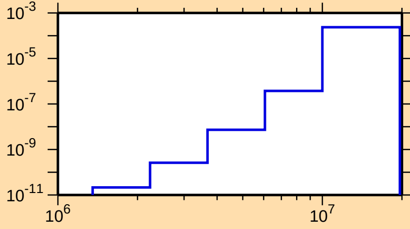
\sigma vs. E for ^{254}\text{Md}(n,n\alpha)
