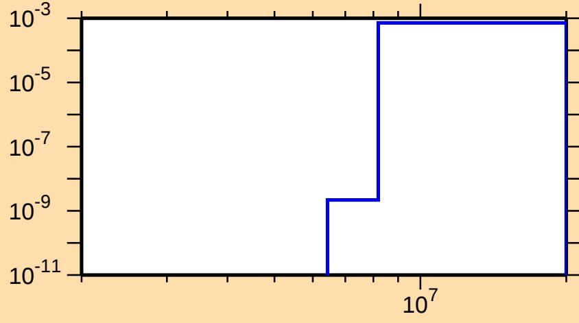
\sigma vs. E for ^{254}\text{Md}(n,d)
