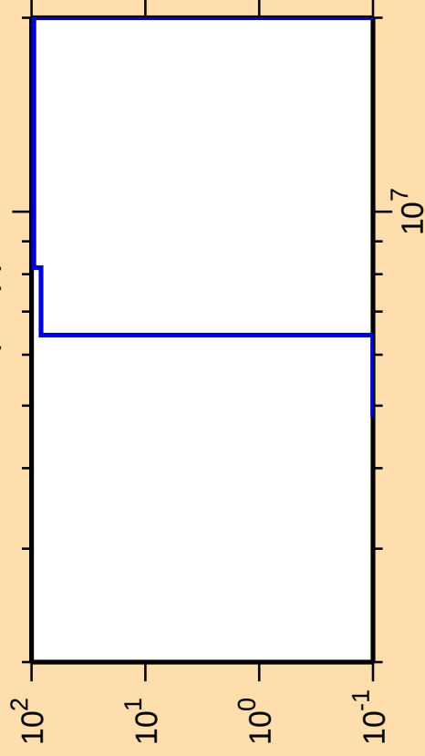
\Delta\sigma/\sigma vs. E for ^{254}\text{Md}(n,np)
