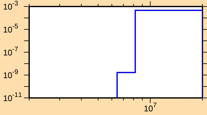
\sigma vs. E for ^{254}\text{Md}(n,np)
