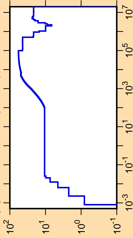
\Delta\mu/\mu vs. E for ^{127}\text{Nd}(\text{mt251})
