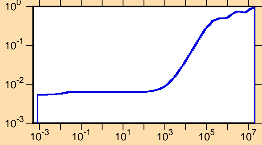
\mu vs. E for ^{127}\text{Nd}(\text{mt251})
