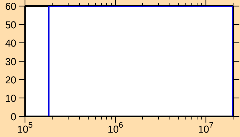
\Delta\sigma/\sigma vs. E for ^{127}\text{Nd}(n,ncont.)
