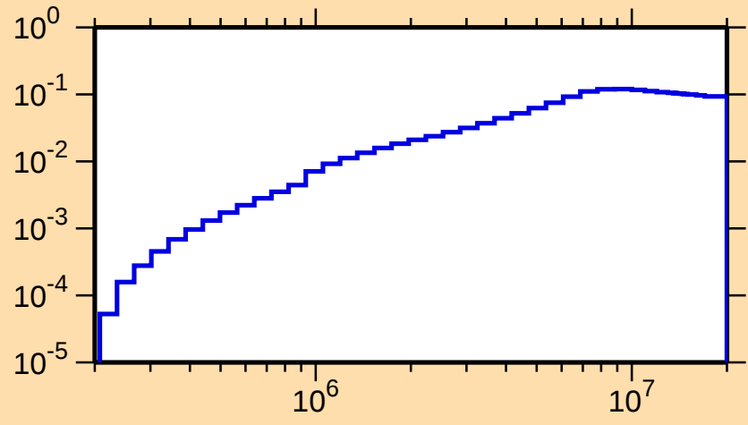
\sigma vs. E for ^{127}\text{Nd}(n,n\text{cont.})
