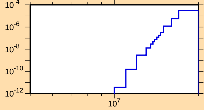
\sigma vs. E for ^{127}\text{Nd}(\text{mt } 45)
