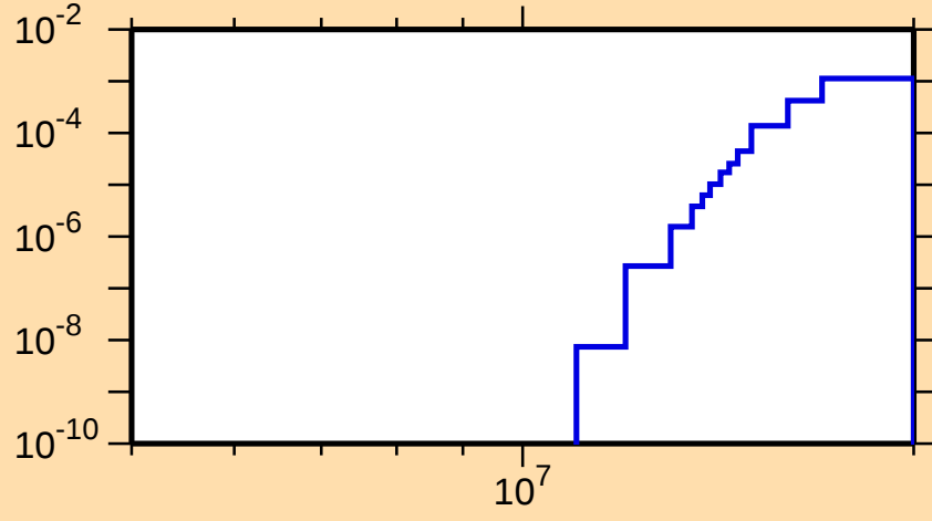
\sigma vs. E for ^{127}\text{Nd}(n,\text{pt})
