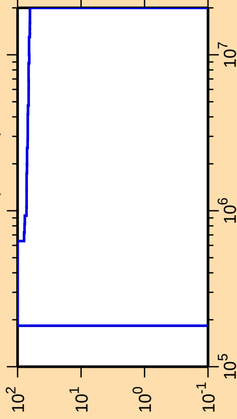
\Delta\sigma/\sigma vs. E for ^{127}\text{Nd}(n,\text{inel.})
