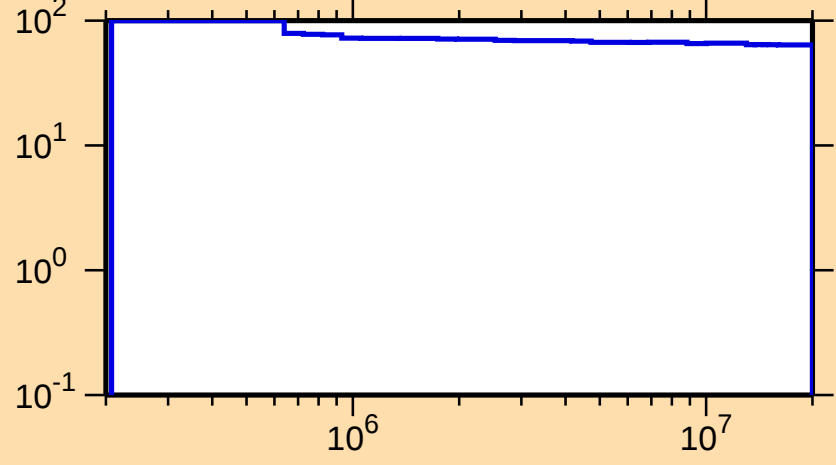
\Delta\sigma/\sigma vs. E for ^{127}\text{Nd}(n,\text{inel.})
