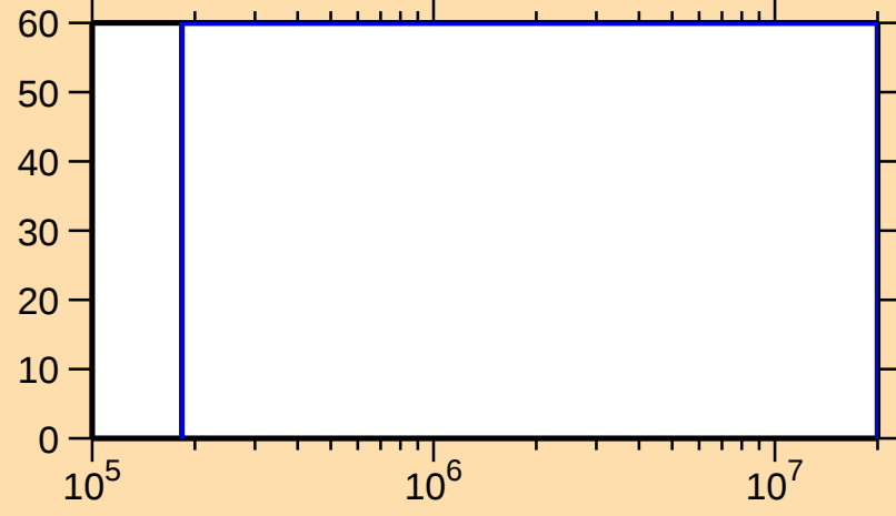
\Delta\sigma/\sigma vs. E for ^{127}\text{Nd}(n,\text{ncont.})
