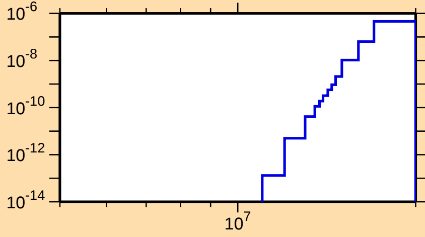
\sigma vs. E for ^{127}\text{Nd}(\text{mt } 34)
