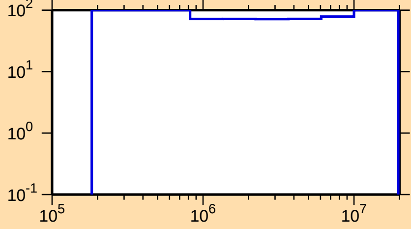
\Delta\sigma/\sigma vs. E for ^{127}\text{Nd}(n,n_1)
