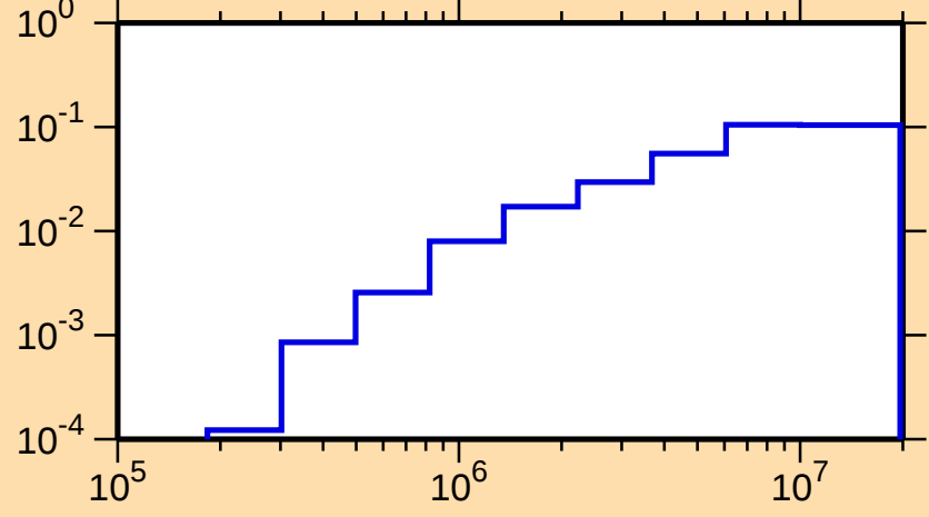
\sigma vs. E for ^{127}\text{Nd}(n,n\text{cont.})
