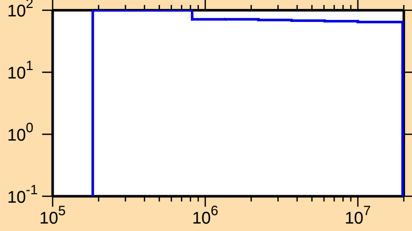
\Delta\sigma/\sigma vs. E for ^{127}\text{Nd}(n,\text{inel.})
