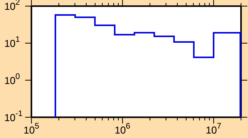
\Delta\sigma/\sigma vs. E for ^{127}\text{Nd}(n,\text{tot.})
