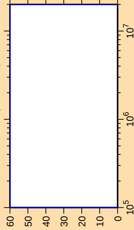
\Delta\sigma/\sigma vs. E for ^{127}\text{Nd}(n,\text{ncont.})
