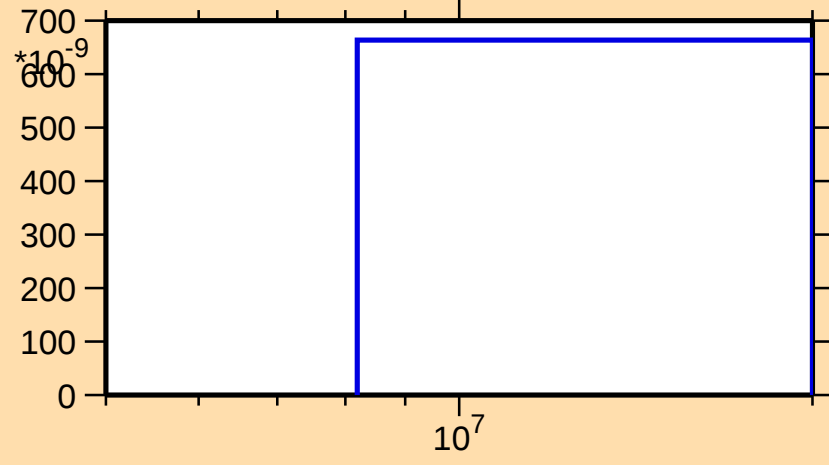
\sigma vs. E for ^{127}\text{Nd}(\text{mt } 45)
