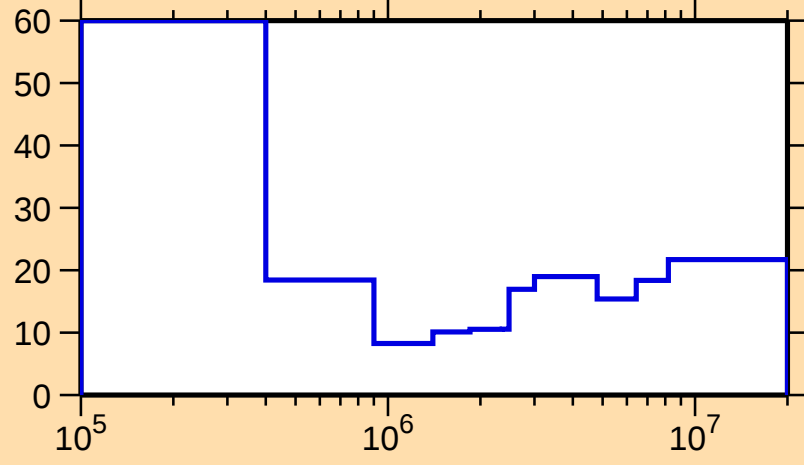
\Delta\sigma/\sigma vs. E for ^{127}\text{Nd}(n,n\text{onel.})
