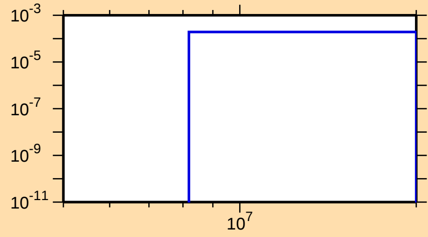
\sigma vs. E for ^{127}\text{Nd}(n,t)
