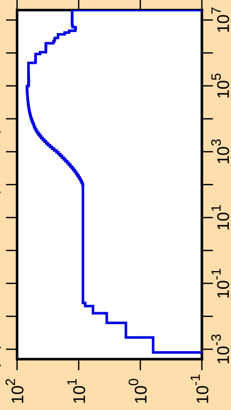
\Delta\mu/\mu vs. E for ^{128}\text{Nd}(\text{mt251})
