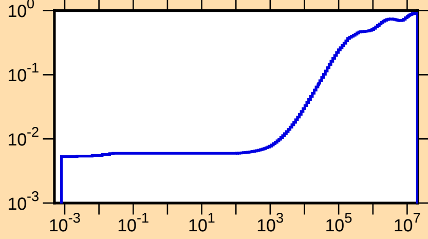
\mu vs. E for ^{128}\text{Nd}(\text{mt251})
