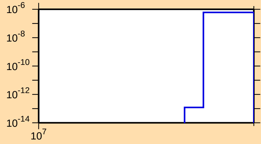
\sigma vs. E for ^{128}\text{Nd}(n,2np)
