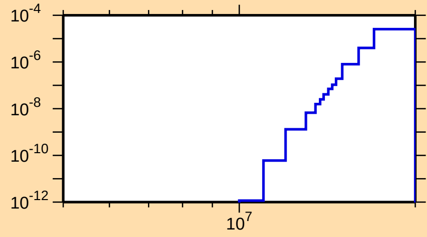
\sigma vs. E for ^{128}\text{Nd}(\text{mt } 45)
