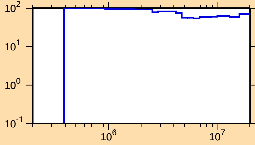
\Delta\sigma/\sigma vs. E for ^{128}\text{Nd}(n,n\text{cont.})
