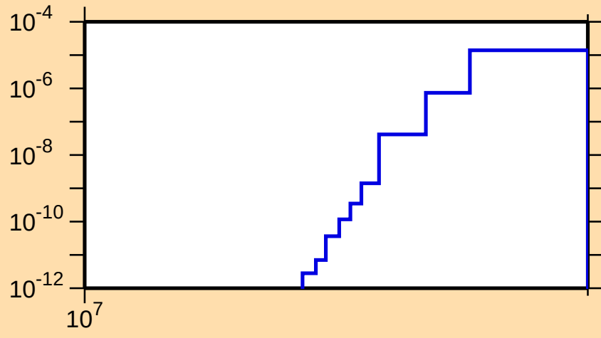
\sigma vs. E for ^{128}\text{Nd}(n,\text{pt})
