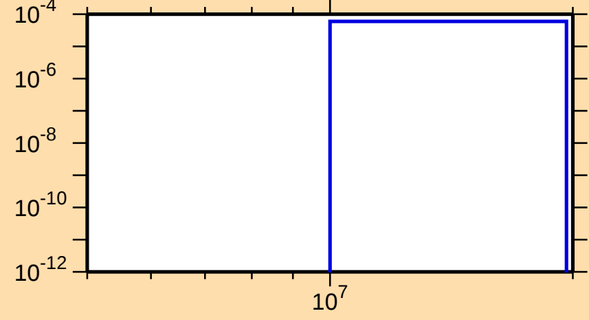
\sigma vs. E for ^{128}\text{Nd}(n,t)
