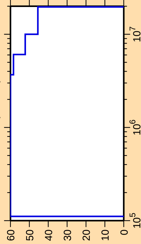
\Delta\sigma/\sigma vs. E for ^{128}\text{Nd}(\text{n,inel.})
