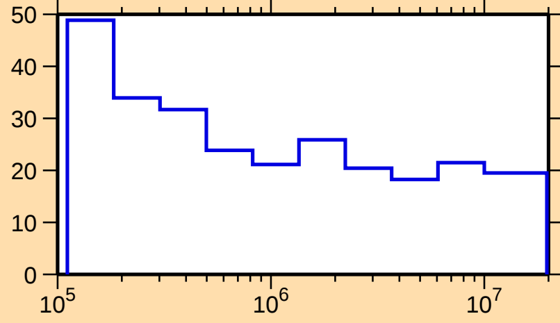
\Delta\sigma/\sigma vs. E for ^{128}\text{Nd}(\text{n,nonel.})
