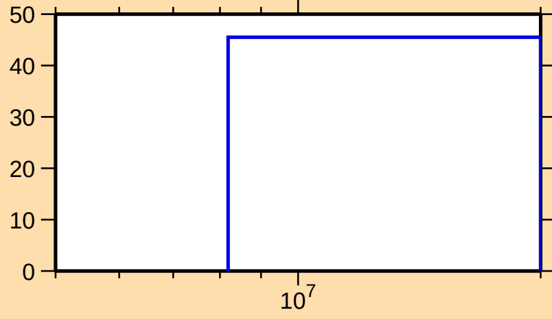
\Delta\sigma/\sigma vs. E for ^{128}\text{Nd}(n,\text{inel.})
