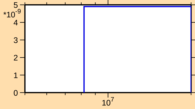
\sigma vs. E for ^{128}\text{Nd}(n,2np)
