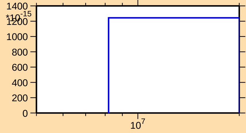
\sigma vs. E for ^{128}\text{Nd}(n,2n\alpha)
