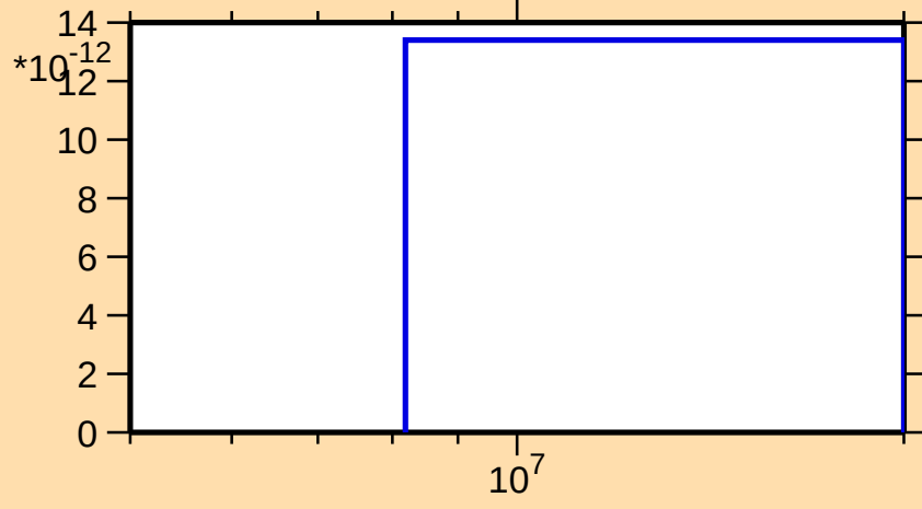
\sigma vs. E for ^{128}\text{Nd}(\text{mt } 34)
