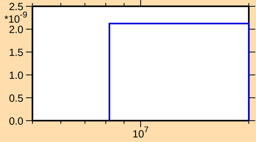
\sigma vs. E for ^{128}\text{Nd}(\text{mt117})
