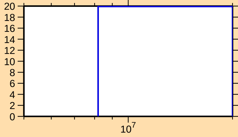
\Delta\sigma/\sigma vs. E for ^{128}\text{Nd}(n,\text{nonel.})
