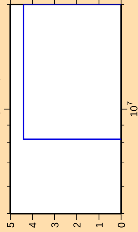
\Delta\sigma/\sigma vs. E for ^{128}\text{Nd}(n,2n\alpha)
