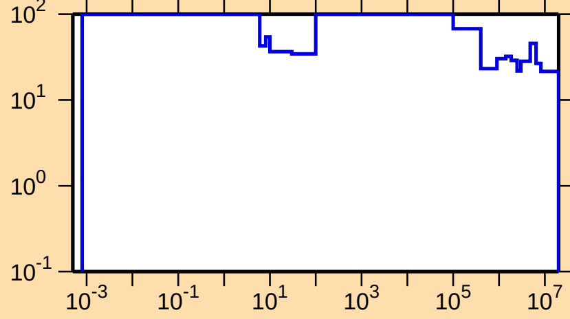
\Delta\sigma/\sigma vs. E for ^{128}\text{Nd}(n,\text{el.})
