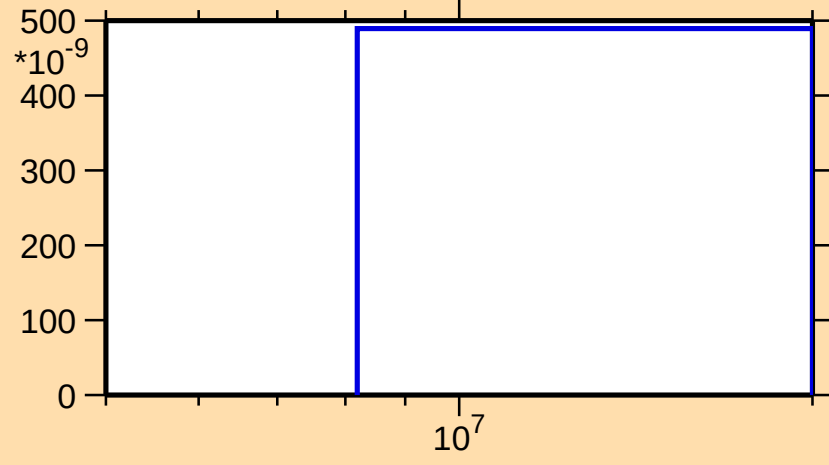
\sigma vs. E for ^{128}\text{Nd}(\text{mt } 45)
