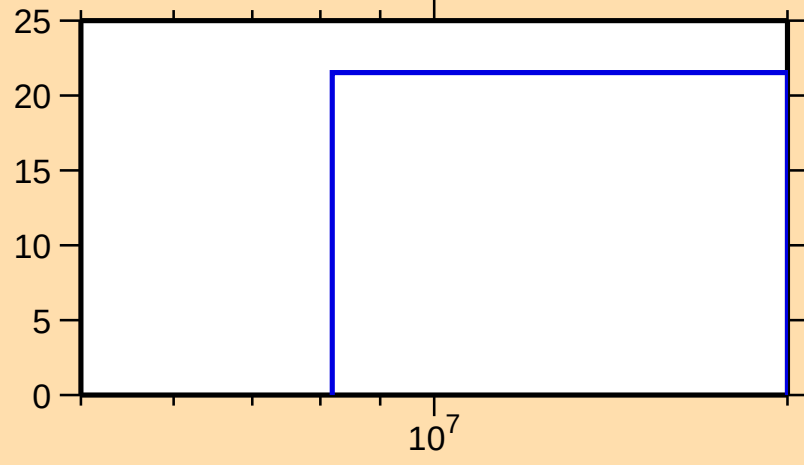
\Delta\sigma/\sigma vs. E for ^{128}\text{Nd}(n,\text{el.})
