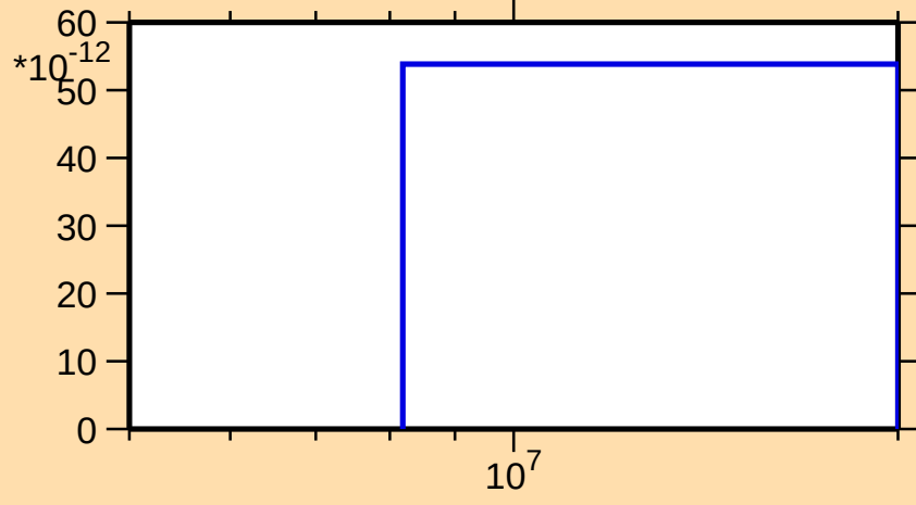
\sigma vs. E for ^{128}\text{Nd}(n,\text{nd})
