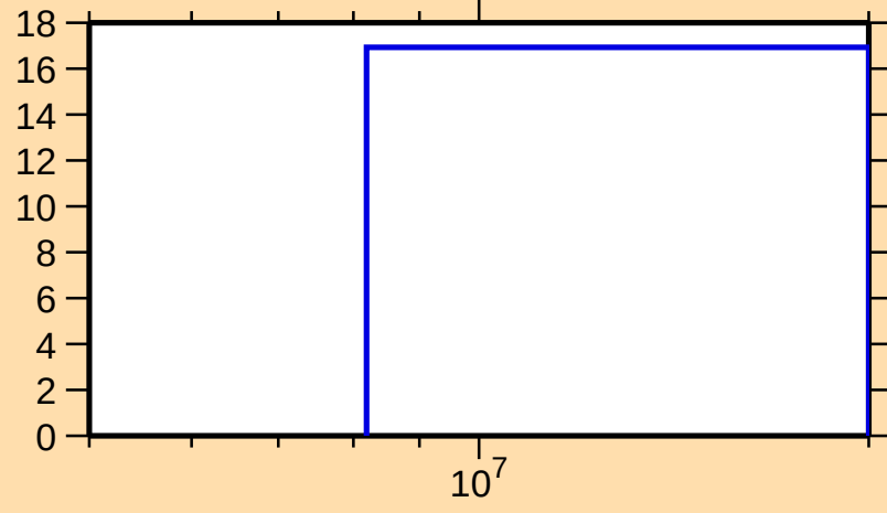
\Delta\sigma/\sigma vs. E for ^{128}\text{Nd}(n,\text{tot.})
