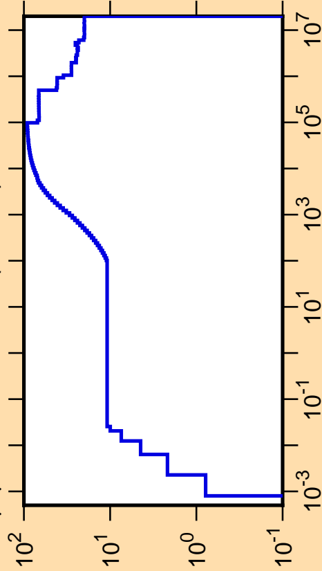
\Delta\mu/\mu vs. E for ^{129}\text{Nd}(\text{mt251})
