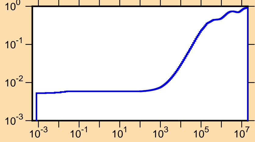
\mu vs. E for ^{129}\text{Nd}(\text{mt251})
