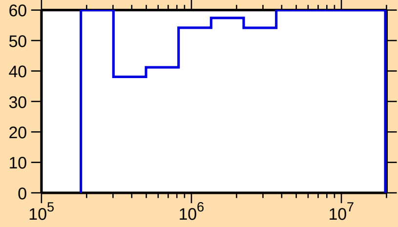
\Delta\sigma/\sigma vs. E for ^{129}\text{Nd}(n,n_1)
