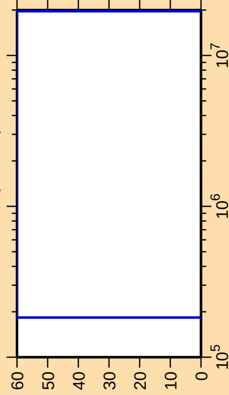
\Delta\sigma/\sigma vs. E for ^{129}\text{Nd}(n,\text{inel.})
