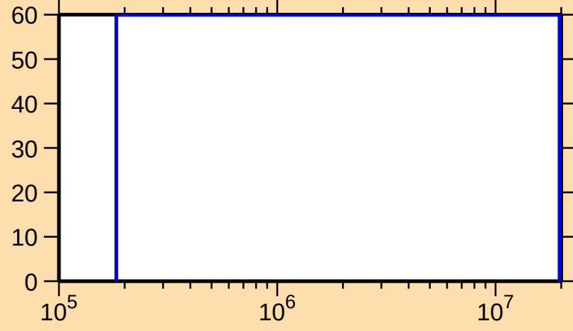
\Delta\sigma/\sigma vs. E for ^{129}\text{Nd}(n,n\text{cont.})
