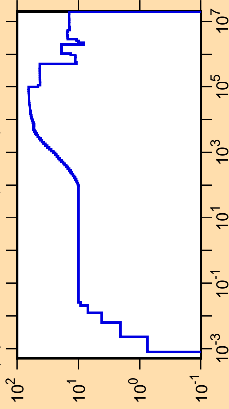
\Delta\mu/\mu vs. E for ^{131}\text{Nd}(\text{mt251})
