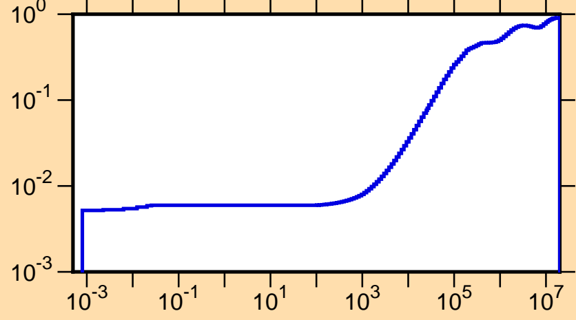
\mu vs. E for ^{131}\text{Nd}(\text{mt251})
