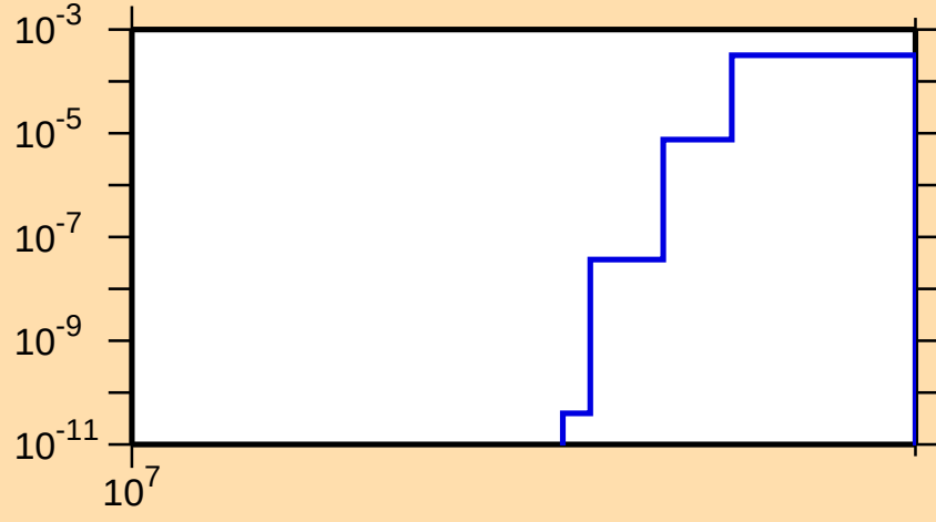
\sigma vs. E for ^{131}\text{Nd}(n,2np)
