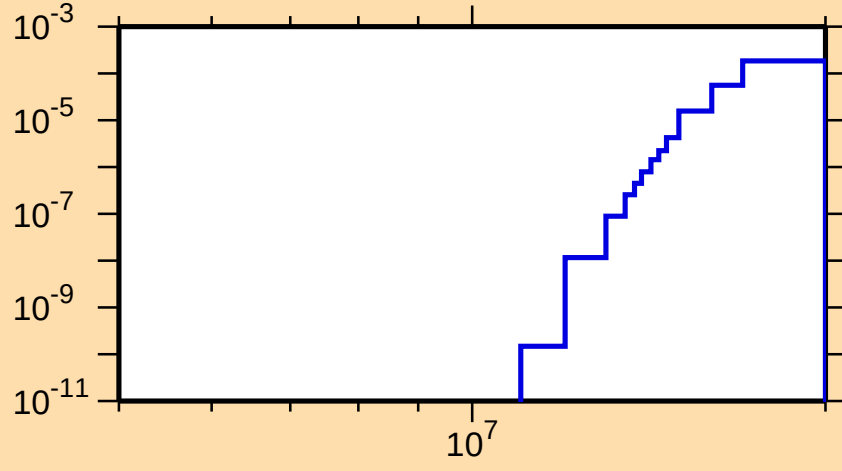
\sigma vs. E for ^{131}\text{Nd}(n,\text{pt})
