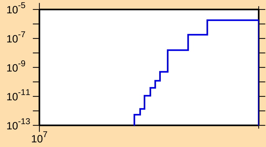
\sigma vs. E for ^{131}\text{Nd}(n,\text{nd})
