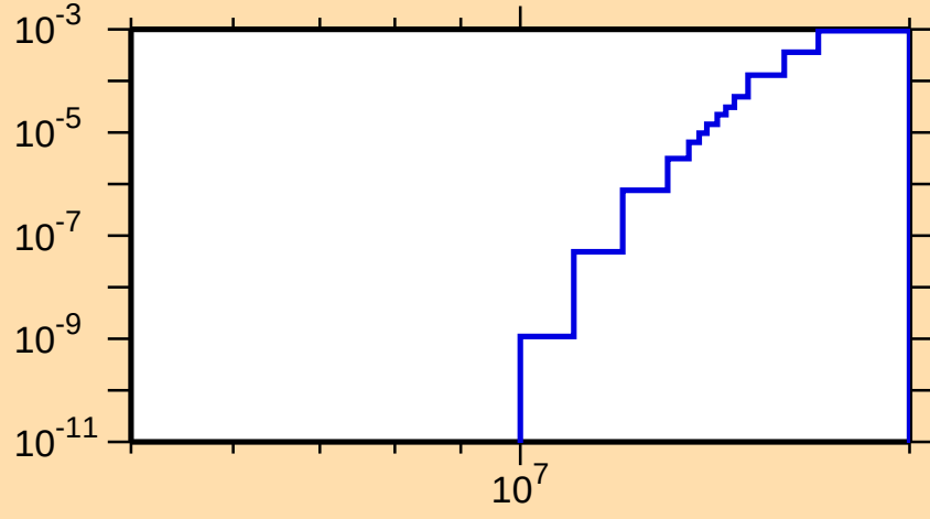
\sigma vs. E for ^{131}\text{Nd}(n,\text{pd})
