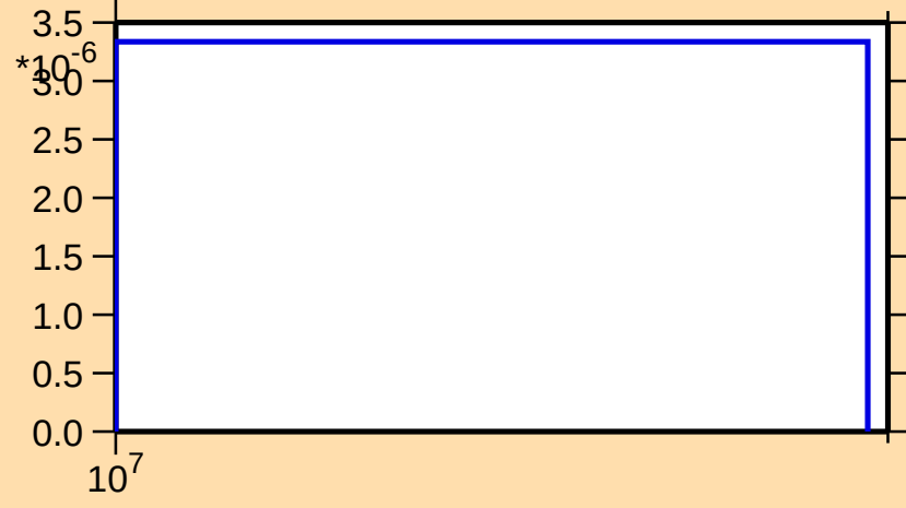
\sigma vs. E for ^{131}\text{Nd}(n,2np)
