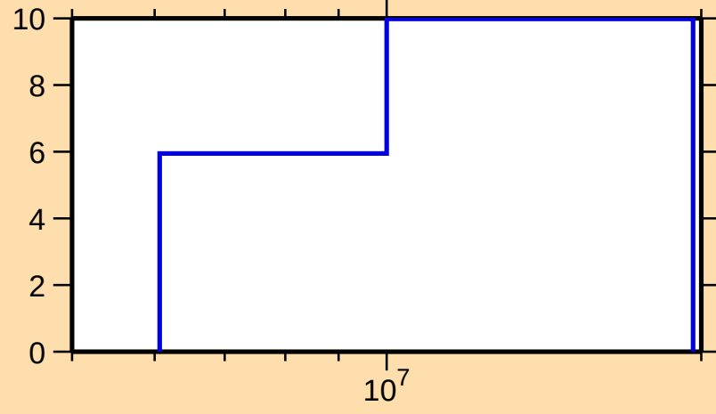
\Delta\sigma/\sigma vs. E for ^{131}\text{Nd}(n,\text{tot.})
