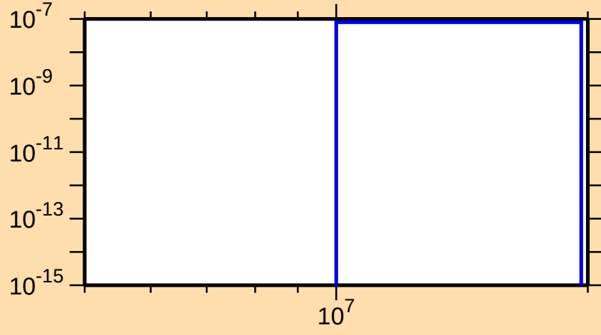
\sigma vs. E for ^{131}\text{Nd}(\text{mt } 45)
