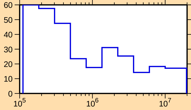
\Delta\sigma/\sigma vs. E for ^{131}\text{Nd}(n,\text{el.})
