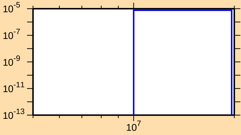
\sigma vs. E for ^{131}\text{Nd}(n,\text{pt})
