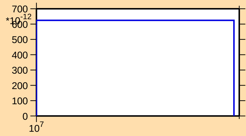
\sigma vs. E for ^{131}\text{Nd}(\text{mt117})
