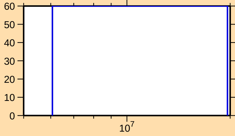
\Delta\sigma/\sigma vs. E for ^{131}\text{Nd}(n,\text{inel.})
