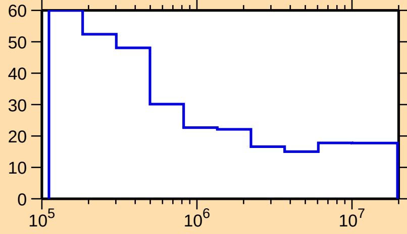
\Delta\sigma/\sigma vs. E for ^{131}\text{Nd}(n,\text{nonel.})
