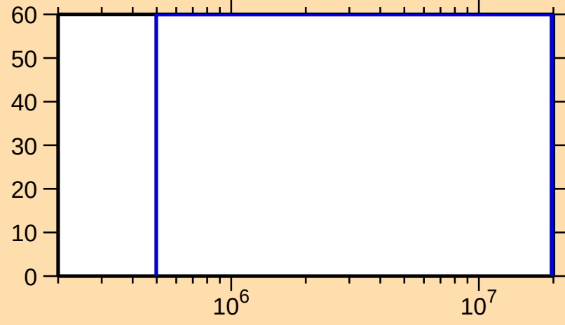
\Delta\sigma/\sigma vs. E for ^{131}\text{Nd}(n,n\text{cont.})
