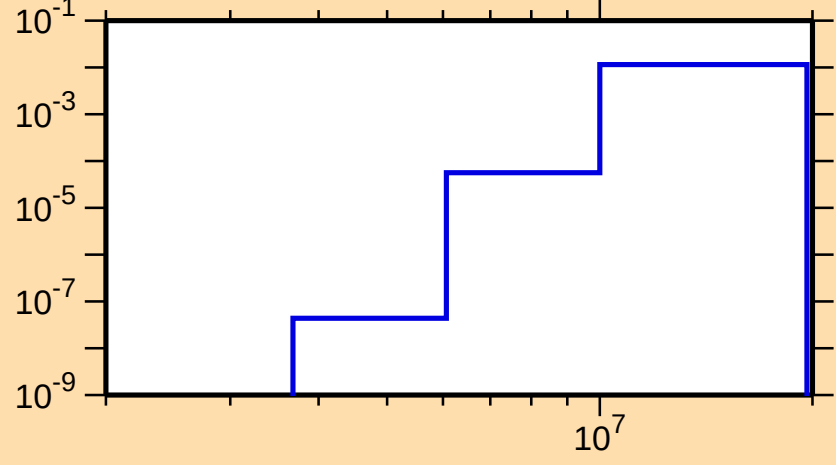
\sigma vs. E for ^{131}\text{Nd}(n,\alpha)
