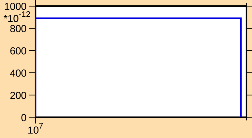
\sigma vs. E for ^{131}\text{Nd}(\text{mt } 34)
