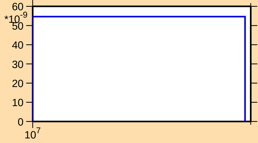
\sigma vs. E for ^{131}\text{Nd}(n,2n\alpha)
