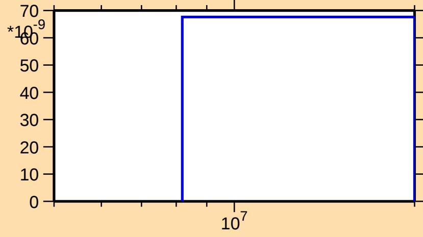
\sigma vs. E for ^{131}\text{Nd}(\text{mt } 45)
