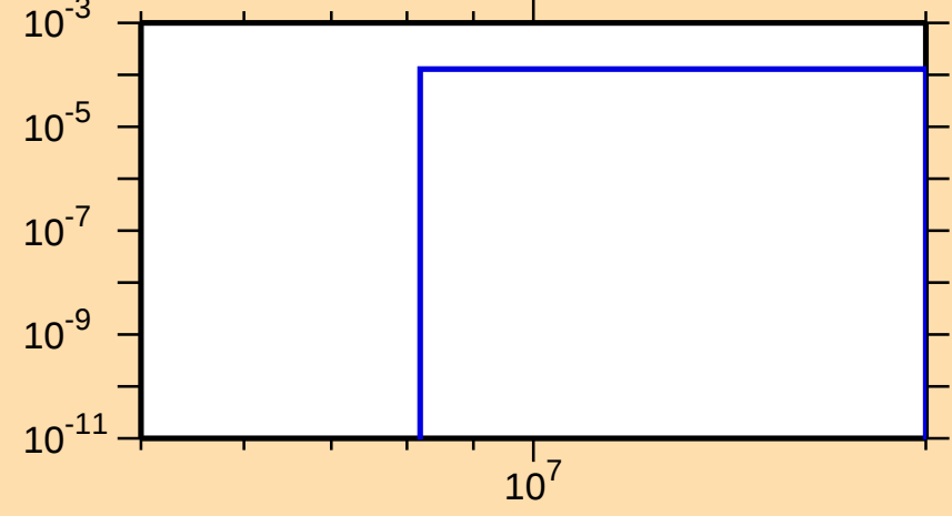
\sigma vs. E for ^{131}\text{Nd}(n,t)
