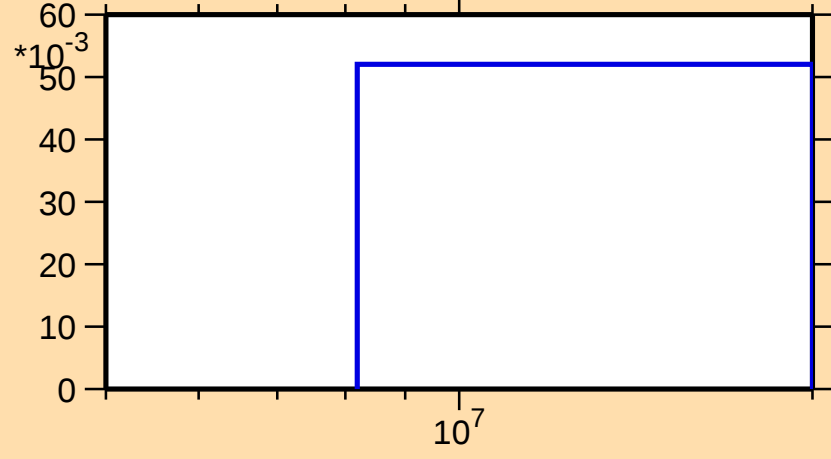
\sigma vs. E for ^{131}\text{Nd}(n,2n)
