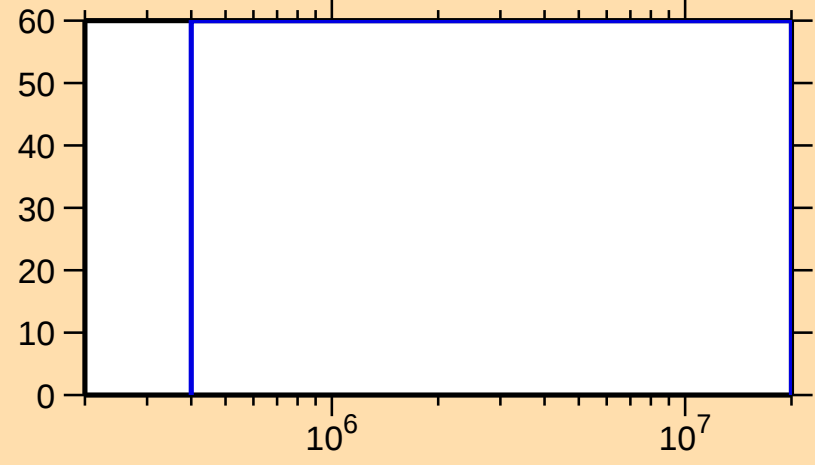
\Delta\sigma/\sigma vs. E for ^{131}\text{Nd}(n,ncont.)
