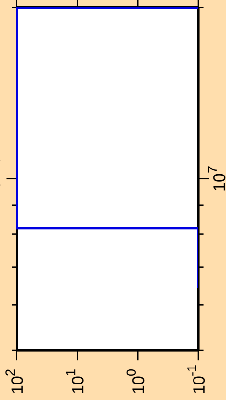
\Delta\sigma/\sigma vs. E for ^{131}\text{Nd}(n,t)
