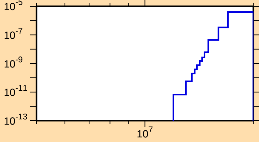
\sigma vs. E for ^{133}\text{Nd}(\text{mt } 45)
