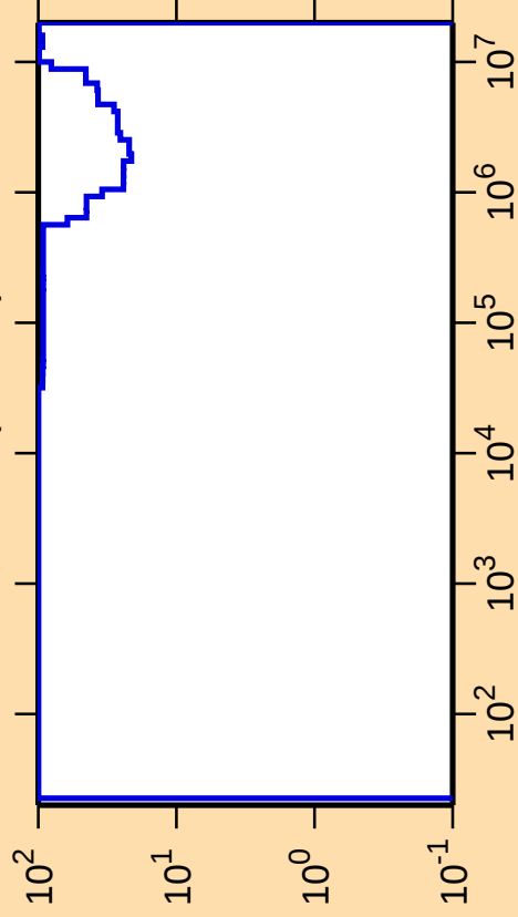
\Delta\sigma/\sigma vs. E for ^{133}\text{Nd}(n,\text{inel.})
