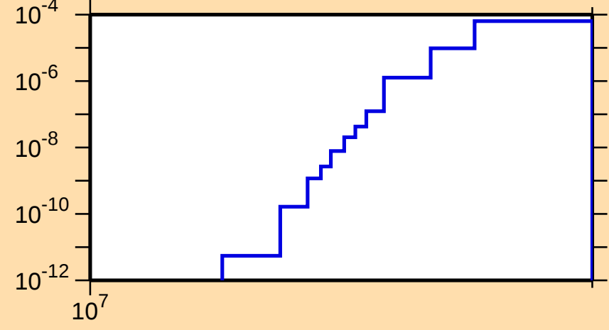
\sigma vs. E for ^{133}\text{Nd}(n,2n\alpha)
