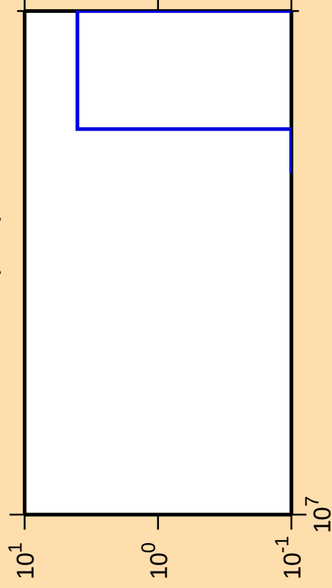
\Delta\sigma/\sigma vs. E for ^{133}\text{Nd}(n,\text{nt})
