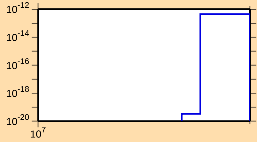
\sigma vs. E for ^{133}\text{Nd}(n,\text{nt})
