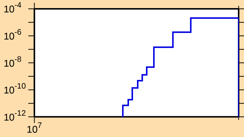
\sigma vs. E for ^{133}\text{Nd}(n,\text{nd})
