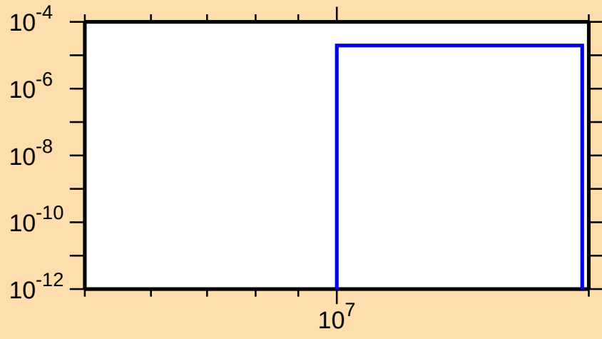
\sigma vs. E for ^{133}\text{Nd}(n,\text{pd})
