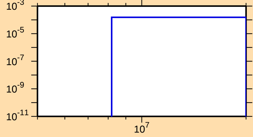
\sigma vs. E for ^{133}\text{Nd}(n,t)
