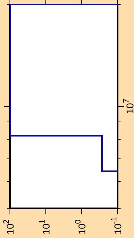
\Delta\sigma/\sigma vs. E for ^{133}\text{Nd}(n,t)
