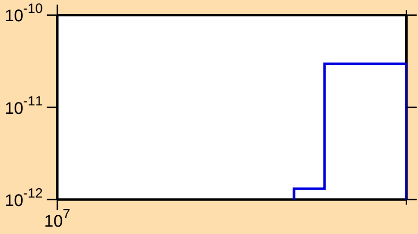
\sigma vs. E for ^{137}\text{Nd}(\text{mt117})
