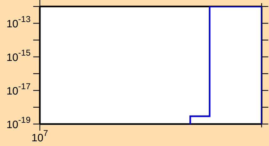
\sigma vs. E for ^{137}\text{Nd}(n,\text{nt})
