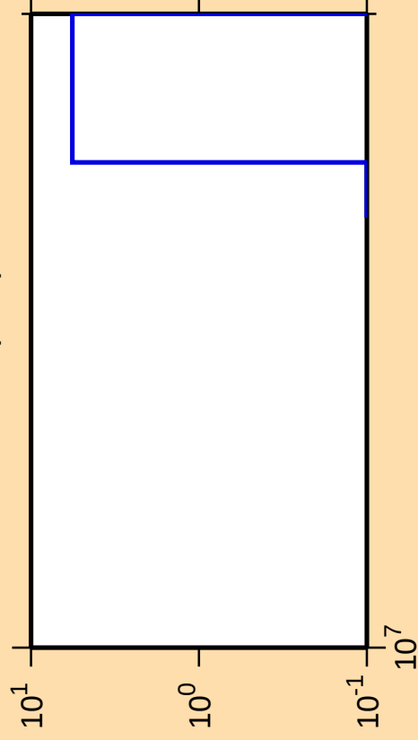
\Delta\sigma/\sigma vs. E for ^{137}\text{Nd}(n,\text{nt})
