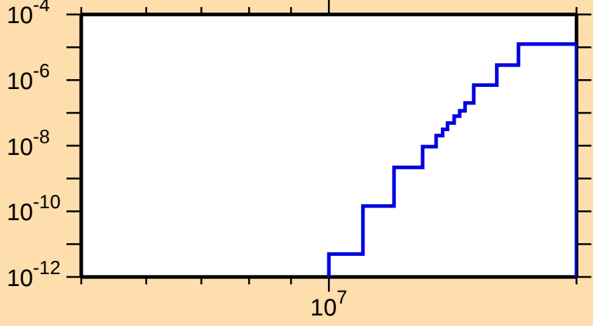
\sigma vs. E for ^{137}\text{Nd}(n,\text{He3})
