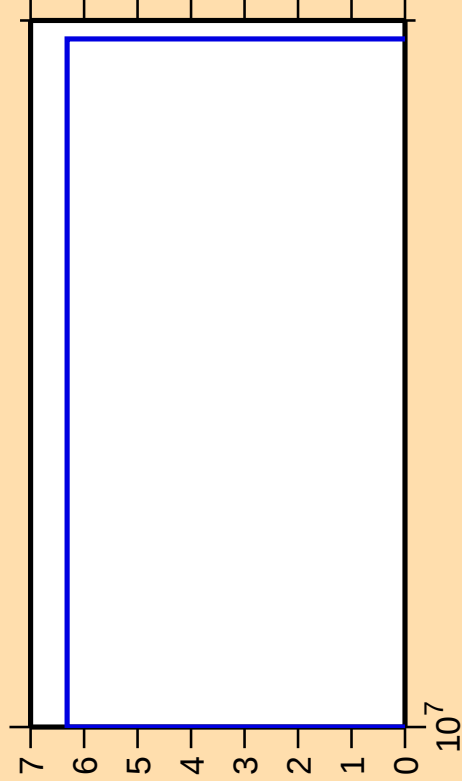
\Delta\sigma/\sigma vs. E for ^{137}\text{Nd}(\text{mt } 34)
