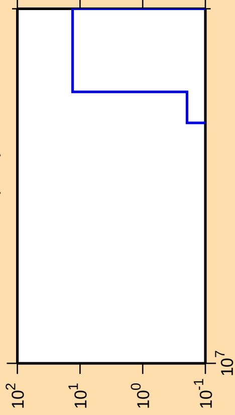
\Delta\sigma/\sigma vs. E for ^{138}\text{Nd}(n,\text{nt})
