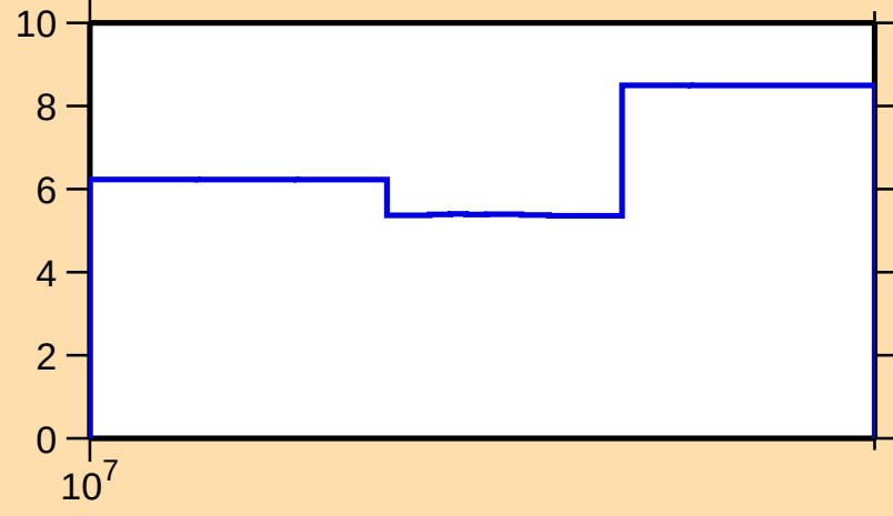
\Delta\sigma/\sigma vs. E for ^{138}\text{Nd}(n,\text{tot.})
