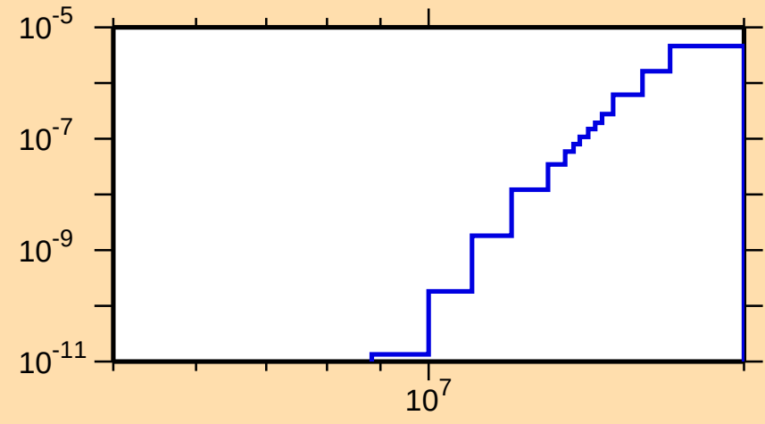
\sigma vs. E for ^{138}\text{Nd}(n,p\alpha)
