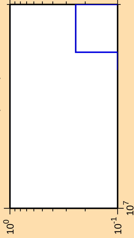
\Delta\sigma/\sigma vs. E for ^{138}\text{Nd}(\text{mt } 34)
