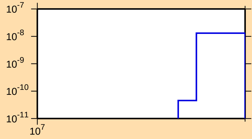
\sigma vs. E for ^{138}\text{Nd}(n,2n\alpha)
