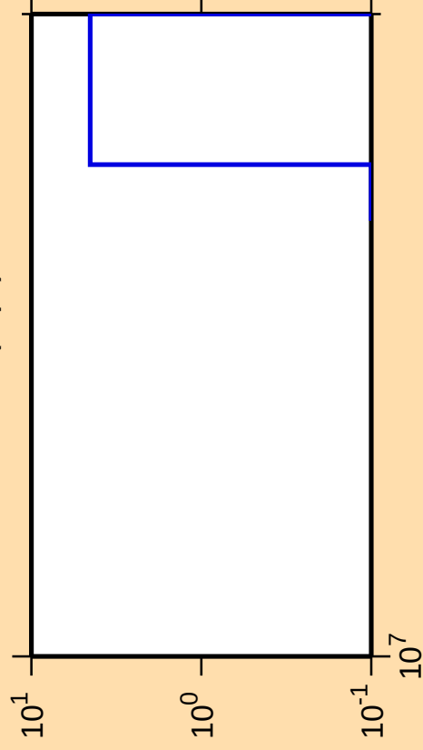
\Delta\sigma/\sigma vs. E for ^{138}\text{Nd}(n,\text{pt})
