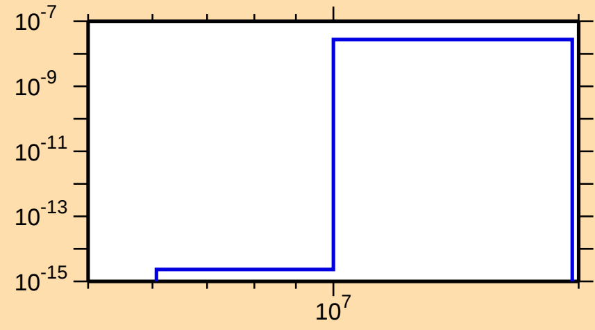
\sigma vs. E for ^{138}\text{Nd}(n,\text{He3})
