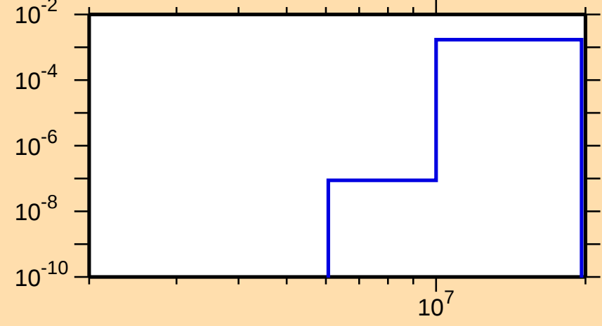
\sigma vs. E for ^{138}\text{Nd}(n,d)
