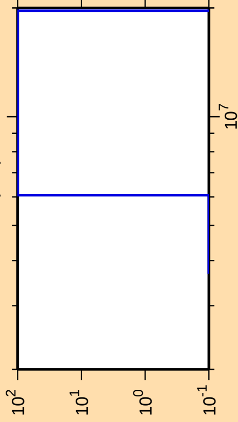
\Delta\sigma/\sigma vs. E for ^{138}\text{Nd}(n,d)
