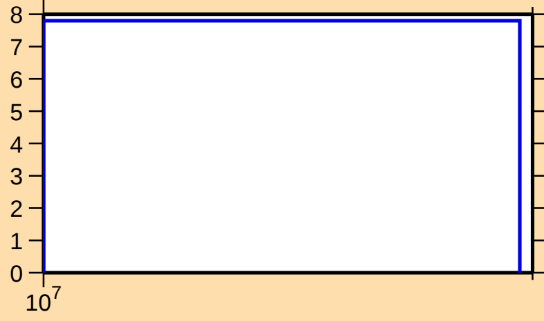
\Delta\sigma/\sigma vs. E for ^{138}\text{Nd}(n,\text{nonel.})
