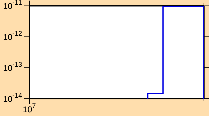
\sigma vs. E for ^{139}\text{Nd}(\text{mt } 34)
