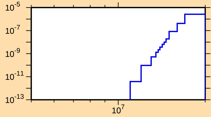
\sigma vs. E for ^{139}\text{Nd}(n,\text{He3})
