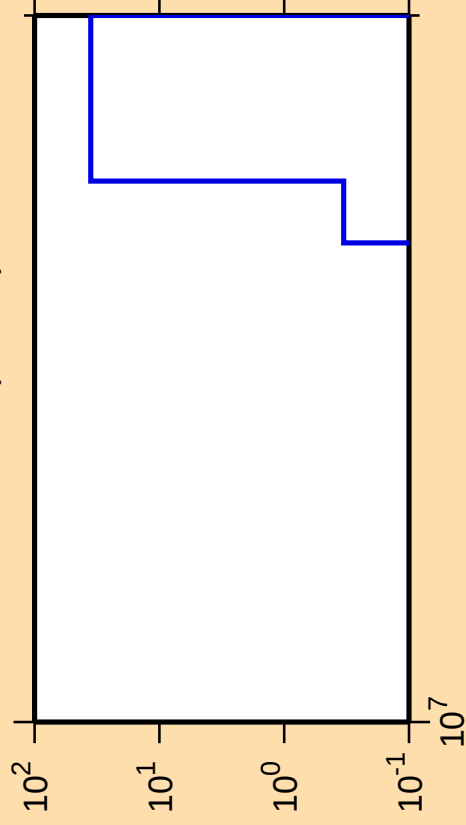
\Delta\sigma/\sigma vs. E for ^{139}\text{Nd}(\text{mt } 45)
