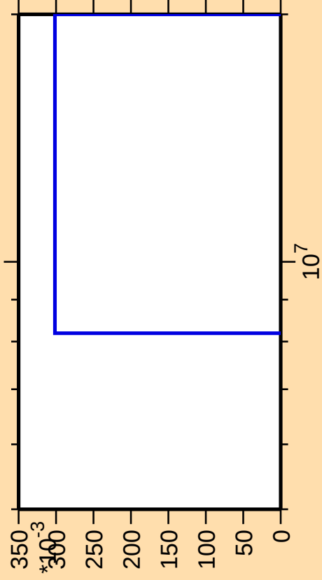
\Delta\sigma/\sigma vs. E for ^{139}\text{Nd}(\text{mt } 45)
