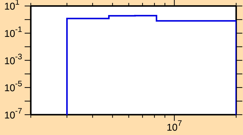
\sigma vs. E for ^{139}\text{Nd}(n,n\text{cont.})
