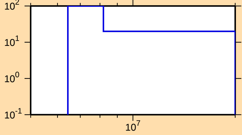
\Delta\sigma/\sigma vs. E for ^{139}\text{Nd}(n,2n)
