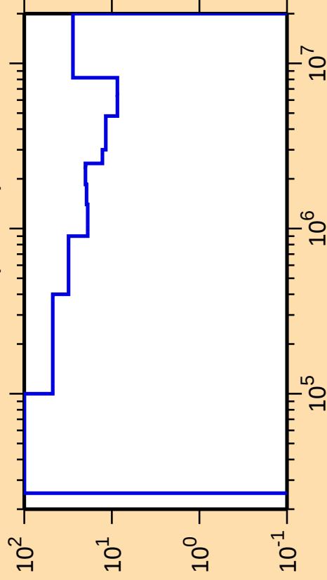
\Delta\sigma/\sigma vs. E for ^{139}\text{Nd}(n,\text{inel.})
