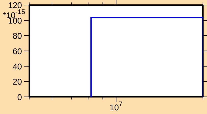
\sigma vs. E for ^{139}\text{Nd}(n,\text{nt})
