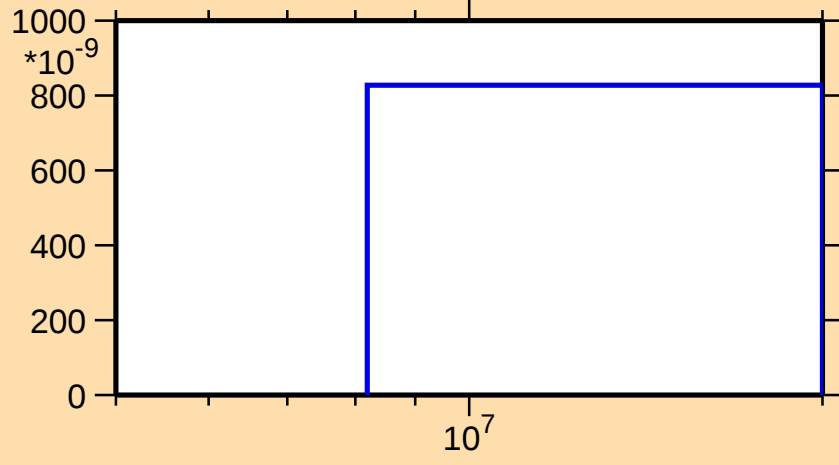
\sigma vs. E for ^{139}\text{Nd}(n,3n)
