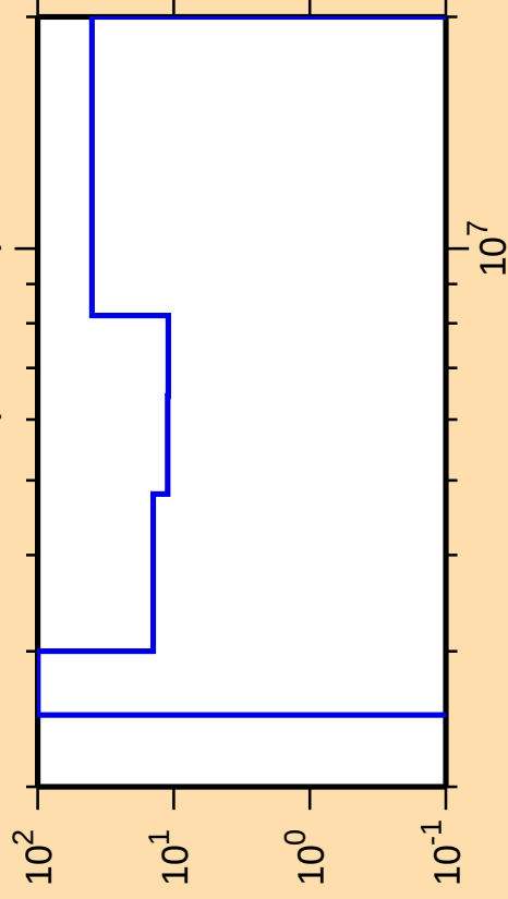
\Delta\sigma/\sigma vs. E for ^{139}\text{Nd}(n,\text{ncont.})
