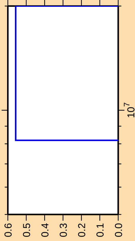
\Delta\sigma/\sigma vs. E for ^{139}\text{Nd}(\text{mt } 34)
