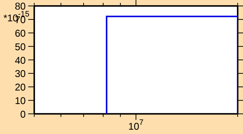
\sigma vs. E for ^{139}\text{Nd}(\text{mt } 45)
