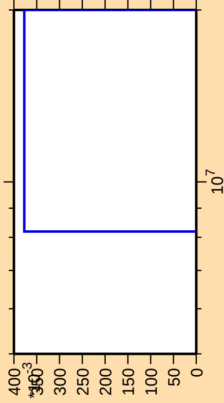
\Delta\sigma/\sigma vs. E for ^{139}\text{Nd}(n,\text{nt})
