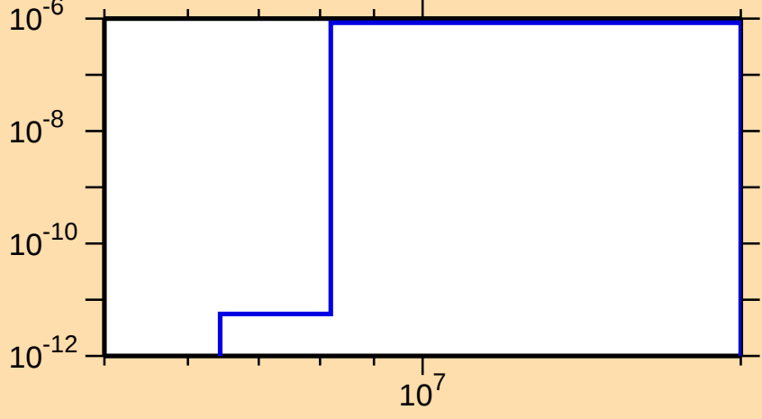
\sigma vs. E for ^{139}\text{Nd}(n,p\alpha)
