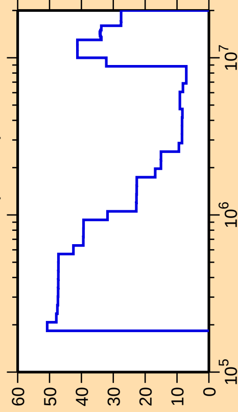
\Delta\sigma/\sigma vs. E for ^{141}\text{Nd}(n,\text{inel.})
