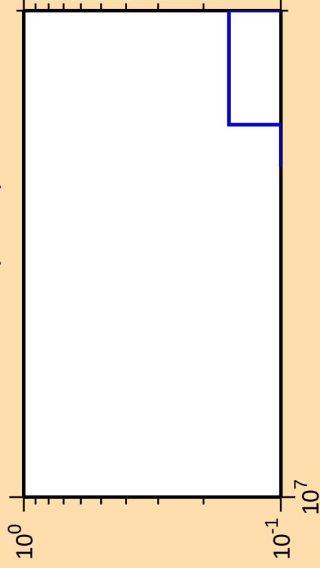
\Delta\sigma/\sigma vs. E for ^{141}\text{Nd}(\text{mt } 45)
