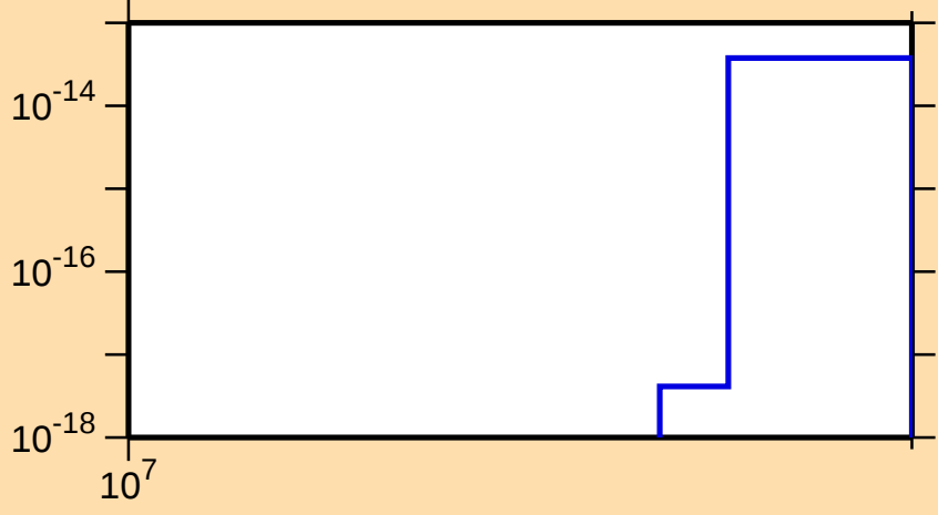
\sigma vs. E for ^{141}\text{Nd}(\text{mt } 45)
