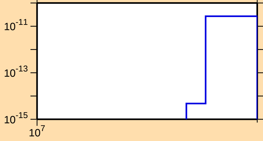
\sigma vs. E for ^{141}\text{Nd}(n,\text{pt})
