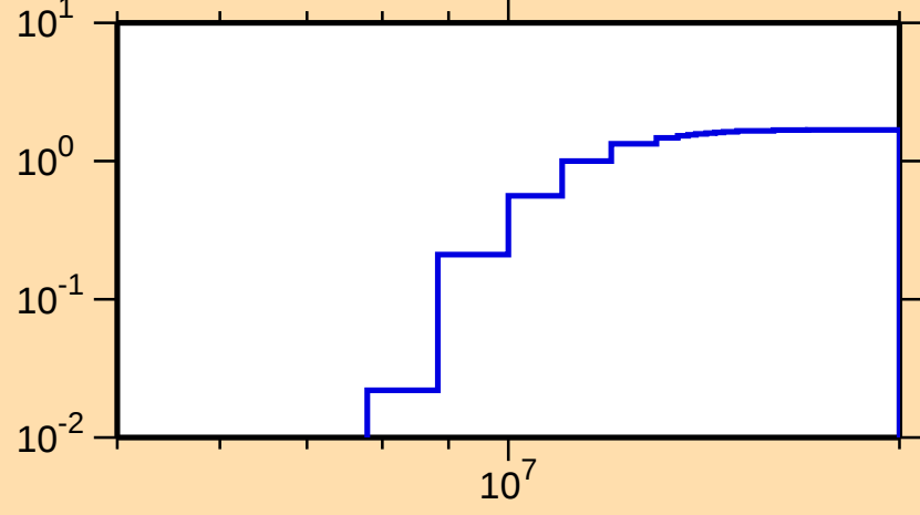
\sigma vs. E for ^{141}\text{Nd}(n,2n)
