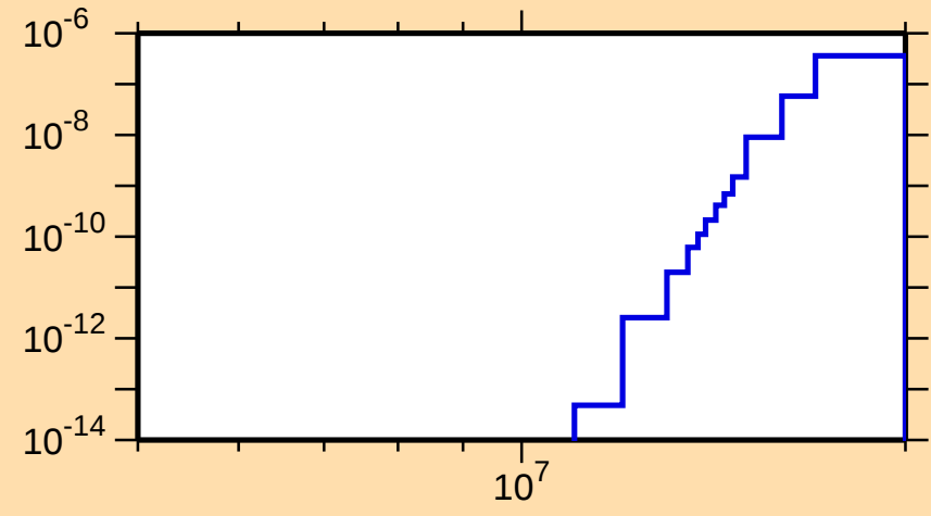
\sigma vs. E for ^{141}\text{Nd}(n,\text{He3})
