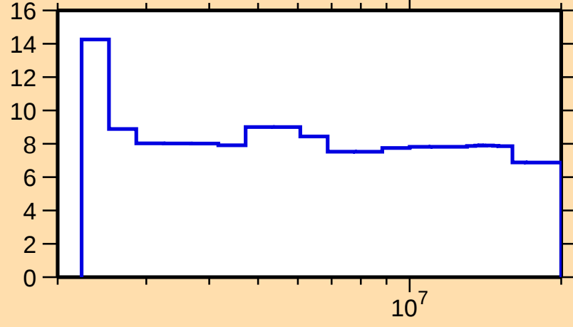
\Delta\sigma/\sigma vs. E for ^{141}\text{Nd}(n,n\text{onel.})
