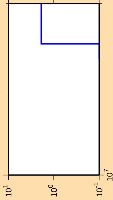
\Delta\sigma/\sigma vs. E for ^{141}\text{Nd}(\text{mt } 34)
