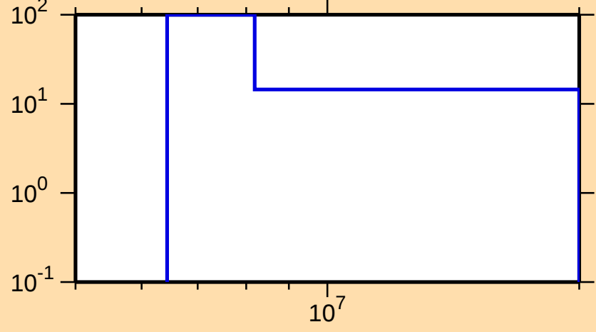
\Delta\sigma/\sigma vs. E for ^{141}\text{Nd}(n,2n)
