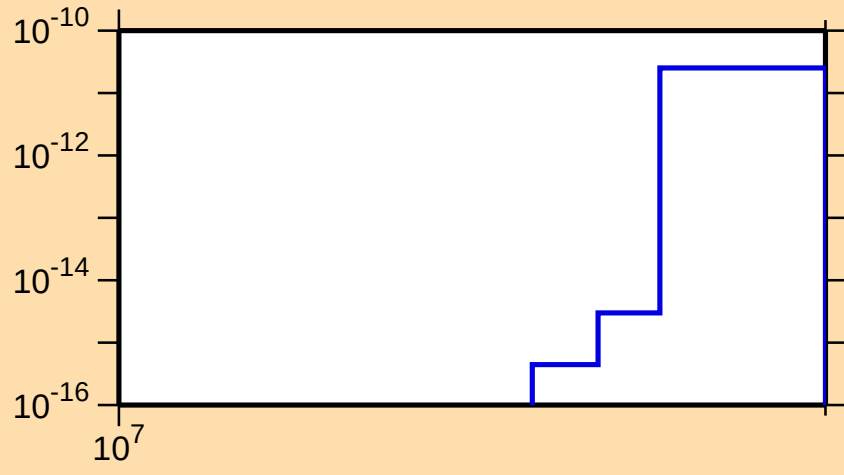
\sigma vs. E for ^{141}\text{Nd}(n,\text{nt})
