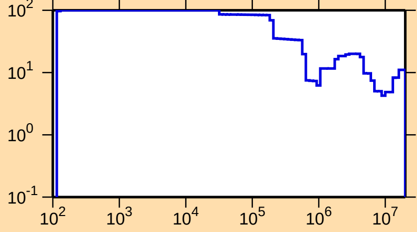
\Delta\sigma/\sigma vs. E for ^{141}\text{Nd}(n,\text{el.})
