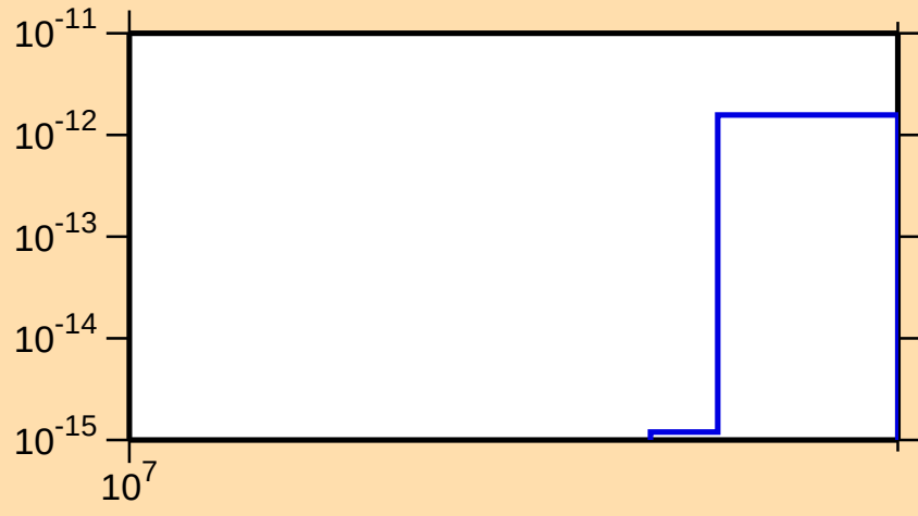
\sigma vs. E for ^{141}\text{Nd}(\text{mt } 34)
