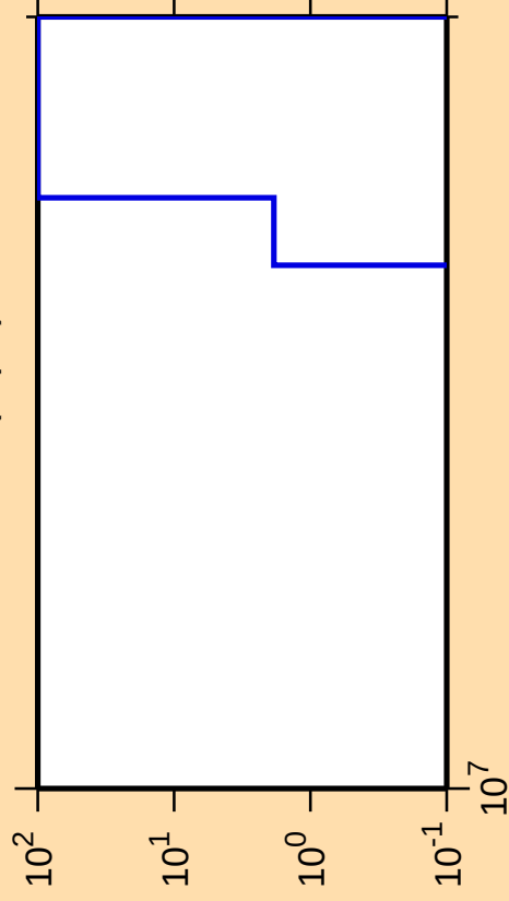
\Delta\sigma/\sigma vs. E for ^{142}\text{Nd}(n,\text{pd})
