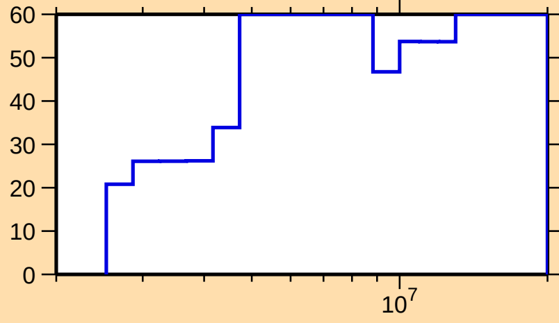
\Delta\sigma/\sigma vs. E for ^{142}\text{Nd}(n,\gamma)
