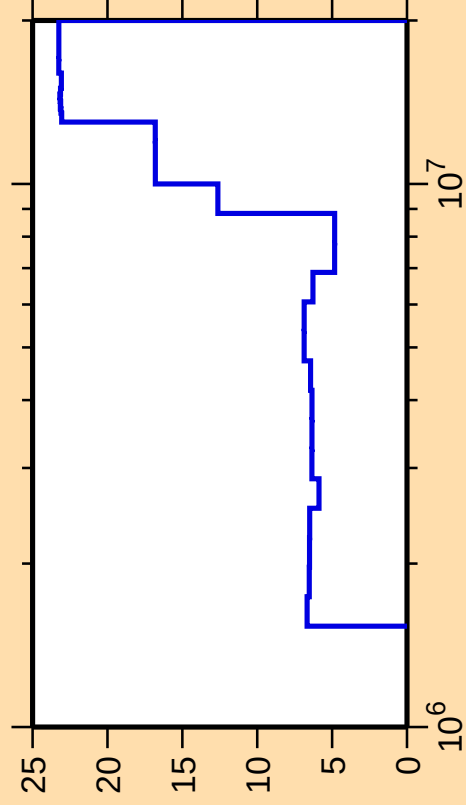
\Delta\sigma/\sigma vs. E for ^{142}\text{Nd}(\text{n,inel.})
