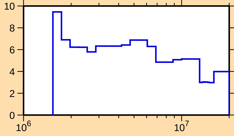
\Delta\sigma/\sigma vs. E for ^{142}\text{Nd}(\text{n,nonel.})
