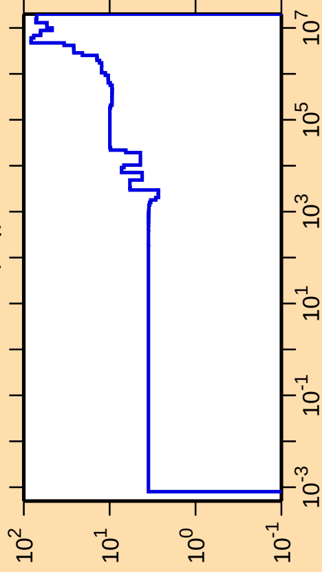
\Delta\sigma/\sigma vs. E for ^{142}\text{Nd}(n,\gamma)
