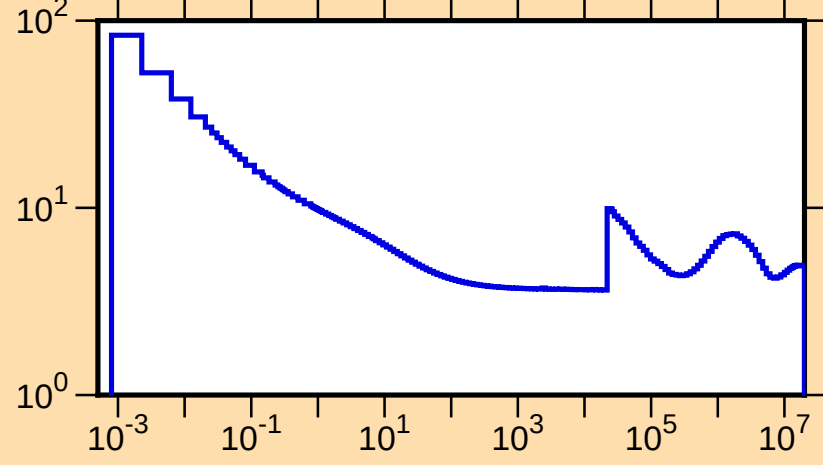
\sigma vs. E for ^{142}\text{Nd}(n,\text{tot.})
