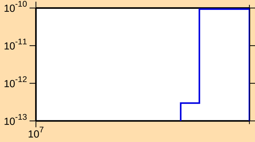
\sigma vs. E for ^{142}\text{Nd}(n,\text{pd})
